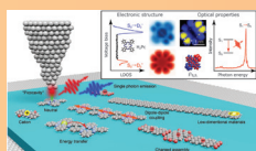
Tip-induced fluorescence of individual molecules: probing light-matter interaction at the subnanometer scale. [Rosławska et al , Rev. Mod. Phys. 98 , 025007 (2026)]
