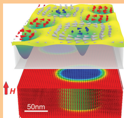
Ginzburg-Landau simulation of the superfluid and supercurrent densities above an experimentally observed skyrmion in a magnet-superconductor heterostructure. [Alexander P. Petrović et al. , Rev. Mod. Phys. 97 , 031001 (2025)]
