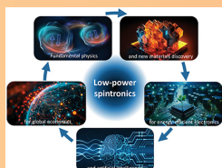
Energy efficient computing enabled by low-power spintronics. [Albert Fert et al. , Rev. Mod. Phys. 96 , 015005 (2024)]
