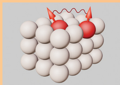
The exchange interaction between two atomic magnetic moments in a solid. [Attila Szilva et al. , Rev. Mod. Phys. 95 , 035004 (2023)]
