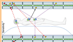
Total-body PET design for the positronium and quantum entanglement imaging [Steven D. Bass, Sebastiano Mariazzi, Pawel Moskal, and Ewa Stepień, Rev. Mod. Phys. 95 , 021002 (2023)]
