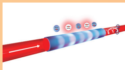
Photons interacting in a waveguide with quantum emitters [Alexandra S. Sheremet, Mihail I. Petrov, Ivan V. Iorsh, Alexander V. Poshakinskiy, and Alexander N. Poddubny, Rev. Mod. Phys. 95 , 015002 (2023)]
