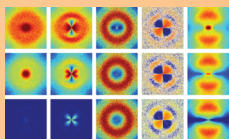
Decryption of magnetic small-angle neutron scattering cross sections using micromagnetic simulations. [Sebastian Mühlbauer et al. , Rev. Mod. Phys. 91 , 015004 (2019)]
