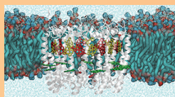
Example of natural light harvesting complex for photosynthesis. [Seogjoo J. Jang and Benedetta Mennucci, Reviews of Modern Physics 90 , 035003 (2018)]
