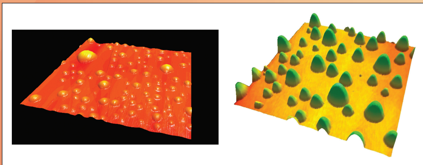
Surface nanobubbles and nanodroplets
