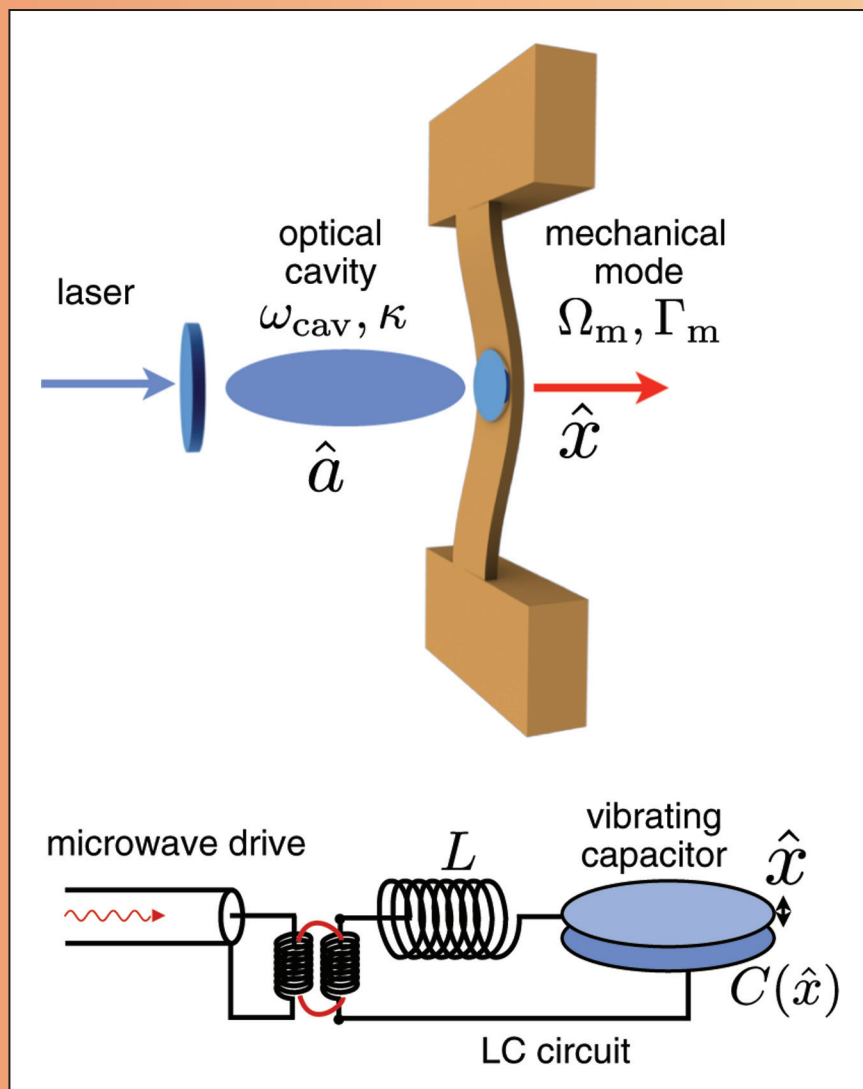
CAVITY OPTOMECHANICS
