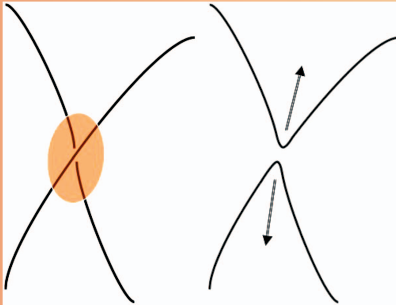
MAGNETIC RECONNECTION
