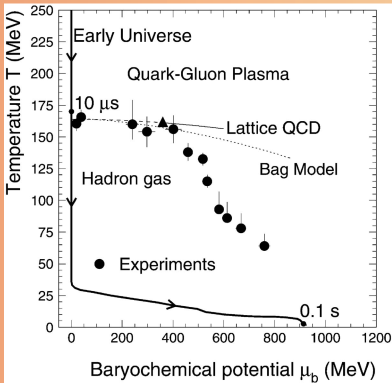
PHASE DIAGRAM OF STRONGLY INTERACTING MATTER
