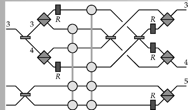
LINEAR OPTICAL QUANTUM COMPUTING WITH PHOTONIC QUBITS
