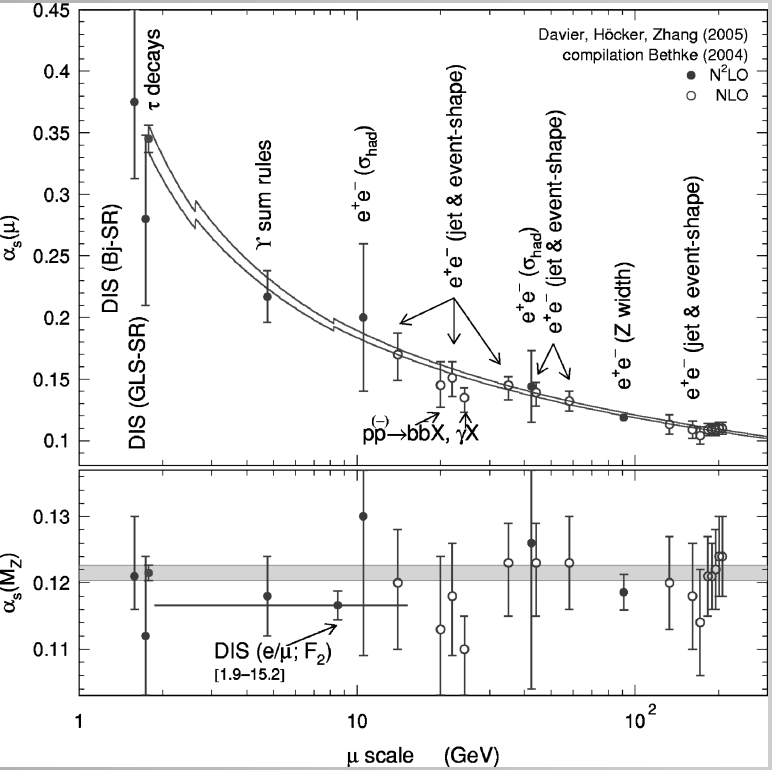
THE PHYSICS OF HADRONIC TAU DECAYS
