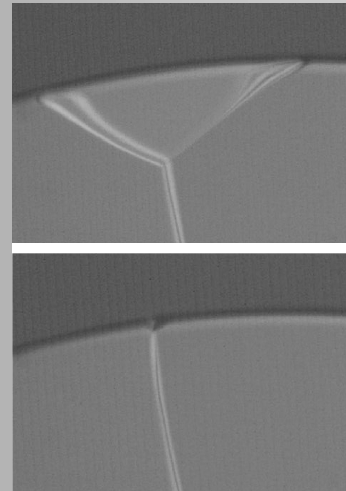
THE PHYSICS OF PREMELTED ICE AND ITS GEOPHYSICAL CONSEQUENCES
