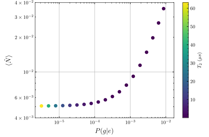
FIG. 9. Relationship between the leftover cavity population and the mixing error in the qubit. For each value of qubit decoherence, the measurement is simulated numerically, reaching a maximum near 100 photons, before being brought down by DRACHMA to around 0.01 photons. The x axis represents the probability of being in the excited qubit state when the system was initially in the ground. A very similar plot occurs with the states reversed. The y axis shows the cavity population immediately after the pulse finishes. The plots are calculated for 1000 ns with the same system parameters given in the main text.
