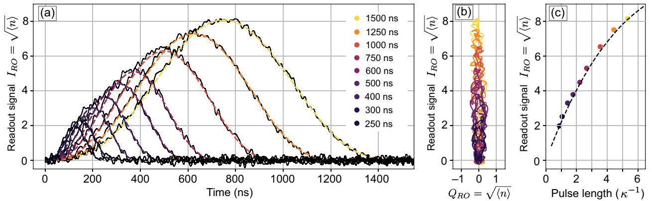
FIG. 4. (a) The measured in-phase readout signal I_{\text{RO}} = \text{Re}[Z_{\text{RO}}(t)] for the various durations of the DRACHMA pulse between 250 and 1500 ns. The magnitude of the input signal results in the same number of photons at the maximum of the intra-cavity field. (b) The evolution of the measured readout signal in the IQ plane. (c) The maximum of the readout signal as the function of the pulse duration. The dashed lines show the theoretical predictions from input-output theory.
