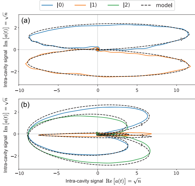
FIG. 3. Time evolution of the intracavity field in the IQ plane during qubit readout for (a) two-states readout and (b) three-states readout. The horizontal \text{Re}[a(t)] and vertical \text{Im}[a(t)] axes correspond to the in-phase and quadrature components of the intra-cavity field, both proportional to the square root of the intra-cavity photon number. The trajectories shown for the qubit in the ground ( |0\rangle , blue), 1st excited ( |1\rangle , orange) and 2nd excited ( |2\rangle , green) states follow distinct paths, while the dashed black lines represent the theoretical model. Both trajectories start and end at the origin, indicating that the optimized pulse shape leaves no residual photons in the resonator after measurement.
