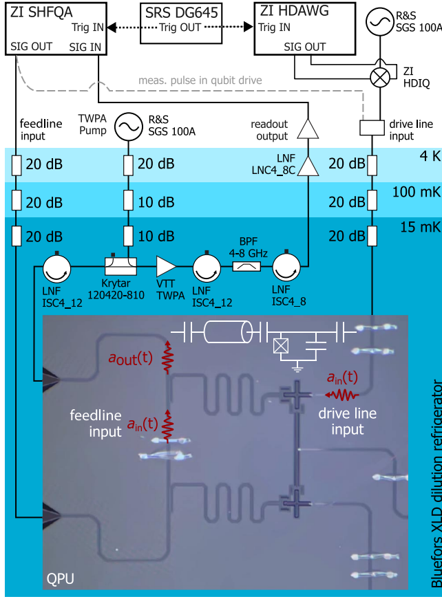
FIG. 7. Wiring diagram of the smooth readout experiment specifying the electronics and components. The readout input pulse a_{in}(t) is synthesized with the quantum state analyzer (SHFQA) and is applied in two different possible configurations: through the feedline input or via the qubit drive. The readout signal a_{out}(t) is amplified and then processed by the SHFQA. The baseband qubit control pulses are generated by HDAWG and upconverted to a carrier frequency. Microscope image of a quantum processing unit (QPU) with two transmon qubits. Only the top qubit is used for the experiment. Simplified circuit diagram of the transmon qubit coupled to the resonator (white).
