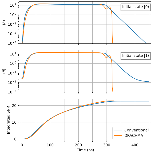
FIG. 10. Comparison of a conventional Gaussian-filtered rectangular measurement pulse and its DRACHMA version in case of a long ( 20/\kappa ) readout of a fast cavity. Both pulses achieve the same SNR in the same time and with the same maximum cavity occupation, but DRACHMA also depletes the cavity at the end of the pulse.
