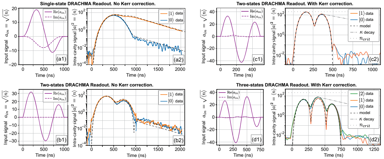
FIG. 2. DRACHMA input fields a_{\text{in}}(t) and the dynamics of intra-cavity fields \langle n(t) \rangle \propto |a(t)|^2 . (a) Readout with cavity reset for a single state. (b) Readout with cavity reset for the ground and first excited states of the transmon. (c),(d) DRACHMA readout when Kerr-nonlinearity corrections are taken into account. (c) Readout with > 35 dB cavity reset for the ground and first excited states of the transmon with T_p = 500 ns. (d) Readout with > 30 dB cavity reset for the ground, excited and second excited (qutrit) states with T_p = 750 ns. Solid lines are experimental data, and black dashed lines represent fits to the theory. The dash-dotted line ( \kappa decay) shows the conventional exponential decay of the readout cavity from the top of the pulse with decay constant \kappa^{-1} . The gray dotted line indicates the field magnitude corresponding to the critical photon number n_{\text{crit}} .
