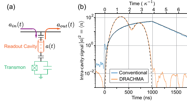
FIG. 1. (a) Simplified circuit diagram for the demonstration of dispersive readout of a superconducting qubit. (b) Demonstration of the concept of readout with cavity reset. Blue: the rectangular input readout pulse of duration T_p = 1 \mu\text{s} causes a long exponential decay of the intra-cavity field |a(t)|^2 . The solid line represents a fit of experimental data to a classic response theory, see Eq. (1). Orange: the DRACHMA readout with the Kerr-corrected pulse of the same length T_p = 1 \mu\text{s} quickly drives the cavity and returns it to the initial state. The dashed line represents a fit of experimental data to theory, see Eqs. (9) and (10).
