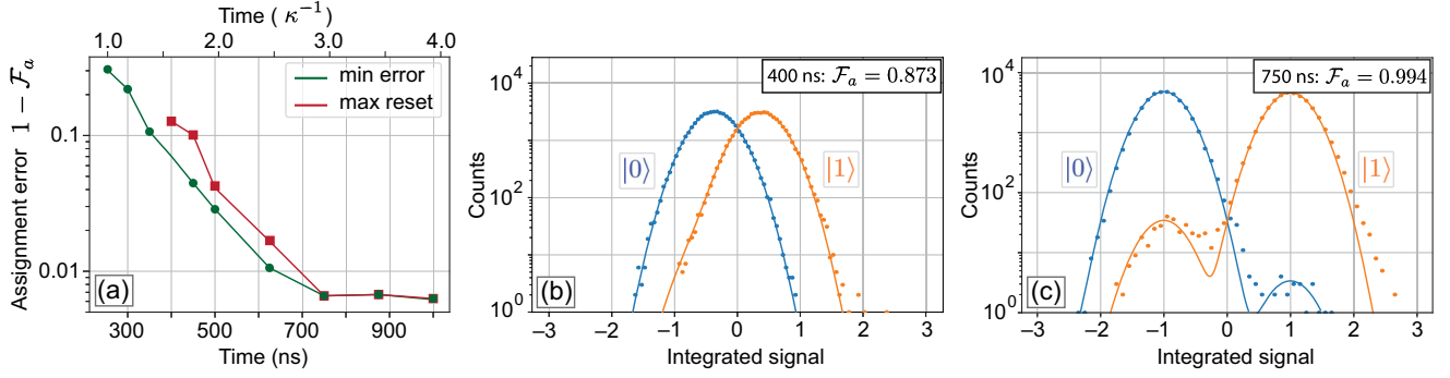
FIG. 5. (a) Best achieved state assignment error 1 - \mathcal{F}_a as a function of the DRACHMA pulse length for two cases: any pulse amplitude (green circles), amplitudes where > 35 dB reset contrast is maintained (red squares). (b),(c) Experimentally measured histograms of the integrated readout quadrature signal for measurement pulse lengths of T_p = 400 ns and T_p = 750 ns and > 35 dB reset contrast. The use of a longer pulse results in better state distinguishability.
