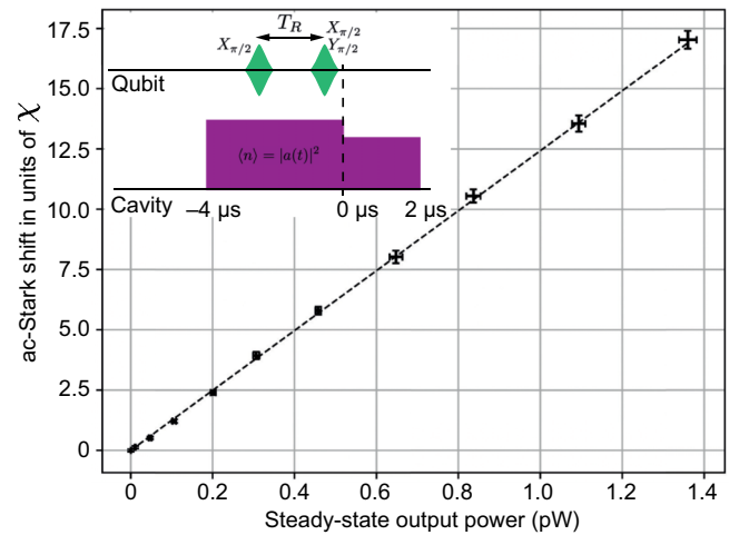
FIG. 8. Calibration of the intra-cavity photon number \langle n(t) \rangle = |a(t)|^2 by measuring the ac-Stark shift in a Ramsey experiment versus steady-state output power. Inset: the experimental pulse sequence. A long 4 \mu\text{s} cavity pulse builds up the steady-state population with variable magnitude, which overlaps with a Ramsey sequence at the end of the pulse. The qubit state is measured with a rectangular pulse of 2 \mu\text{s} duration.
