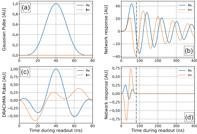
FIG. 6. Relationship between the Purcell network mode population and the input readout pulse. In (a) and (b) a standard Gaussian measurement pulse is simulated, while in (c) and (d) the DRACHMA pulse (15) is used. In the left column the pulses are plotted for an 80 ns readout, while in the right column the time-domain response is, respectively, shown. The dashed line indicates the end of the readout pulse. Without correction, the network mode requires a much longer time to empty than expected from the bare cavity linewidth. Non-linearity is not included in the simulation but would not be visible on the linear grid plot. Parameters are G/2\pi = 20 MHz, \kappa/2\pi = 14 MHz, \delta/2\pi = 50 MHz, \chi/2\pi = 6 MHz, taken from Refs. [26,27].
