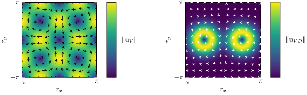
FIG. 4. Velocity field for the investigated initial states. Velocity field \mathbf{u}^*(\mathbf{r}^*, 0) (arrows) and its magnitude \|\mathbf{u}^*(\mathbf{r}^*, 0)\| (color map) for the Taylor-Green vortex (left) and Gaussian vortex dipole (right) initial states for D = 2 .
