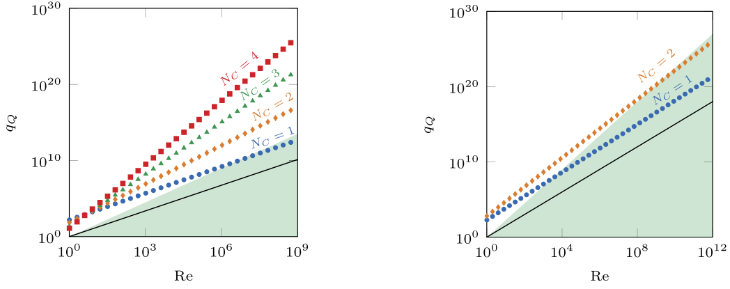
FIG. 9. Query complexity. The lower bound from Eq. (162) (black line) and upper bounds from Eq. (166) for different values of Carleman truncation order N_C (different symbols) of the query complexity q_Q of our quantum LBE algorithm resolving the Kolmogorov microscale and for systems with dimension D = 1 (left) and D = 2 (right). The green highlighted region indicates potential for quantum advantage, when q_Q is smaller than classical complexity. In the expressions of the form O(\text{Re}^x) for Complexity _C and the lower bound for q_Q , we assumed a constant 1 and plotted \text{Re}^x .
