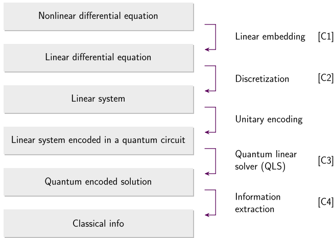
FIG. 1. Pipeline and challenges. The QLS-based algorithmic pipeline for Carleman-linearized dynamics commonly used in the literature, together with the challenges C1–C4 that we identify in Sec. IV.
