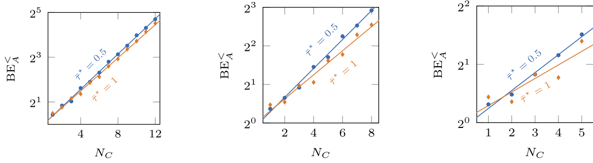
FIG. 6. Upper bounds for block-encoding prefactors. The numerical values of BE_A^< from Eq. (143) for different values of the Carleman truncation order N_C , relaxation parameter \bar{\tau}^* , and dimension D (left to right: D = 1 to D = 3 ), together with their best exponential fits as in Eq. (146). Note that the fits showcase slightly different slopes for the even and odd N_C , but we took an overall fit.
