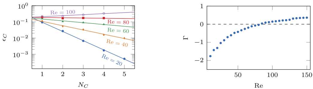
FIG. 3. Carleman error convergence and divergence for D = 1 . Left: dependence of the Carleman error \epsilon_C (points) on the truncation order N_C for selected values of the Reynolds number Re below and above the threshold Re_T , together with the best exponential fits (solid lines). Data obtained for the D = 1 system with the initial sinusoidal state. Right: values of the corresponding exponential damping parameters \Gamma [see Eq. (134)] as a function of the Reynolds number Re .
