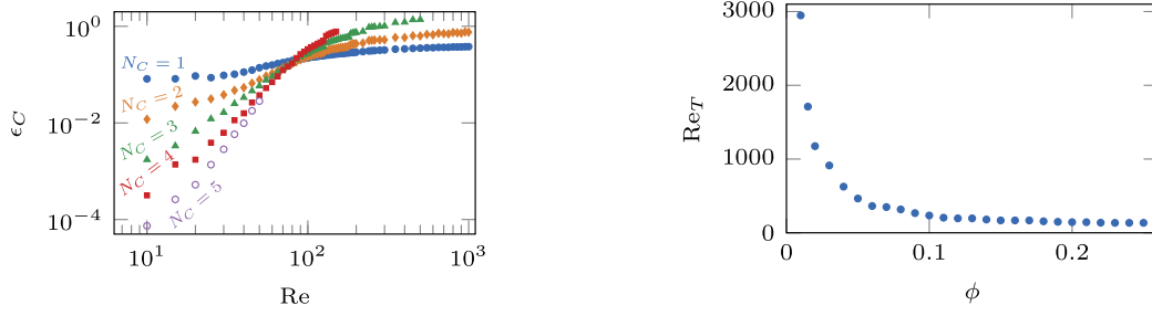
FIG. 2. Carleman truncation error and convergence for D = 1 . Left: truncation error \epsilon_C dependence on the Reynolds number Re and truncation order N_C for the D1Q3 model with \beta = 3/4 (corresponding to spatial discretization resolving the Kolmogorov microscale), u_0^* = 1 (enough to keep the norm of the solution below 1 at all times), and the initial sinusoidal state. Right: threshold value Re_T above which the Carleman truncation error \epsilon_C is larger for truncation order N_C = 2 than for N_C = 1 . Data for the D1Q3 model with \beta = 3/4 , u_0^* = 1 , and initial states given by colliding states with a fraction parameter \phi .
