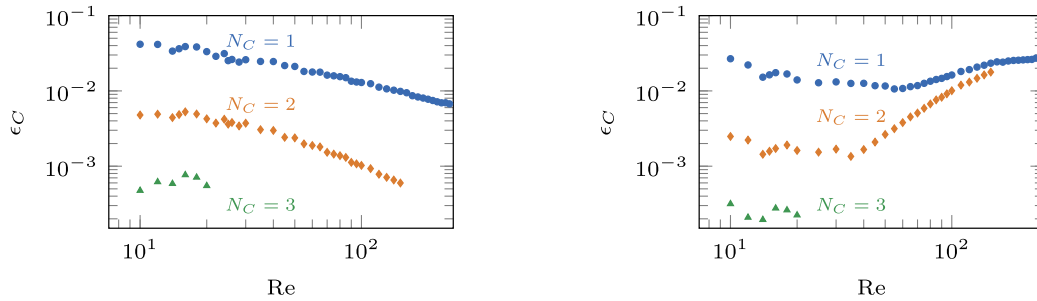
FIG. 5. Carleman truncation error \epsilon_C for D = 2 . Data for the D2Q9 model with \beta = 3/4 (corresponding to spatial discretization resolving the Kolmogorov microscale) and u_0^* = 1 (enough to keep the norm of the solution below 1 at all times). Initial states given by the Taylor-Green vortex (left) and Gaussian vortex dipole with s = \pi/2 and \sigma = \pi/5 (right).
