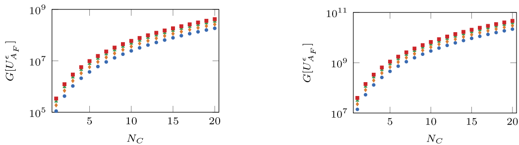
FIG. 8. T -gate cost of U_{A_F}^{\epsilon} . The estimates for the number G[U_{A_F}^{\epsilon}] of T gates needed to prepare a circuit \epsilon -close to a unitary U_{A_F} encoding the LBE problem with dimension D = 1 (left) and D = 2 (right) as a function of Carleman truncation order N_C . Different symbols, bottom to top, correspond to the allowed error level \epsilon = 10^{-3k} for k \in \{1, 2, 3, 4\} . Note that the dependence of G[U_{A_F}^{\epsilon}] on the Reynolds number \text{Re} is only logarithmic, making the presented data applicable with a very good approximation to all \text{Re} \geq 1 .
