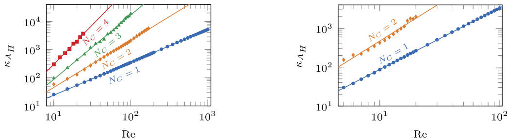
FIG. 7. Condition number. Scaling of the condition number \kappa(A_H) with the Reynolds number \text{Re} for the D1Q3 model (left) and D2Q9 model (right), and different Carleman truncation orders N_C . The considered systems have periodic boundary conditions with no walls and \beta = 3/4 .
