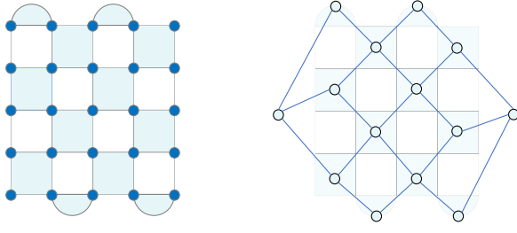
FIG. 11. Left: X stabilizer checks on the distance-5 rotated surface code. Each filled circle represents d_s^2 qubits comprising the code, and each light-blue square plaquette represents an X stabilizer check. Right: the corresponding error graph. Each vertex (open circles), except for the leftmost and rightmost, corresponds to an X stabilizer check, and each edge corresponds to a data qubit shared by two stabilizer checks. The leftmost (rightmost) vertex is a virtual vertex referred to as the left (right) boundary node.
