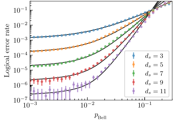
FIG. 16. Circuit-level simulation results of the logical error rate of logical Bell pairs generated by remote lattice surgery protocol, as a function of the physical Bell pair error rates p_{\text{Bell}} , with noise model of Table II. Solid curves are the fits to the data below the threshold with Eq. (A1). Error bars represent the standard error of estimated probability from the 10^7 sampling results.
