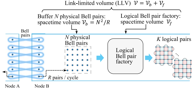
FIG. 2. Link-limited volume (LLV). LLV consists of network-related volume \mathcal{V}_b = N^2/R and Bell pair factory volume \mathcal{V}_f in each node [Eq. (1)], where N is the number of physical Bell pairs needed for the factory and R is the throughput of the physical Bell pairs, defined by the number of Bell pairs generated in the duration a single syndrome extraction cycle.
