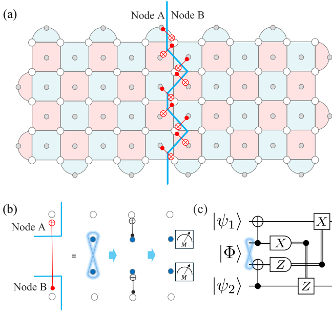
FIG. 15. Remote lattice surgery with rotated surface code. (a) The zig-zag interface for remote lattice surgery of a merged patch [26], where the blue line represents the interface between the two nodes and red CNOTs represent the teleported CNOT gates implemented by Bell pairs. (b),(c) Gate teleportation by physical Bell pairs. Remote Bell pair (blue circles) interacts with qubits in each node (white circles) via CNOT gates, before the Bell pair is measured for feedforward Pauli gates, as shown in (c).
