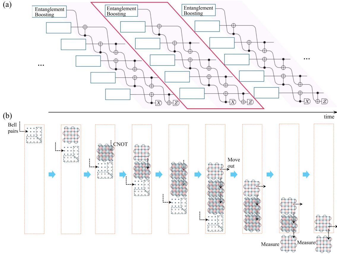
FIG. 8. Reconfigurable-qubit implementation of pipelined entanglement distillation with [[2m, 2m - 2, 2]] quantum parity code. (a) An example circuit for [[6, 4, 2]] code, distilling 4 logical Bell pairs out of 6 logical Bell pairs. The curved wires in the circuit represent the logical qubit reconfigurations, which move the location of the logical qubits for transversal CNOT gates. For example, we assume the input to the circuit originates from the entanglement boosting protocol. (b) More detailed illustration of qubit reconfiguration for one instance of the distillation in (a) (marked by red rhombus). The first two input qubits are moved along the vertical direction inside the Bell pair factory (orange rectangle), interacting with other qubits. Once the interactions are completed, they are moved out from the factory for logical X- and Z-basis measurements. Bell pair input and output can be directed along the horizontal axis, with sequential input of n boosted Bell pairs during the execution of the distillation.
