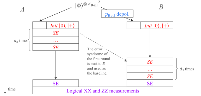
FIG. 10. Numerical simulation of the boosting stage described in Sec. IV. Steps in red are subject to the noise model shown in Table II, while the steps in purple (with underlines) are noiseless. We initially prepare d_{\text{Bell}}^2 Bell pairs and subjected one of the arms of the pairs to a single-qubit depolarizing channel. The remaining d^2 - d_{\text{Bell}}^2 physical qubits are prepared with noise strength 0.1% in each party. We simulate the SE steps of two parties in series for implementation purposes, which is equivalent to simultaneous SE operations followed by classical communication to exchange the syndrome information in an actual operation.
