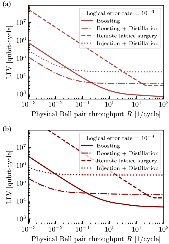
FIG. 17. Additional plots for the LLV as a function of physical Bell pair throughput R , for target logical error rates of 10^{-6} with d_s = 7 (a) and 10^{-9} with d_s = 13 (b), with the same error model as for Fig. 9(a), i.e. p_{\text{Bell}} = 1\% . Solid lines represent the entanglement boosting, the dash-dotted lines denote the boosting-and-pipelined distillation protocol with [[10, 8, 2]] quantum parity code, dashed lines indicate remote lattice surgery, and dotted lines are the injection-distillation approach using optimized sequence of [2, 1, 2]_X, [2, 1, 2]_Y , and [[8, 6, 2]] for (a), and [2, 1, 2]_X, [2, 1, 2]_Y , and [[8, 3, 3]] for (b). These optimized sequences are obtained using the open-source code accompanying Ref. [30] with buffer space of 10 logical qubits (see Appendix C 5).
