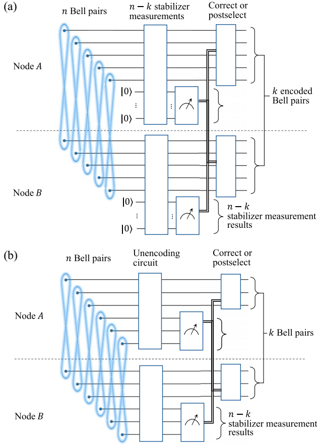
FIG. 1. Two entanglement distillation protocols based on [[n, k, d]] stabilizer code \mathcal{C} used in this work. (a) Auxiliary-qubit-assisted, projection-based preparation of logical Bell pairs from physical Bell pairs. Here, stabilizer checks of n Bell pairs are measured by n-k auxiliary qubits, allowing either post-selection or error correction to achieve k high-fidelity logical Bell pairs encoded in code \mathcal{C} . (b) A decoding-based approach, which combines the protocol in (a) and decoding of the encoded state, to result in k output Bell pairs. The stabilizer measurements are performed by the measurement of n-k qubits that do not constitute the output.
