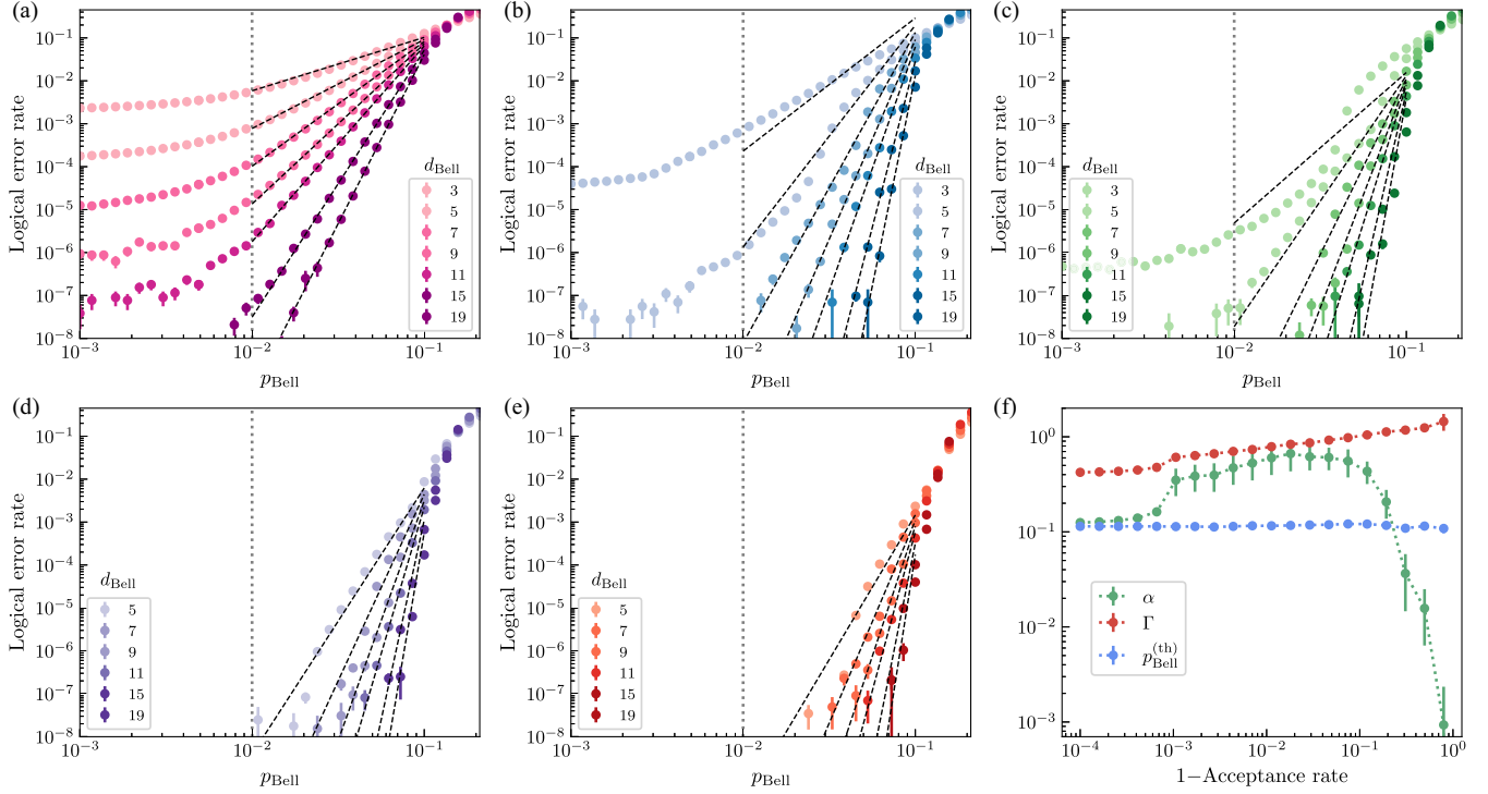
FIG. 14. Additional plots showing the scaling of the logical error rate for logical Bell pairs produced with the entanglement boosting protocol. (a–e) Logical error rate as a function of the physical Bell-pair error rate p_{\text{Bell}} for different d_{\text{Bell}} , with discard probabilities of 0% (a), 10% (b), 35% (c), 50% (d), and 70% (e), based on the complementary gap. Each point is obtained from circuit-level simulations of the entanglement boosting protocol with soft-output decoding and postselection based on varying complementary-gap thresholds that result in different discard probabilities. The dashed line represents the fitting with Eq. (2) in the range 10^{-2} < p_{\text{Bell}} < 9 \times 10^{-2} . In (d),(e), the statistics of the d_{\text{Bell}} = 3 simulation results are insufficient to obtain cases with complementary-gap-based discard rates reaching 50% or above; thus, no points are shown for d_{\text{Bell}} = 3 . (f) The dependence of the fitted values of parameters \alpha , \Gamma , and p_{\text{Bell}}^{(\text{th})} on the discard probabilities of entanglement boosting.
