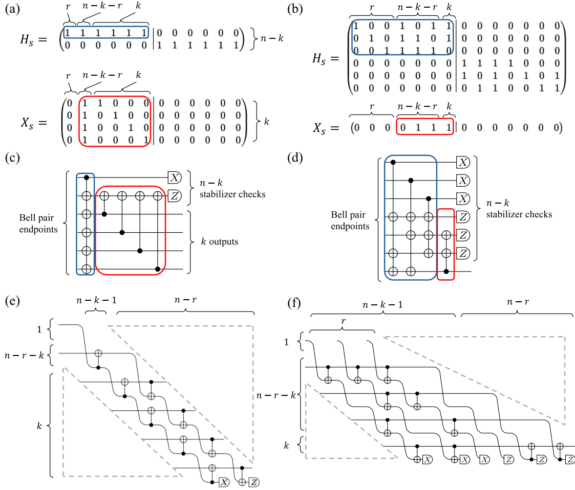
FIG. 7. Pipelined entanglement distillation based on CSS codes. (a),(b) Standard form of (n-k) \times 2n binary matrices H_s representing the stabilizer generators of [[6, 4, 2]] quantum parity code and [[7, 1, 3]] Steane code, along with binary matrix representation of logical X gates. (c),(d) Entanglement distillation circuit (only for one of the nodes shown), based on the encoding circuit synthesis of Ref. [51]. (e),(f) Same circuits as (c),(d), implemented with qubit reconfigurations (wire bending); see Fig. 8.
