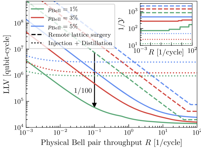
FIG. 6. Link-limited volume (LLV) to prepare a logical Bell pair encoded in the rotated surface code at logical error rates of 10^{-10} . We set the distance of the expanded surface code to be d_s = 19 . The dashed line is the corresponding LLV for the remote lattice surgery protocol for the rotated surface code (see Appendix A 5 and Refs. [25,26]), and the dotted line is the concatenated injection-distillation protocol (see Appendix C 4 and Ref. [30]) with corresponding colors for each p_{\text{Bell}} . At R = 0.1 , with d_{\text{Bell}} = 9 , d_s = 19 for entanglement boosting and d_s = 21 for remote lattice surgery, the improvement of the LLV from the remote lattice surgery to the entanglement boosting protocol is 100, mainly from the order-of-magnitude improvement of the yield while maintaining nearly the same V_f . (inset) The number of physical Bell pairs consumed per output logical Bell pair (inverse yield, 1/Y ). The jumps in the plots are due to the changes in optimal d_{\text{Bell}} that minimizes the LLV for varying R .
