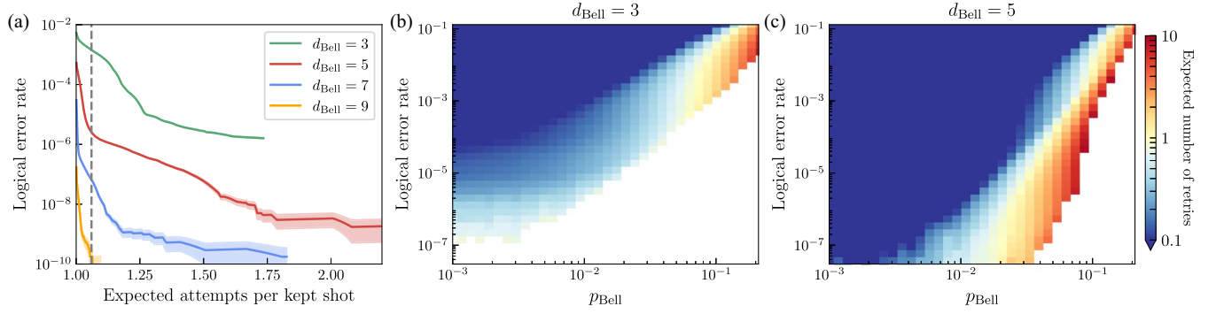
FIG. 4. Numerical simulation results for the entanglement boosting protocol. (a) Numerical simulation results of the logical error rates of the logical Bell pairs generated by the entanglement boosting protocol, for varying postselection criteria, for d_{\text{Bell}} = 3, 5, 7 , and 9 , with d_s fixed at 19 and p_{\text{Bell}} = 0.01 . Varying threshold values for the complementary gap results in different acceptance rate q_0 ; here, the logical error rate is shown for varying expected attempt count per kept shots, 1/q_0 . The shaded region is the standard error of estimated probability from 10^{10} sampling results. At d_{\text{Bell}} = 9 , logical error rate of 10^{-10} is reached at the expected attempts per kept shot of 1.06 (vertical gray dashed line): a logical Bell pair with logical error rate of 10^{-10} is prepared with an average of 86 noisy physical Bell pairs having p_{\text{Bell}} = 1\% . (b), (c) Numerical simulation results for the expected number of retries (colors), 1/q_0 - 1 , to achieve target error rates (vertical axis) for varying input Bell pair error rates p_{\text{Bell}} (horizontal axis) over two orders of magnitude, for d_{\text{Bell}} = 3 and 5 .
