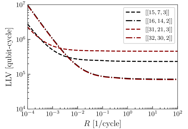
FIG. 18. Additional evaluation of the LLV for the combined boosting + pipelined distillation protocol, with four different quantum error-correcting codes used for the pipelined distillation, with p_{\text{Bell}} = 0.01 and target logical error rate of 10^{-12} . Here, quantum parity codes [[2m, 2m - 2, 2]] with m = 8 (black dash-dotted line) and m = 16 (red dash-dotted line), and quantum Hamming codes [[2^\ell - 1, 2^\ell - 2\ell - 1, 3]] with \ell = 4 (black dashed line) and \ell = 5 (red dashed line) are used for the pipelined entanglement distillation.
