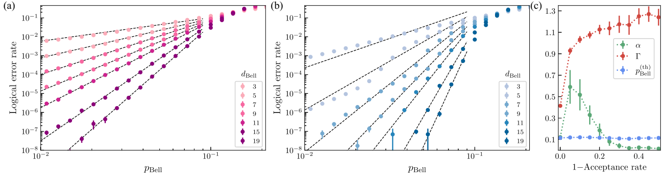
FIG. 5. Scaling of the logical error rate of the Bell pairs produced with the entanglement boosting protocol. (a),(b) logical error rate as a function of the physical Bell pair error rate p_{\text{Bell}} for different d_{\text{Bell}} , with acceptance rates q_0 of 100% (a) and 90% (b) based on the complementary gap. Each point is obtained from circuit-level simulations of the entanglement boosting protocol, and the dashed line represents the fitting with Eq. (2). Error bars represent the standard error of estimated probability from the 10^8 sampling results. (c) The dependence of the fitted values of parameters \alpha , \Gamma , and p_{\text{Bell}}^{(\text{th})} on the discard rates 1 - q_0 of entanglement boosting, where the error bars represent 95% confidence intervals. While p_{\text{Bell}}^{(\text{th})} remains nearly constant, the scaling prefactor \Gamma increases as a function of the discard rates.
