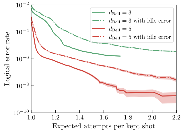
FIG. 13. Effect of idling errors on the logical error rates of logical Bell pairs generated by entanglement boosting. Here, we set p_{\text{Bell}} = 1\% and d_s = 19 , and physical operation errors are shown in Table II.
