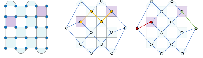
FIG. 12. Left: X stabilizer checks on the distance-5 rotated surface code. Z errors are detected by the purple checks. Middle: a solution of the MWPM problem conditioned with the left boundary check off. Right: a solution of the MWPM problem conditioned with the left boundary check on. Matching paths are shown in different colors.
