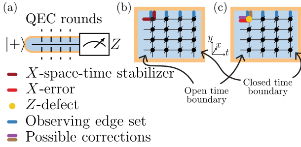
FIG. 6. A simple example of a fragile observable. (a) A |+\rangle reset followed by a Z -measurement, with four QEC rounds in between for ease of visualization. (b) The Z -detectors of the decoding hypergraph \mathcal{G} , with an X -space-time stabilizer and the observing edge set of the observable containing the Z -measurement. Because the observable is fragile, the observing edge set has odd overlap with the edges contained in the X -space-time stabilizer. (c) There are two equal-weight corrections to the weight-one measurement error shown, one of which flips the observable while the other one does not. In this simple circuit, it does not matter which decision the decoder makes because the observable has 50-50 measurement statistics anyway.
