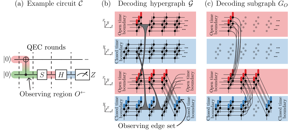
FIG. 4. The decoding hypergraph and subgraph G_O for an observable O for an example circuit. (Actually, the Z measurement observable which is decoded here happens to be fragile, and decoding fragile observables can be avoided for reasons discussed in Sec. III B 2.) (a) The observing region O^\leftarrow of the observable O being the Z -measurement is shown, where red, green, and blue shading regions indicate X , Y , and Z support, respectively. (b) The decoding hypergraph \mathcal{G} of the encoded circuit \mathcal{C} for the d = 3 unrotated surface code. The vertices of \mathcal{G} are partitioned based on the logical qubit to which they pertain and whether they represent X - (red background) or Z - (blue background) detectors. Note that the x and y spatial coordinates have been swapped between the X - and Z -detectors for ease of visualization. Also note that we have only shown the weight-3 hyperedges that appear on the top-front qubit to reduce clutter; weight-3 hyperedges with the same pattern also exist at all the other spatial coordinates in \mathcal{G} but are not shown here. We have also labeled all the edges that make up the observing edge set \mathcal{H}_O (in blue and red), and the open and closed time boundaries that arise from resets and measurements in (a). (c) The decoding subgraph G_O for the observable O . As explained in the text, G_O contains all the vertices V_O of \mathcal{G} that pertain to the same logical qubit and represent a detector of the same Pauli type ( X or Z ) as an edge in the observing edge set. It clearly has the property that it is a graph with no hyperedges. Vertices that are excluded from V_O are shaded in gray.
