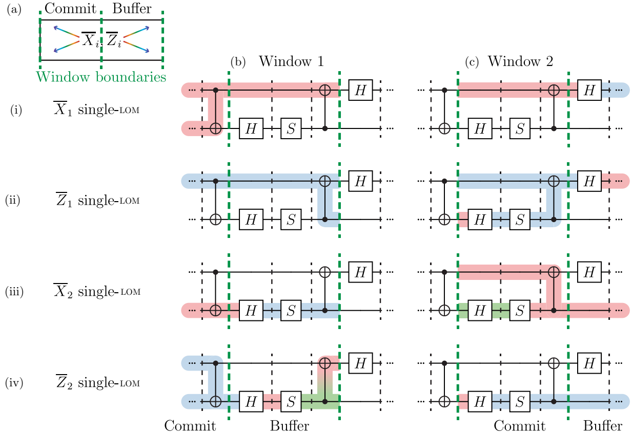
FIG. 19. (a) A visual representation of the windowed-LOM decoder, including both the buffer and commit regions. In each window, a single-LOM decoding instance is run on the track obtained by forward- and backward-propagating a single-logical-qubit \bar{X} or \bar{Z} from the center of the window. (b) and (c) A detailed example of the single-LOM tracks in two windows of the windowed-LOM decoder implemented on the d = 3 surface code, where red, green, and blue regions represent X , Y , and Z Pauli support, respectively.
