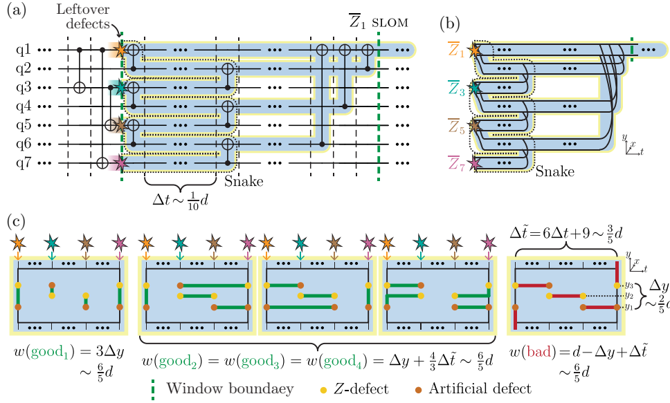
FIG. 25. The second window of decoding the errors from Figs. 22 and 23 along with the leftover defects from the first window of decoding in Fig. 24. We are only interested in the single-LOM corresponding to \bar{Z}_1 in the center of the window. (a) The propagation of the \bar{Z}_1 single-LOM through the circuit, with the locations of the leftover defects from the four single-LOMs from the first window shown. (b) The decoding subgraph of the single-LOM. Focusing only on the “snake” part of the subgraph and flattening it out gives the representation in (c), which shows five possible corrections to the leftover defects in the single-LOM. The temporal length \Delta \tilde{t} is the length of the snake; note that it includes a constant offset (nine in this example) due to the turns of the snake. The first four corrections shown are good because they correspond to corrections in the same logical class as the physical error that occurred, while the last one is bad because it causes a logical error equivalent to an \bar{X}_1 error in the middle of the second window. All five corrections have weight \sim 6d/5 , despite being caused by a physical error of weight only \sim 2d/5 .
