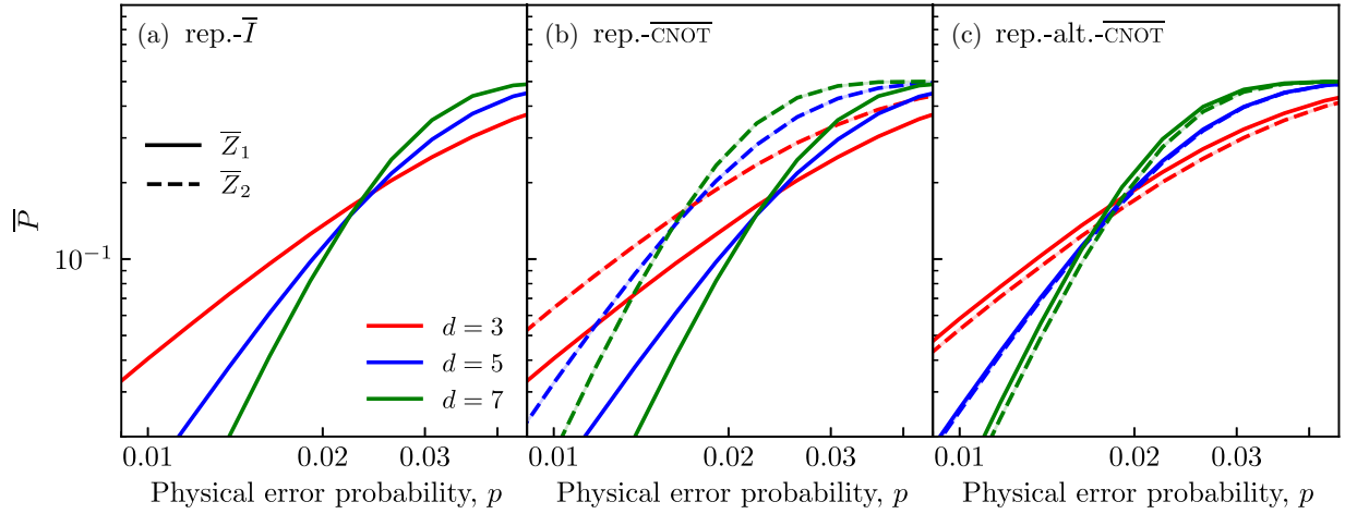
FIG. 13. Focusing on single logical observables for the two-qubit repeated-gate experiments under phenomenological noise. As one may expect, the performance of \bar{Z}_1 in the repeated- \overline{\text{CNOT}} experiment in (b) matches the performance of the repeated- \bar{I} experiment in (a) while \bar{Z}_2 , being sensitive to logical X errors on both qubits, performs worse. For the alternating- \text{CNOT} experiment, the logical error rates of \bar{Z}_1 and \bar{Z}_2 are symmetrized. The 95% confidence intervals are shown as shaded regions but they are too small to be visible.
