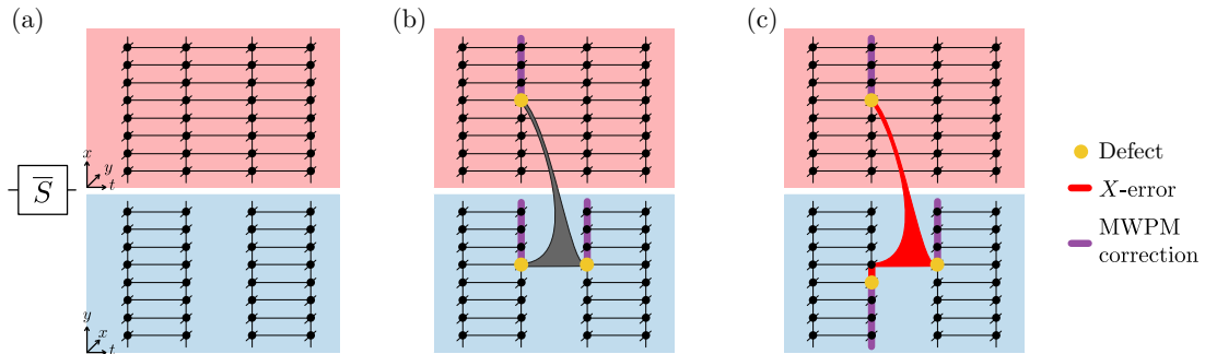
FIG. 3. Hyperedge decomposition and error combination that explains the bad performance of a “splitting-hyperedge” matching decoder in the pre-gate frame. (a) \mathcal{G}_{\text{matchable}} of the \bar{S} gate, which is built by only taking the edges from the decoding hypergraph in Fig. 2. (b) The procedure from Ref. [23] to decompose the gray hyperedge goes as follows: (1) the detectors involved in the hyperedge are triggered (yellow dots), (2) such syndrome is decoded with MWPM using \mathcal{G}_{\text{matchable}} , and (3) the correction (purple edges) corresponds to the hyperedge decomposition. Note that the number of purple edges in the decomposition can badly grow with the code distance. (c) The two errors marked in red lead to a logical error when decoded using \mathcal{G}_{\text{matchable}} , thus the logical scaling is at most O(p^2) for any distance.
