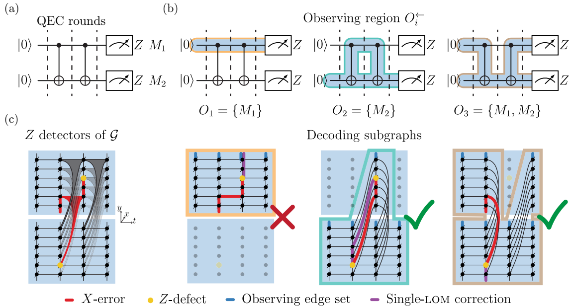
FIG. 5. An example of a weight-5 error in the d = 7 surface code in which the decoded outcomes for the reliable observables O_1 , O_2 , and O_3 = O_1 O_2 are inconsistent. (a) The circuit consists of two consecutive CNOT gates, with both qubits initialized and measured in the Z-basis. The logical action of the circuit is trivial here and only serves as a simple example. (b) The observing regions of the three observables. (c) The Z-detectors in the decoding hypergraph \mathcal{G} . For simplicity, only a slice of \mathcal{G} is shown for a fixed value of the spatial coordinate x . When each of the observables is decoded by the single-LOM decoder, it predicts a flip in the observable O_1 but not in O_2 or O_3 , despite the fact that O_3 = O_1 O_2 . This is only possible because the weight of the error—five—is greater than d/2 = 7/2 . Note that in this figure and throughout, we will refer to measurement errors of Z-stabilizers as X-errors (and vice versa for X-stabilizer errors) for simplicity.
