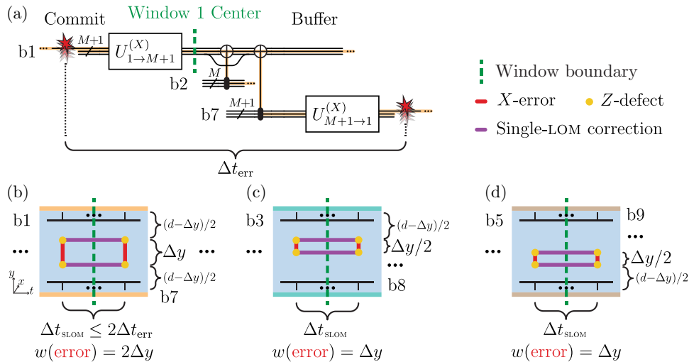
FIG. 27. The first window of decoding the error from Fig. 26. Each \bar{Z}_i single-LOM with i representing a qubit in blocks 1, 3, or 5 are relevant for our example. (a) The propagation of an arbitrary block-1-single-LOM for \bar{Z}_n , n = 1, \dots, M + 1 through the circuit. Similar structures are followed for the other single-LOMs in this window. (b)–(d) The decoding subgraphs of single-LOMs in blocks 1, 3, and 5 (respectively), along with the errors and corrections in each single-LOM. The artificial defects from each single-LOM appear in the second window and cause a logical error in decoding, as shown in Fig. 28.
