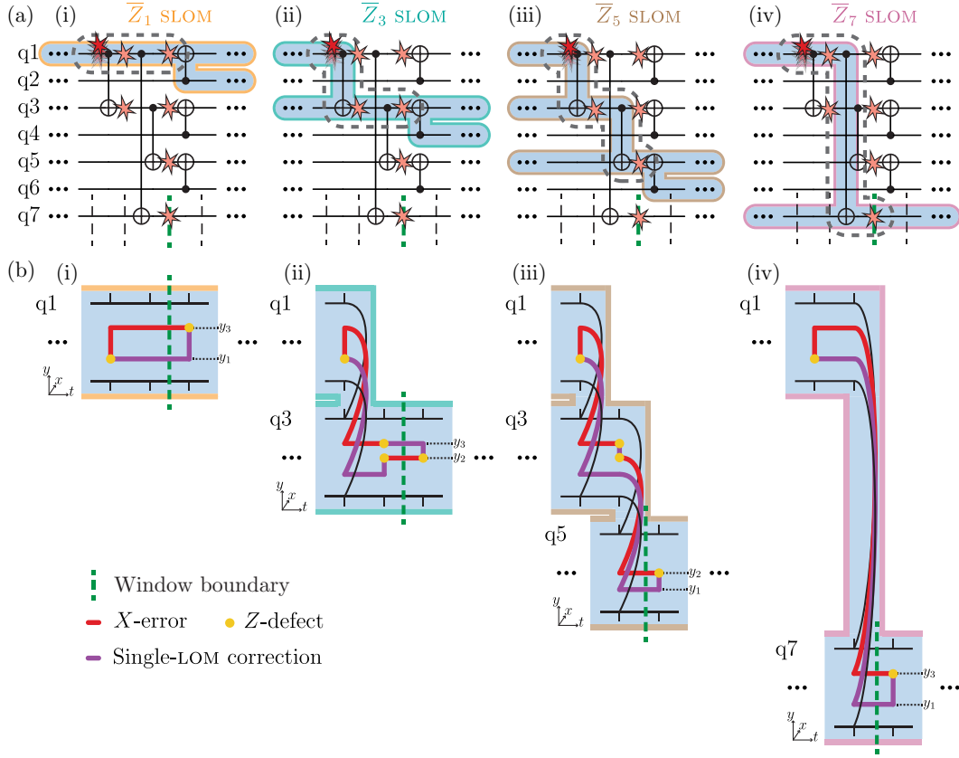
FIG. 24. The first window of decoding the error from Figs. 22 and 23. We are only interested in four of the iterations of the single-LOM (abbreviated SLOM in the figure), corresponding to the \bar{Z} operators on logical qubits (i) 1, (ii) 3, (iii) 5, and (iv) 7 in the center of the window. (a) The propagation of each single-LOM through the circuit. (b) The decoding subgraph of each single-LOM, focusing only on the regions containing physical errors, as shown by the gray dotted regions in (a). In order to create a logical error in the second window, the correction in each single-LOM decoder must follow the pattern shown in purple. Each correction is one of multiple minimum-weight corrections in each single-LOM.
