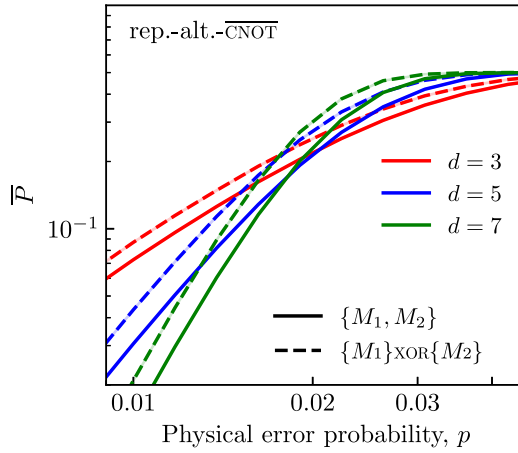
FIG. 14. Performance of the LOM decoder for the \bar{Z}_1\bar{Z}_2 observable of the repeated-alternated- \overline{\text{CNOT}} when using two different methods of obtaining the logical correction. The “ \{M_1, M_2\} ” method corresponds to running a single-LOM decoder for the \bar{Z}_1\bar{Z}_2 observable. The “ \{M_1\}\text{XOR}\{M_2\} ” method corresponds to running single-LOM decoders for the \bar{Z}_1 and \bar{Z}_2 observables separately and then obtaining the error-corrected \bar{Z}_1\bar{Z}_2 outcome by taking their XOR. The circuit is run with phenomenological depolarizing noise. The 95% confidence intervals are shown as shaded regions but they are too small to be visible.
