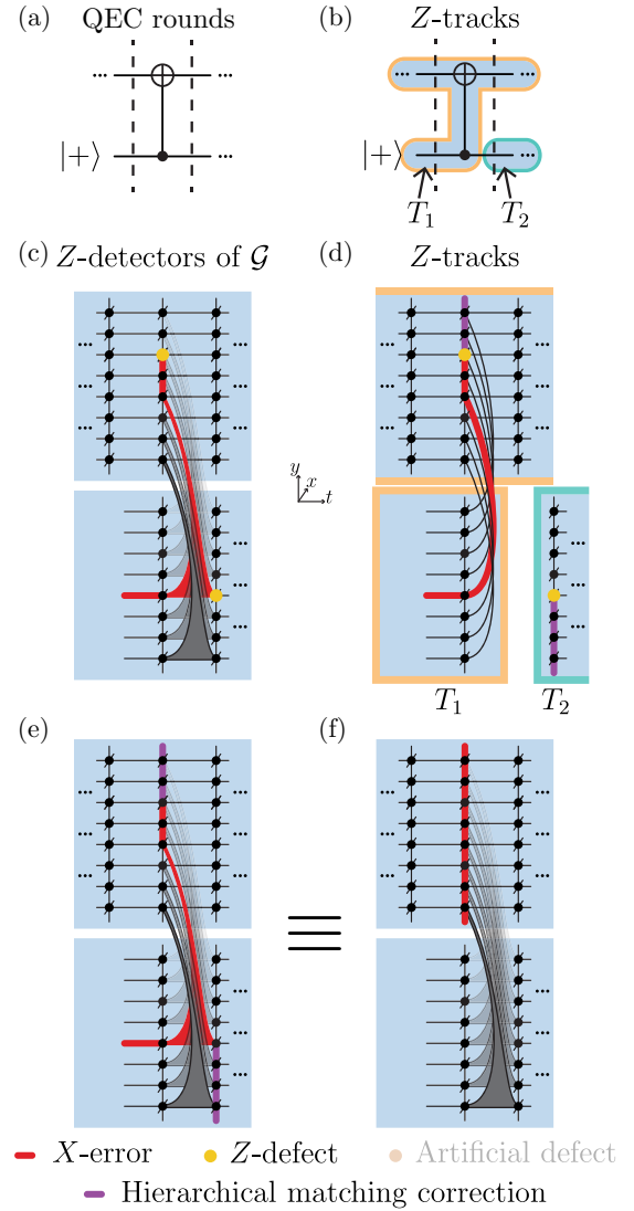
FIG. 21. An example of a failure of hierarchical matching due to the presence of a fragile time boundary in the first track. (a)–(e) The circuit, tracks, error, action of the hierarchical matching decoder, and the final correction for the error, respectively, similar as in Fig. 8. The error + correction in (e) can be multiplied by space-time stabilizers to the error string in (f), which corresponds to a logical X -error on the top qubit in (a). The physical error here has weight 4 < 9/2 = d/2 . Note also that although we have suggested that the circuit extends in both time directions in the figure, this example still works if, say, the first qubit is initialized in |0\rangle .
