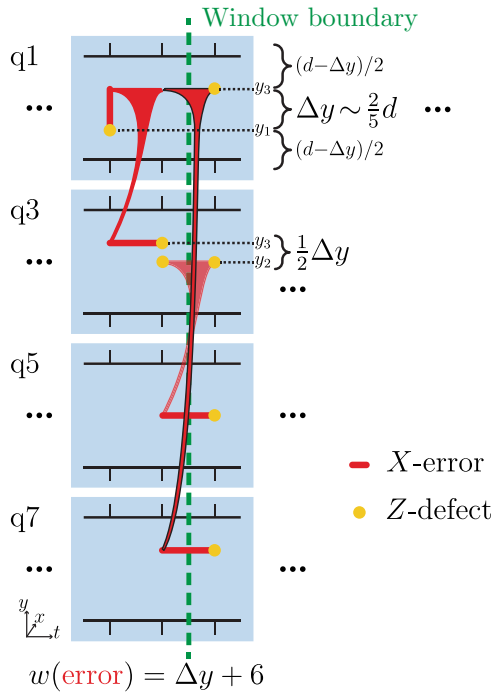
FIG. 23. A simplified representation of the decoding hypergraph \mathcal{G} showing the X -error pattern of weight 2d/5 + 6 in the circuit in Fig. 22 that leads to a logical error when decoded by the windowed-LOM decoder. Only the slice of the circuit in Fig. 22 where the physical errors occur is shown in the figure. For ease of visualization the space and time coordinates are not to scale; each interval in time represents just one time-like edge.
