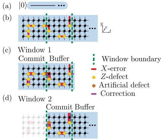
FIG. 18. The operation of a sliding window matching decoder on a Z -basis memory experiment, shown in (a), in the d = 5 surface code. (b) The Z -detectors in the first rounds of the full decoding graph with an arbitrarily chosen set of X -errors. The decoding problem is split into overlapping windows, the first two of which are shown in (c) and (d), including their respective buffer and commit regions and the correction that they apply. Note that only the correction in the commit region of window 1 is committed to, giving rise to an artificial defect in window 2.
