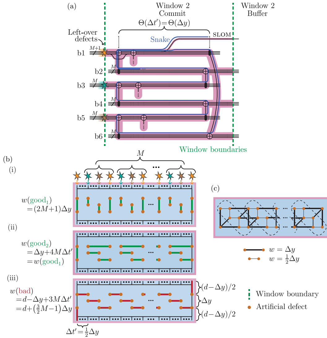
FIG. 28. The second window of decoding the leftover defects from the errors and corrections in Figs. 26 and 27. We are only interested in the single-LOM corresponding to \bar{Z}_1 , shown shaded in (a). We also show in dark blue the structure of the snake, which wriggles from the first qubit in block b1, then to the first qubit in each of the blocks in turn down to b6, before returning to the second qubit in block b1, and so on. On blocks b1, b3, and b5 artificial defects are created at different spatial locations according to Figs. 27(b)–27(d). (b) Some good and bad corrections. (c) The matching graph of the artificial defects, with edges to the boundaries removed, used in the arguments in Lemma B1. The weight of each edge is indicated by the thickness of the line and follows the Manhattan distance. The dashed ovals indicate each “descending staircase” of defects, as used in Lemma B1.
