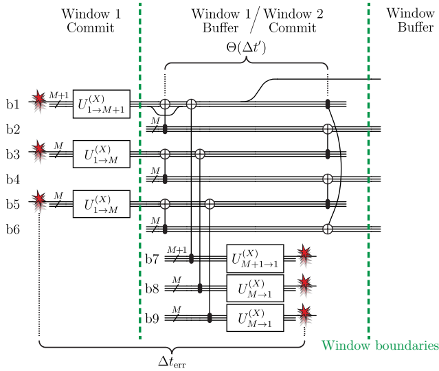
FIG. 26. A circuit \bar{C} with 9M + 2 logical qubits in which an error which scales less than linearly in d can cause a logical error when decoded by the windowed-LOM decoder. We represent the logical qubits in nine blocks of M or M + 1 qubits labeled b1–b9. CNOT gates between the blocks represent independent logical CNOTs between the m th qubit in the first and the m th qubit in the second block. The U -gates are defined in Eq. (B1). Note that we also split off individual logical qubits from block 1 in some of the CNOTs, either from the top of the block or from the bottom. X -data-qubit-errors occur in six circuit locations, the coordinates of these errors are shown in detail in Fig. 27.
