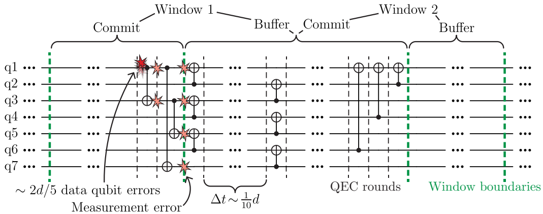
FIG. 22. A circuit \bar{C} with seven logical qubits, each encoded in the unrotated surface code of distance d . An error of weight \sim 2d/5 can cause a logical error when decoded by the windowed-LOM decoder, in the absence of short-cut edges. The error occurs at seven locations in the circuit: the first set of errors consists of \sim 2d/5 X -errors on data qubits immediately before the first CNOT gate, while the remaining errors are single measurement errors on Z -stabilizer measurements during a QEC round. No other physical errors occur. The precise configuration of the X errors is shown in Fig. 23. The error will be decoded in two windows (1 and 2) of width > d , whose commit and buffer regions are labeled above the circuit. We will show in Figs. 23–25 that a logical error will be inferred for the \bar{Z}_1 operator at the end of the circuit.
