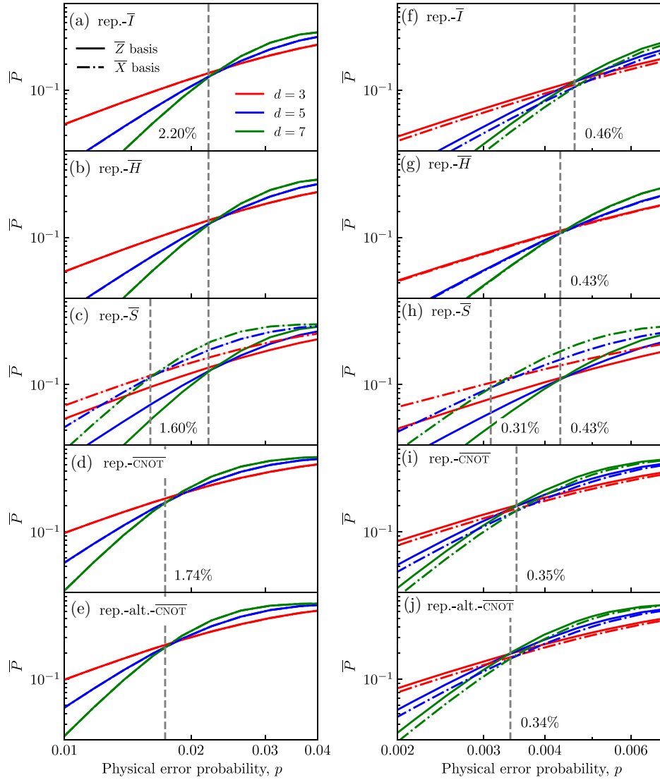
FIG. 12. Logical error probability of the LOM decoder as a function of the physical error probability for the repeated-gate experiments under (a)–(e) phenomenological depolarizing noise and (f)–(j) circuit-level noise for the pre-gate frame. In the experiments, each logical operation is followed by one QEC round, thus d + 2 rounds are performed, see Fig. 10(a). The vertical dashed gray lines indicate the crossing of \bar{P} for the d = 5 and 7 surface codes. The 95% confidence intervals are shown as shaded regions but they are too small to be visible.
