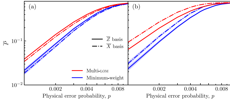
FIG. 16. Performance comparison between LOM and (approximate) minimum-weight decoding for (a) the two-qubit memory experiment and (b) circuit [Eq. (5)] for the distance-3 unrotated surface code under circuit-level noise. The solid (dashed) line corresponds to the experiment in the \bar{Z} - (respectively, \bar{X} -) basis. The shaded regions show the confidence interval with 95% confidence level. Note that for the LOM decoder, the interval is too small to be visible.
