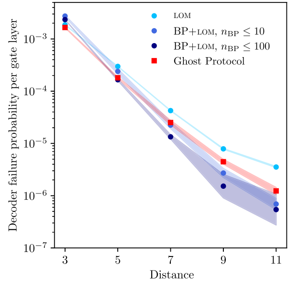
FIG. 17. Decoder failure probability per gate layer of the LOM, BP+LOM, and Ghost Protocol [25] decoders for the deep Clifford circuit with a single QEC round per gate layer and noise model from Ref. [25]. The circuit has 32 gate layers, where each layer is composed of random transversal \{H, X, Y, Z\} gates followed by random transversal CNOTs on each qubit. All distances have been simulated with the same noise strength p = 10^{-3} . The parameter n_{BP} in BP+LOM corresponds to the maximum number of belief-propagation iterations that are run. The shaded regions show the confidence interval with 95% confidence level. Note that, for n_{BP} = 100 at distances 9 and 11, the confidence intervals are quite large as only \sim 10 decoding failures have been sampled due to longer decoding runtimes.
