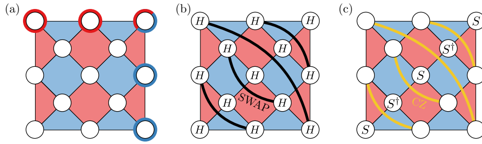
FIG. 1. (a) The d = 3 unrotated surface with data qubits as white circles and X - (respectively, Z -) stabilizers as shaded red (respectively, blue) regions. Representatives of the Pauli \bar{X} (respectively, \bar{Z} ) are shown by the red (respectively, blue) circles around the data qubits on which it has support. (b) and (c) The fold-transversal \bar{H} and \bar{S} gates, respectively. The logical Hadamard gate is implemented as a layer of Hadamard gates followed by a layer of SWAP gates. The long-range SWAPs (respectively, CZs) are shown as thick black (respectively, yellow) lines.
