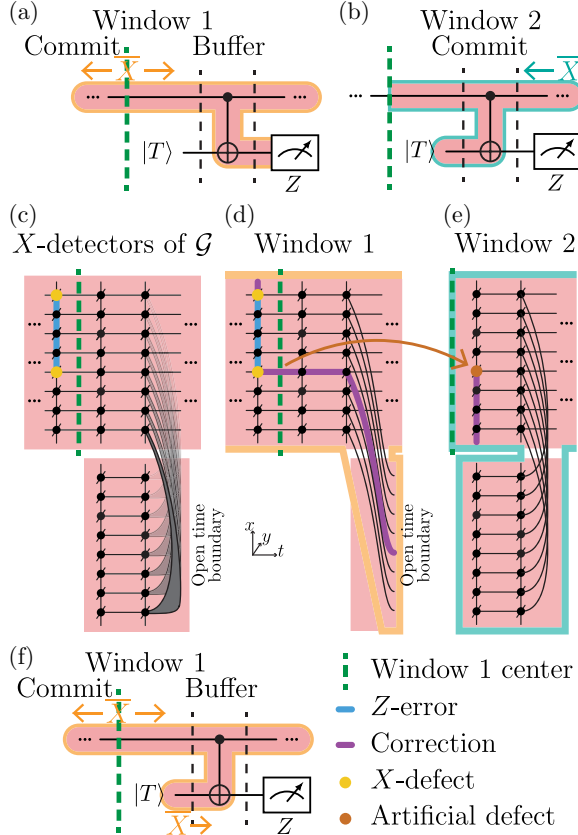
FIG. 20. (a) An example of a fragile time boundary in the forward direction, in which a logical X operator at the window boundary propagates forward to the logical Z measurement that it anticommutes with. Since the window boundary of the windowed-LOM decoder is too close (less than d/2 time-edges away) to the logical Z measurement, a low-weight error can subsequently cause a logical error in a single-LOM decoder in window 2, shown in (b). (c) An example of a weight-4 error in the d = 9 surface code that will cause a logical error. In general the weight of the error is d/4 + O(1) . (d) The correction that the single-LOM decoder shown in (a) makes involves matching to the fragile time boundary, causing an artificial defect in window 2. (e) The correction of this artificial defect in a single-LOM in window 2 that leads to a logical error. Note that in window 2 we backpropagate the logical X and therefore have no support on this fragile-time boundary. (f) A modification to the single-LOM in (a) avoids this issue by “peeling” the single-LOM off the fragile time boundary and onto the closed time boundary arising from the fault-tolerant state preparation of |\bar{T}\rangle .
