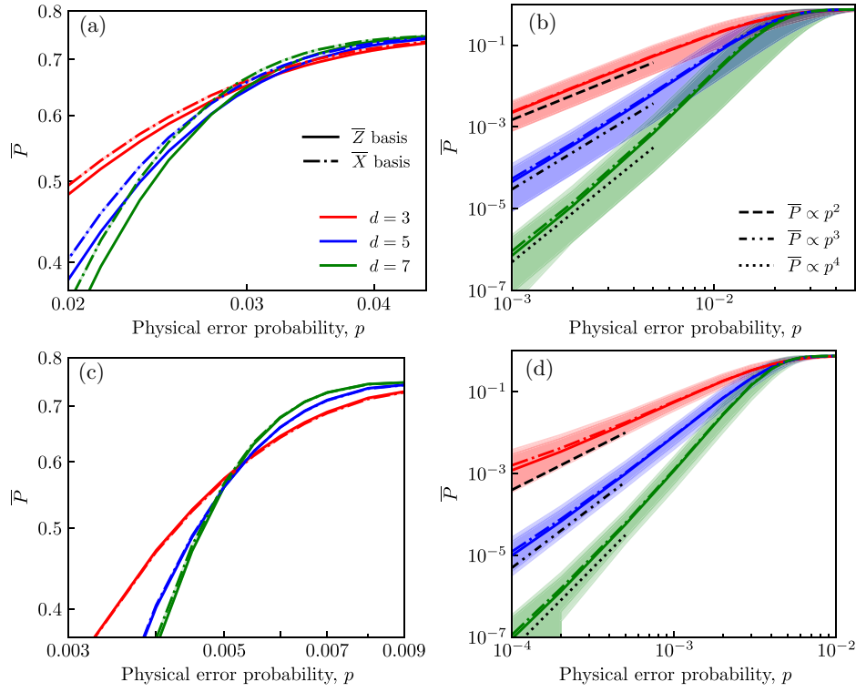
FIG. 15. Logical error probability of the LOM decoder as a function of the physical error probability for the two-qubit Clifford experiments in the pre-gate frame under (a) and (b) phenomenological and (c),(d) circuit-level noise. The solid (respectively, dashed) line corresponds to the average over all experiments in the \bar{Z} - (respectively, \bar{X} -) basis. The shaded regions in (a) and (c) are the 95% confidence intervals, but they are too small to be visible. The shaded regions in (b) and (d) show the best and worst performance across all circuits.
