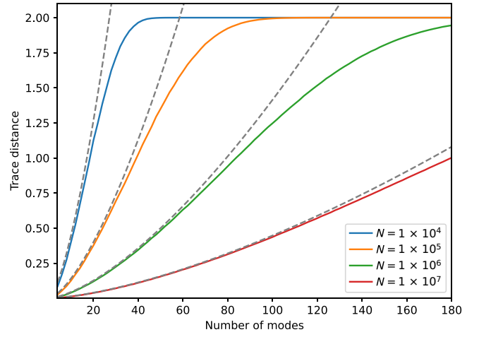
FIG. 2. Numerical simulation of the performance of the fermionic tomography algorithm for pure Gaussian states. We consider different numbers of total measurement rounds N as a function of the number of modes. The fit (dotted gray line) uses \varepsilon = 2n^{3/2}N^{-1/2} , where \varepsilon denotes the trace-distance error. The data are averaged over 50 randomly selected Gaussian states each.
