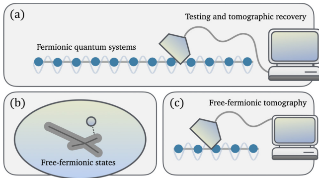
FIG. 1. (a) Testing free-fermionic quantum states and improved tomography. (b) Any procedure aiming to solve the property-testing problem for possibly mixed free-fermionic states must have a sample complexity scaling exponentially with the system size. Low-rank free-fermionic states can, however, be efficiently and robustly tested. (c) We then show sample optimal bounds for quantum state tomography for free-fermionic states. Our results strongly rely on a new set of inequalities that we derive concerning the distance of free-fermionic states (which constitute a nonconvex set) and the distance between their respective, efficiently tractable, correlation matrices (which form a convex set).
