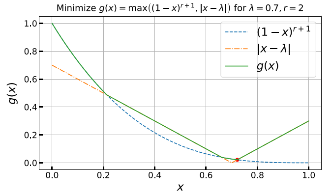
FIG. 3. A plot illustrating the behavior of the objective function g(x) = \max\{(1-x)^{r+1}, |x-\lambda|\} , which arises in Eq. (B113), where \lambda = 0.7 and r = 2 . The red point indicates the location of the minimum value of the function.
