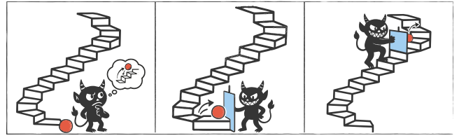
FIG. 8. Information-driven motion. A microscopic particle moves within a spiral-staircase potential, where thermal fluctuations cause it to randomly jump between steps. By measuring the particle's position at regular intervals, we can determine when it jumps upwards. This allows us to implement a feedback mechanism by placing a block behind the particle, preventing subsequent downward jumps. Repeating this process allows the particle to move up the staircase. Ideally, the energy required to position the block is negligible, meaning the particle's motion is driven purely by the information obtained from measuring its position. Figure inspired by Ref. [125].
