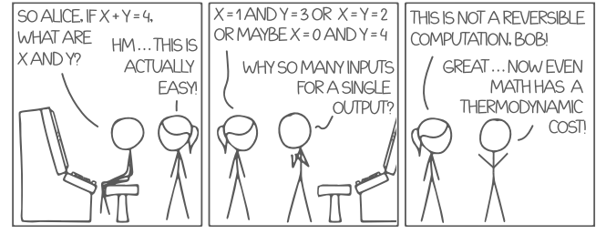
FIG. 12. Without a history tape, no such a thing as a free lunch. Imagine a machine that does nothing but adding numbers. If the machine outputs the number four, and Bob asks Alice to figure out the inputs that resulted in this number by running the process backward, she immediately encounters a problem. The inputs could have been one and three, or zero and four, among many other combinations. This fundamentally illustrates the concept of irreversibility: there is no single inverse solution, but rather a range of possibilities that could lead to the same outcome of four. Illustration inspired by XKCD [162].
