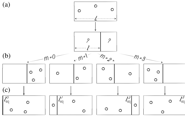
FIG. 5. Quantum Szilard engine . Three quantum particles are confined in a box of size L . (a) A partition is installed at location l , and (b) a measurement is made revealing the number m of particles on the left. (c) Then, the particles expand isothermally until they reach equilibrium at l_{eq}^m , and the partition is removed.
