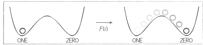
FIG. 9. Restoring to ZERO. A bistable potential with a particle can be recast as an information-restoring process by assuming the particle represents a bit, with its two states corresponding to the left (ONE) and right (ZERO) positions. The task consists of moving the particle from left to right using a conservative force F(t) regardless of its initial position. However, such a task is not possible as this process cannot be reversed.
