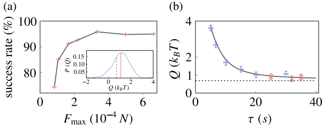
FIG. 11. Success rate and dissipated heat. Panel (a) shows the success rate of the erasure cycle as a function of the maximum tilt. The inset presents the heat distribution, with the solid red line indicating the average dissipated heat, and the dashed vertical line marking the Landauer bound. Panel (b) displays the average dissipated heat as a function of the protocol duration, measured for three success rates: blue for r \geq 0.9 , red for r \geq 0.85 , and green for r \geq 0.75 . The horizontal dashed line represents the Landauer bound. These figures have been adapted from Ref. [145], with minor edits for consistency with this tutorial, while retaining their original meaning.
