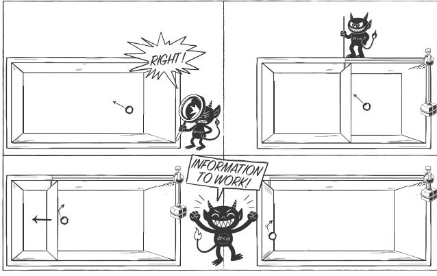
FIG. 4. Szilard engine . A chamber containing a single particle (atom or molecule) is initially in an unknown position. A demon measures the particle's position and inserts a movable, massless wall with an attached mass. As the gas in the chamber expands at a constant temperature, the attached mass is raised, resulting in work being performed. This mechanism appears to enable the conversion of information into useful energy, seemingly contradicting the second law of thermodynamics, as the demon extracts heat from the heat bath and converts it fully into mechanical work.
