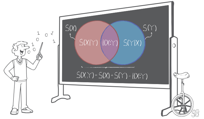
FIG. 7. Information diagram. Venn diagram illustrating the relationships among the joint entropy S(X, Y) , individual entropies S(X) and S(Y) , conditional entropies S(X|Y) and S(Y|X) , and mutual information I(X : Y) . Next to it, we see Shannon's unicycle and some of his juggling balls, as he was known for often doing both simultaneously.
