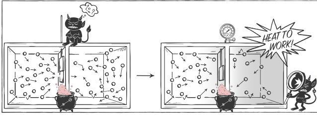
FIG. 3. Pressure demon . A less intelligent demon controls a door between two gas chambers connected by a constant temperature reservoir. As gas molecules approach the door, the demon selectively opens and closes it, allowing only right-moving molecules to pass in one direction and only left-moving molecules to pass in the opposite direction. This strategy increases the pressure on one side of the system while decreasing it on the other. The demon's actions convert heat from the reservoir into work, seemingly in violation of Kelvin's statement of the second law of thermodynamics.
