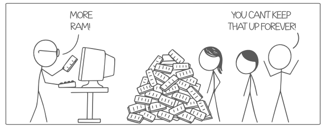
FIG. 14. Without erasure, there is no end to lunch. Imagine a computer scientist determined to avoid the thermodynamic cost of erasure. Instead of deleting information, they endlessly accumulate RAM, offloading used memory into an ever-growing pile. While reversible computation avoids heat dissipation, storing every intermediate state demands increasingly more resources. Eventually, the physical burden becomes unsustainable. Illustration inspired by XKCD [162].
