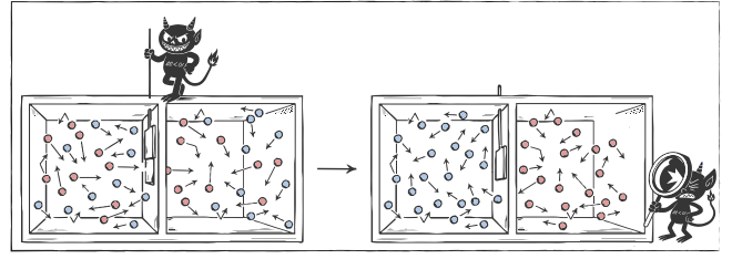
FIG. 2. Temperature demon . An intelligent being, a demon, controls a door between two gas chambers. As gas molecules approach the door, the demon selectively opens and closes it, allowing only fast molecules to pass one way and slow molecules the other. Since the kinetic temperature of a gas is directly linked to the velocities of its constituent molecules, the demon's strategy results in one chamber warming up while the other chamber cools down. This reduces the overall entropy of the system without requiring any work, thereby violating the second law of thermodynamics.
