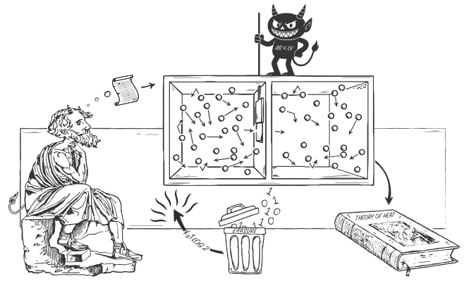
FIG. 1. Maxwell’s Gedanken experiment . In 1867 James Clerk Maxwell addressed a letter to Peter Guthrie Tait with the provocative idea that the second law is a statistical principle that only holds on average [13]. There, he introduced his famous demon—an intelligent being capable of sorting gas molecules by their velocities. By creating a temperature difference, the demon apparently defies the second law of thermodynamics, decreasing the system’s entropy without expending energy. Later on, this apparent paradox appeared in his book “ Theory of Heat ” [12].
