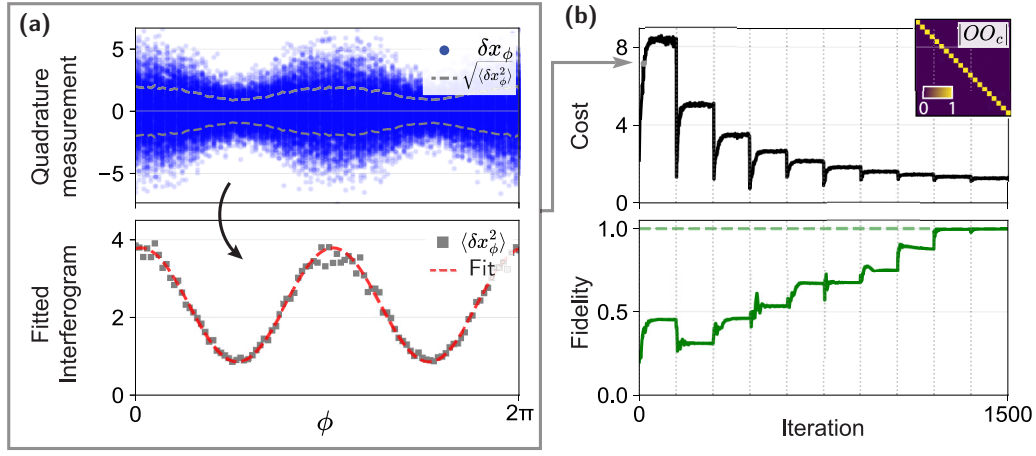
FIG. 2. Numerical simulation of variational learning of multimode squeezed light. (a) Simulated quadrature measurement, and the corresponding homodyne interferogram signal for the quadrature variance. The interferogram is fitted according to Eq. (3) and the cost function extracted according to the Supplemental Material, Section S2B [38]. (b) Plotted cost function [Eq. (4)] and overall Hilbert-Schmidt fidelity \text{Tr}|OO_C|/2N as a function of iteration number, where |\cdot| denotes element-wise absolute value. The inset shows the product |OO_C| to reflect the high fidelity between O_C and O^T .
