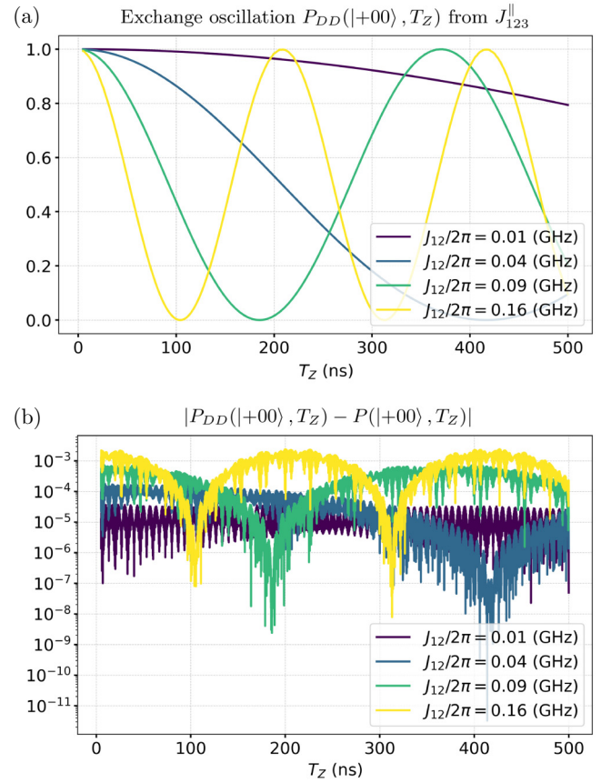
FIG. 5. Measurement of the chiral anisotropic exchange interaction using a four-layer DD sequence. We consider the full three-qubit Hamiltonian (including all flip-flop terms) for the optimal SOI configuration of the C^2Ry(\pi) gate [see Fig. 4(c)] with two-body exchange interaction strength J_{12}/2\pi = J_{23}/2\pi given by 10 MHz (purple), 40 MHz (blue), 90 MHz (green), and 160 MHz (yellow). (a) Exchange oscillations induced by the three-qubit interaction J_{123}^{\parallel} , obtained from numerical simulations of the measurement circuit introduced in Eq. (48). (b) Measurement error. Absolute difference between the expected probability curve, given by Eq. (49), and the numerically computed oscillation curve. Both plots are shown as a function of the free-evolution time T_Z \in [5, 500] ns. Notably, at all considered T_Z , the deviation between the numerical and expected oscillation curves remains below 10^{-3} .
