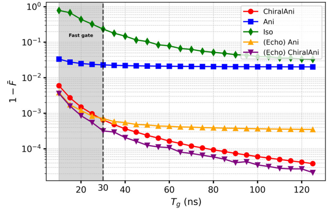
FIG. 3. Gate infidelity vs T_g with flip-flop interactions. We present the Iso gate (green), Ani gate (blue), ChiralAni gate (red), and their echo variants (yellow and purple, respectively). We exclude qubit phase-correction gate times and single-qubit gate times for the echo variants, as these are typically fast or can be accounted for with software. The plot is divided into two regions: (i) the fast regime (shaded), where the ( Echo ) Ani gate outperforms the ChiralAni gate, and (ii) the normal regime, where the ChiralAni gate performs better.
