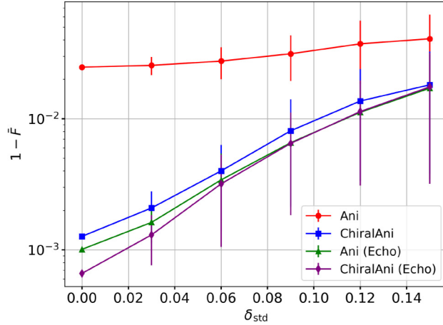
FIG. 6. Gate performance with noise. Numerical simulation with qubit frequencies \omega_1/2\pi = 4.2 GHz, \omega_2/2\pi = 4.5 GHz, and \omega_3/2\pi = 4.8 GHz. Exchange interactions are J_{12}/2\pi = J_{23}/2\pi = 20 (90) MHz and J_{13}/2\pi = 1.6 MHz for normal (fast) gates with gate time T_g = 100 (22.22) ns. The Ani gate follows the (0, 1) synchronization, with Rabi frequencies \Omega_2/2\pi \approx 5.16 (23.24) MHz, while the ChiralAni gate follows (0, 1, 1, 2), with \Omega_2/2\pi \approx 5.04 (22.68) MHz. The three-qubit interaction amplitude is J_{123}^{\parallel}/2\pi \approx 0.96 (4.34) MHz. We plot the gate infidelity under different noise sources for the anisotropic interaction (red), chiral anisotropic interaction (blue), and their Echo variants (green and purple, respectively). (a),(b) Gate infidelity against quasistatic error, where the noise is modeled as \delta_i(t) = \delta_i , drawn from a uniform distribution [-\delta_{\text{std}}, \delta_{\text{std}}] . (c),(d) Gate infidelity under high-frequency 1/f noise, modeled as a white noise with fluctuation \delta_{\text{std}} under infinite impulse response filter. Error bars represent \pm one standard deviation from the mean.
