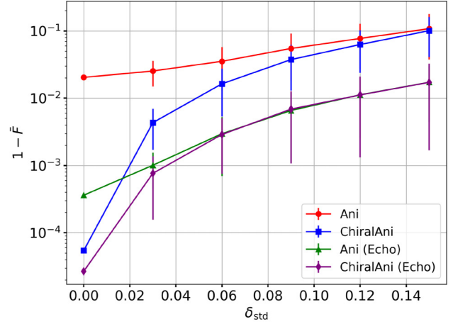
(b) Normal gate under quasi-static error
