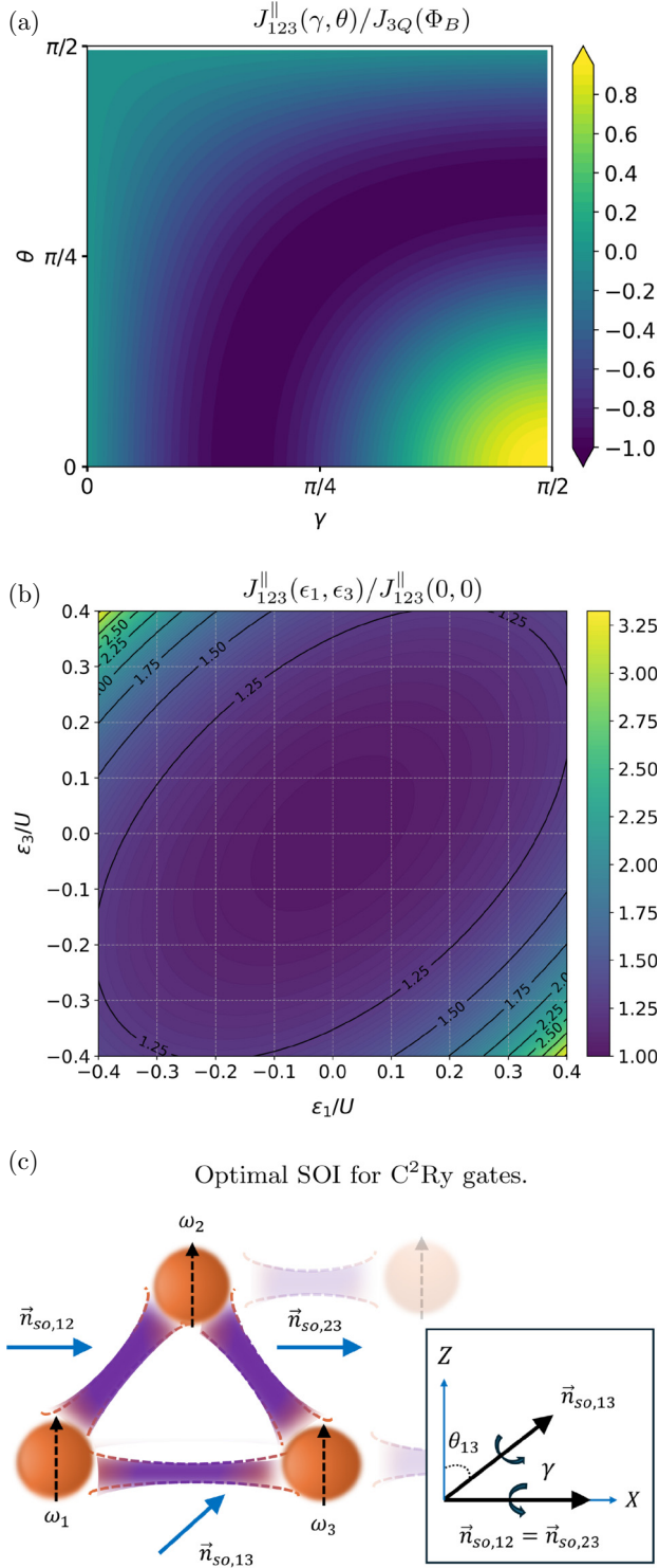
FIG. 4. Dependence of J_{123}^{\parallel} on SOI and QD energy detuning (a) The ratio J_{123}^{\parallel}/J_{3Q}(\Phi_B) for a symmetric system with (\gamma_{ij}, \theta_{ij}, \varphi_{ij}) = (\gamma, \theta, \varphi) . This ratio is independent of \varphi . (b) The ratio J_{123}^{\parallel}(\epsilon_1, \epsilon_3)/J_{123}^{\parallel}(0, 0) , where \epsilon_i are the dot energies. This ratio is independent of the SOI configuration. (c) Sketch of the SOI configuration considered in Eq. (44). The optimal configuration for the C^2Ry(\pi) gate is obtained at \theta_{13} = 0 and \gamma = \pi/2 .
