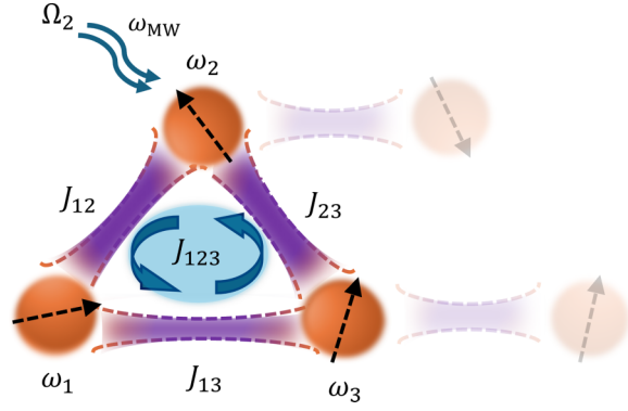
FIG. 1. Sketch of a three-qubit setup. We consider a triangular arrangement comprising three tunnel-coupled QDs each containing a single spin with frequency \omega_i . This system displays both nearest-neighbor exchange interactions J_{ij} and chiral anisotropic interactions J_{123} . The target qubit Q_2 of our controlled-controlled-rotation gate is driven by a microwave pulse with frequency \omega_{\text{MW}} and amplitude \Omega_2 .
