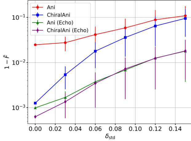
(a) Fast gate under quasi-static error
