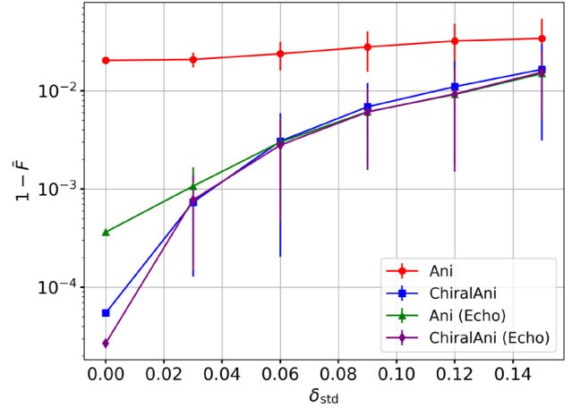
FIG. 6. Gate performance with noise. Numerical simulation with qubit frequencies \omega_1/2\pi = 4.2 GHz, \omega_2/2\pi = 4.5 GHz, and \omega_3/2\pi = 4.8 GHz. Exchange interactions are J_{12}/2\pi = J_{23}/2\pi = 20 (90) MHz and J_{13}/2\pi = 1.6 MHz for normal (fast) gates with gate time T_g = 100 (22.22) ns. The Ani gate follows the (0, 1) synchronization, with Rabi frequencies \Omega_2/2\pi \approx 5.16 (23.24) MHz, while the ChiralAni gate follows (0, 1, 1, 2), with \Omega_2/2\pi \approx 5.04 (22.68) MHz. The three-qubit interaction amplitude is J_{123}^{\parallel}/2\pi \approx 0.96 (4.34) MHz. We plot the gate infidelity under different noise sources for the anisotropic interaction (red), chiral anisotropic interaction (blue), and their Echo variants (green and purple, respectively). (a),(b) Gate infidelity against quasistatic error, where the noise is modeled as \delta_i(t) = \delta_i , drawn from a uniform distribution [-\delta_{\text{std}}, \delta_{\text{std}}] . (c),(d) Gate infidelity under high-frequency 1/f noise, modeled as a white noise with fluctuation \delta_{\text{std}} under infinite impulse response filter. Error bars represent \pm one standard deviation from the mean.
