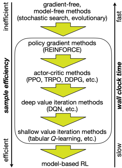
FIG. 11. Heuristic schematic of sample efficiency and runtime of some RL algorithms.
