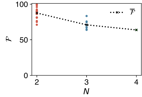
FIG. 5. Fidelity of entangled states as a function of qubit number N . Plotted are the state fidelities \mathcal{F} obtained from quantum state tomography of the Bell states ( N = 2 ), the state prepared by the circuit in Fig. 4(c) ( N = 3 ), and GHZ states ( N = 3, 4 ) in this work. A decrease in fidelity is observed as the number of qubits N increases. Colored dots represent the individual measurements, while black crosses denote the mean value.
