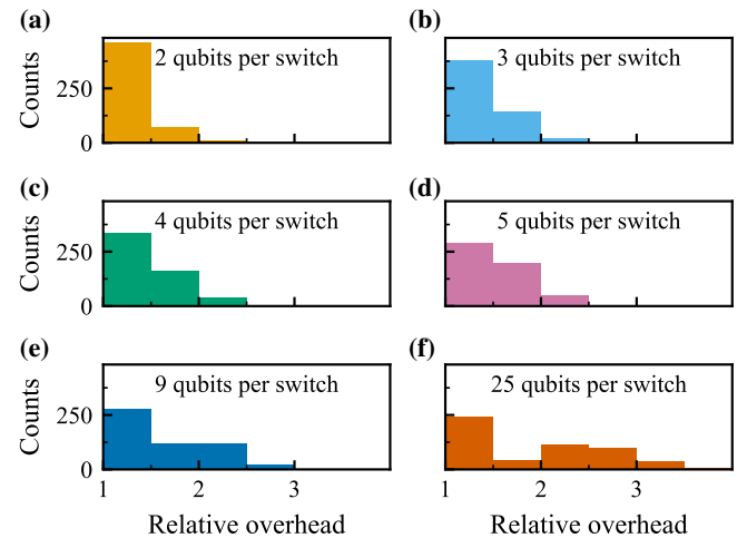
FIG. 16. Distribution of time-multiplexing overhead across switch sizes on a 5 \times 5 grid, for the quantum algorithms from MQT Bench shown in Fig. 14. The histograms show the relative overhead (the ratio of serialized to routed circuit duration) for different numbers of qubits per switch. The +n notation to the right in the bottom right histogram indicates n additional counts beyond the histogram limits.
