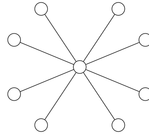
FIG. 1. The star graph on nine vertices, S_9 .
