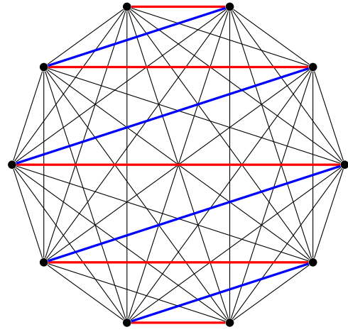
FIG. 4. Any cyclic permutation can be decomposed into two stages of transpositions. For example, a clockwise cycle of all vertices can be achieved by a global transposition between pairs of sites connected by blue edges followed by a global transposition for red edges. To perform an anticlockwise cycle, simply transpose along the red edges and then the blue edges.
