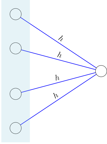
FIG. 8. Linear entangling rate between N leaves of the star graph and the center vertex. If the initial state is a product state of the N -qubit GHZ (Greenberger-Horne-Zeilinger) state \frac{1}{\sqrt{2}}(|00\dots 0\rangle + |11\dots 1\rangle) on the leaves, and |0\rangle on the center, then evolving for time \pi/N with interaction h = \frac{1}{4}(I - Z_{l_i}) \otimes (I - X_c) (i.e., the generator of a CNOT) on each edge results in a final (N + 1) -qubit GHZ state on all the vertices.
