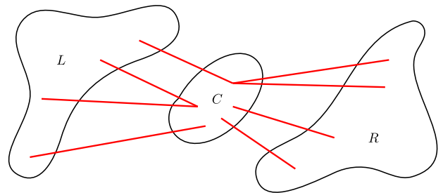
FIG. 2. A tripartition with vertex bottleneck C . Parts L, C, R contain N_L, N_C, N_R qubits, respectively. By the tripartite connectivity constraint, there are no edges between qubits in L and qubits in R .
