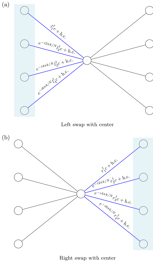
FIG. 7. Swapping the k th Fourier modes on the left and right sets of leaves. (a) Left swap with center. (b) Right swap with center.
