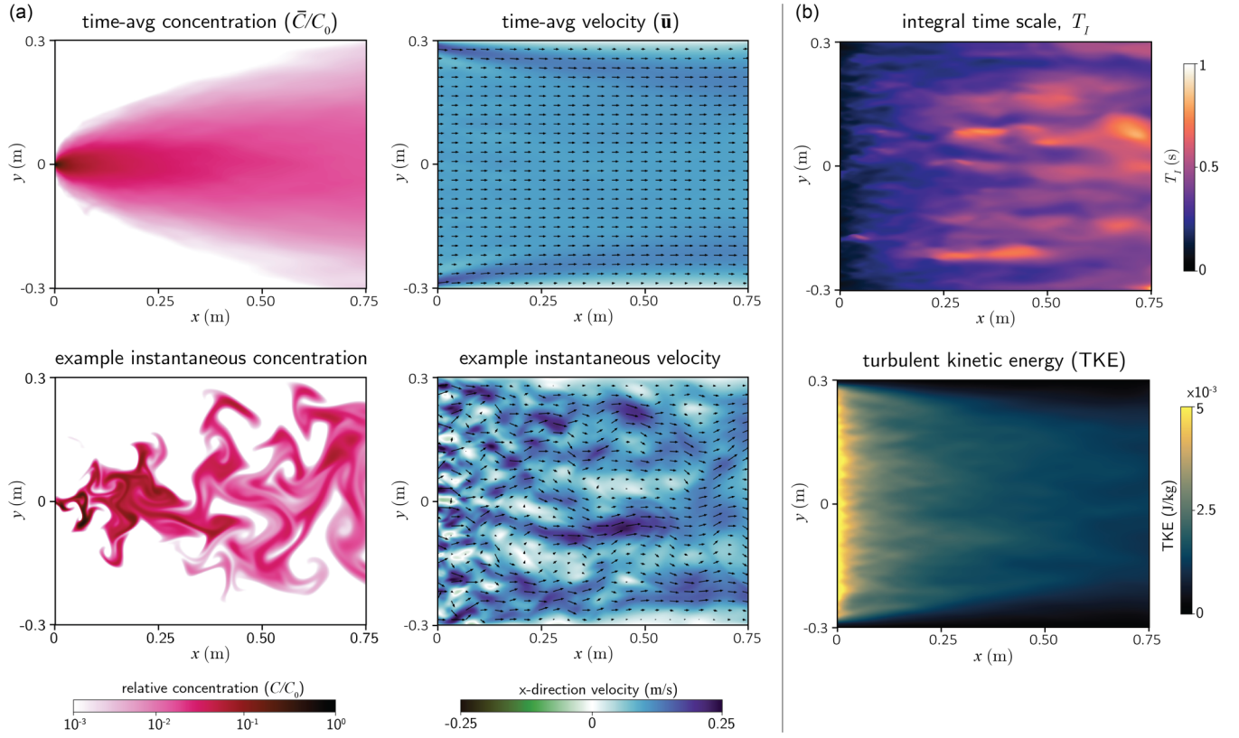
FIG. 9. Spatial distribution of properties computed for the computational fluid dynamics simulation, including (a) time-average (top) and instantaneous snapshots (bottom) of the concentration and velocity fields and (b) two time-averaged velocity field quantities: integral timescale and turbulent kinetic energy.
