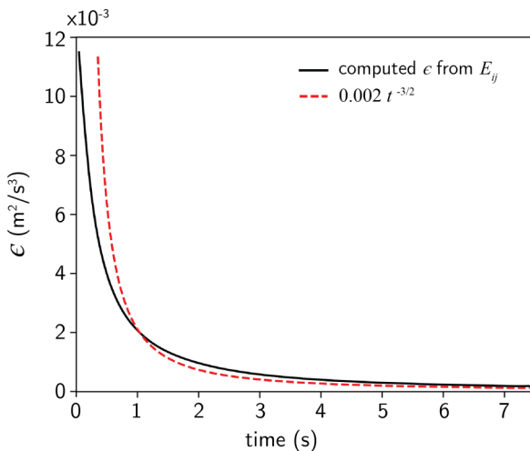
FIG. 11. Enstrophy dissipation rate demonstrating scaling approximately as t^{-3/2} .
