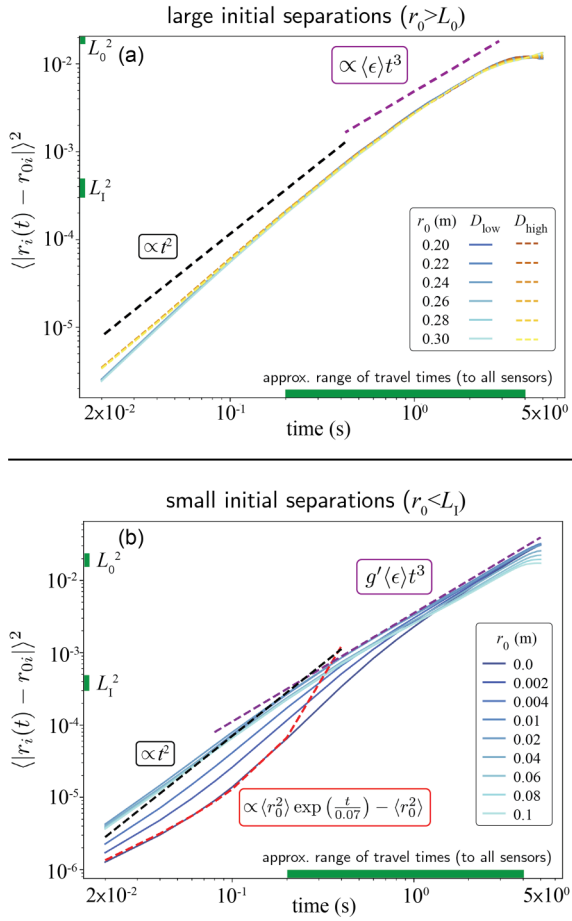
FIG. 10. Mean-squared particle pair separations computed from trajectory data.
