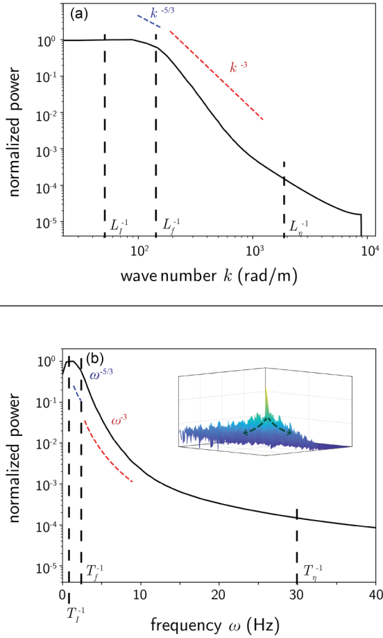
FIG. 6. Velocity spectrum for sensor at a downstream distance of 0.05 m (a) shown in the traditional fluid dynamics form as a log-log plot with wave number k on the x axis and (b) shown in a more sensory-relevant form that mimics the mapping matrix format as a semilog plot with frequency on the x axis. Red and blue dashed lines show expected power scaling in the inertial range. Relevant length (time) scales are shown as black dashed lines: integral scale is marked with subscript I , forcing scale with subscript f , and Kolmogorov scale with subscript \eta . A perspective plot of the frequency mapping function from Fig. 4(c) is inset in (b) to illustrate the component of frequency spreading.
