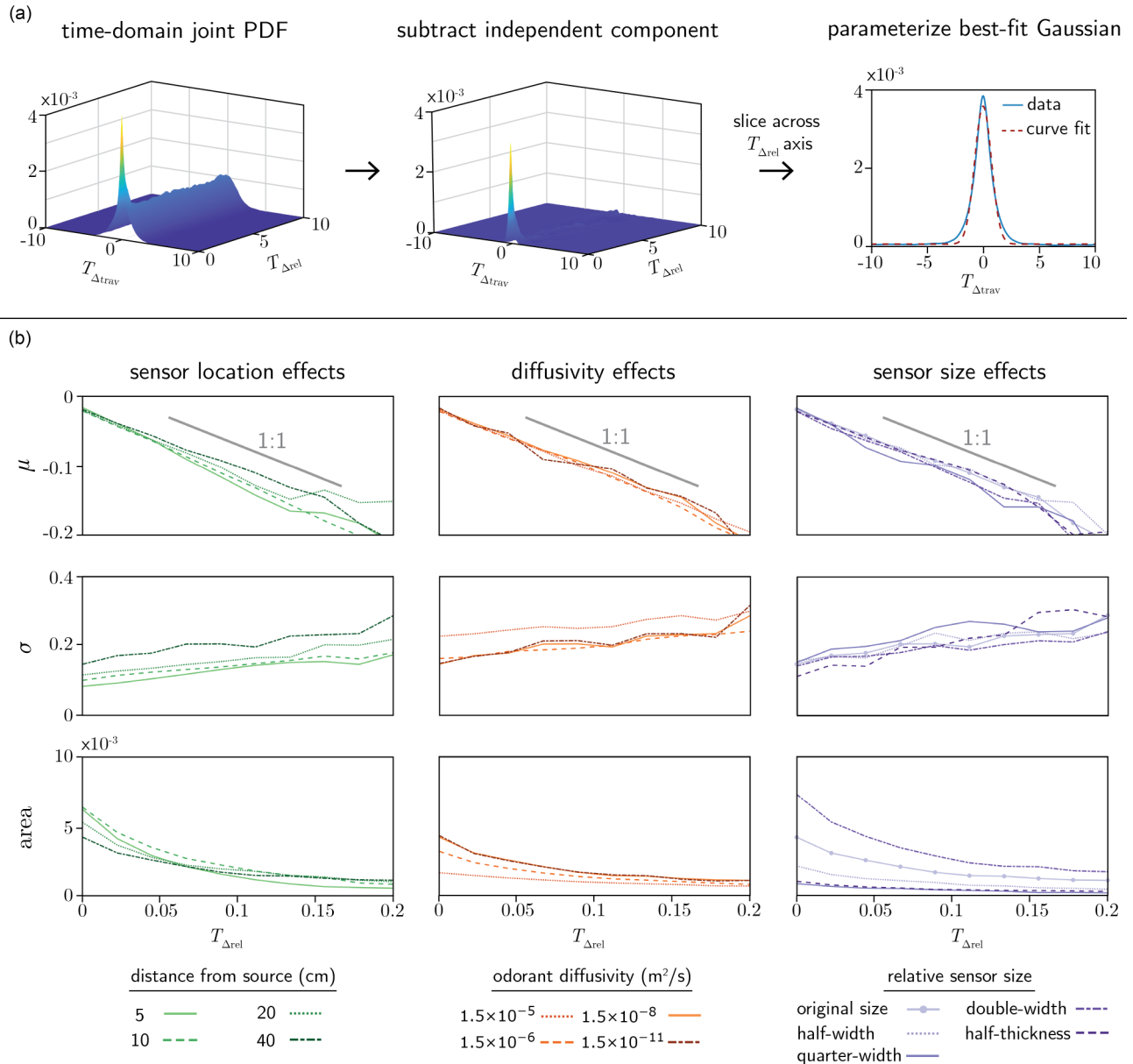
FIG. 8. Time-domain approach and results for parametrizing the correlated component of the frequency mapping function. (a) Analysis approach: First, we construct a time-domain plot of difference in travel time, T_{\Delta\text{trav}} , vs difference in release time, T_{\Delta\text{rel}} , for particle pairs. Next, the quantifiable independent component is subtracted, leaving a “spike” representing the correlated component, significant at small differences in release time. Finally, slices are taken along the T_{\Delta\text{rel}} axis and Gaussian functions are fit to each curve using an iterative approach to minimize the \chi^2 metric. (b) Resulting parameters characterizing a Gaussian fit to the correlated component of the time-domain mapping function for a range of small differences in release time. The top row shows the mean, \mu , the middle row the standard deviation, \sigma , and the third row the area of the best-fit Gaussian function (computed as \text{area} = A\sigma\sqrt{2\pi} , where A is the amplitude). The first column shows the effects of moving the sensor to different downstream distances with diffusivity held constant at 1.5 \times 10^{-5} \text{ m}^2/\text{s} and sensors at the original size (2 cm thickness with the width scaling as \sqrt{x_i/x_0} ). The second column measures effects from varying the odor diffusivity, at a location of 40 cm downstream and the original sensor size ( 0.087 \times 0.02 \text{ m} at this location). Because there is constant kinematic viscosity across cases, this can also be thought of as varying the Schmidt number ( Sc , a dimensionless number that quantifies the ratio of momentum diffusivity to mass diffusivity as Sc = \nu/D ), from Sc = 1 to Sc = 10^6 . Note that Sc of order unity represents typical air-borne odor conditions, while odors in water exhibit Sc on the order of 10^3 \text{m}^2/\text{s} , and a Sc of 10^6 is essentially a nondiffusive condition. The third column displays results of changing the sensor size, with diffusivity held constant at 1.5 \times 10^{-5} \text{ m}^2/\text{s} and sensor location at 40 cm downstream of the source.
