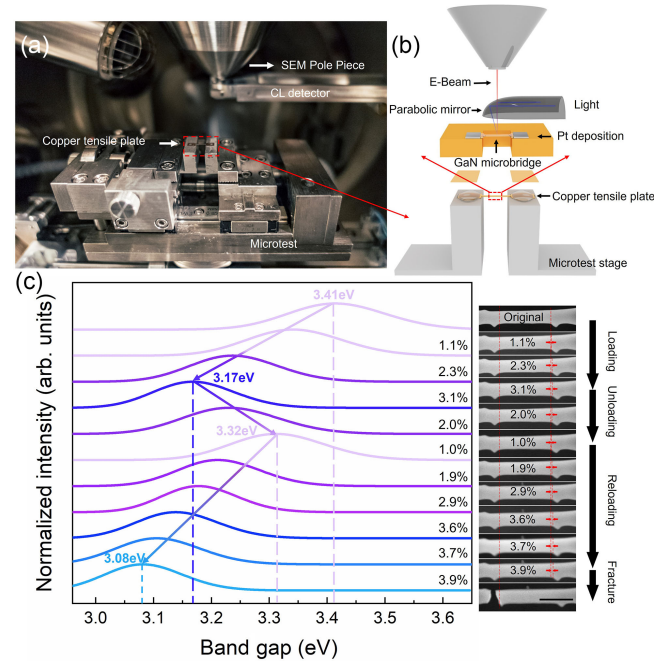
FIG. 2. in situ tension-CL analysis on band gap modulation during the GaN loading-unloading process. (a) The in situ tension-CL setup, including a microtest tensile stage and a CL detector installed in SEM. (b) The schematic of the measurement setup. The GaN microbridge was fixed on a copper tensile plate which is strained by the tensile stage. (c) The normalized CL spectra shift from invisible to the visible range during the loading-unloading processes, and the corresponding SEM images during loading-unloading processes. Transparent spectra are in the invisible range. Scale bar: 1 \mu\text{m} .
