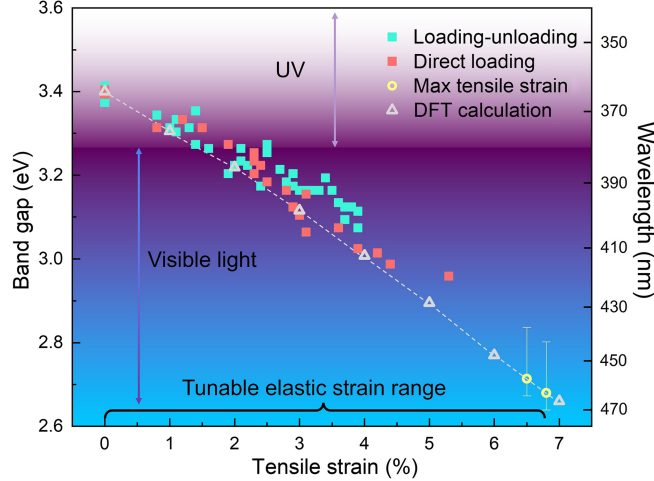
FIG. 4. Summary of the in situ CL band gap measurements along with the DFT calculation for [0001]-oriented GaN microbridges upon tensile straining experiments (both loading-unloading and direct tensile loading experiments, respectively). Solid blue squares show the loading-unloading in situ CL emission results; solid red squares show the direct tensile loading in situ CL emission results; hollow gray triangles refer the DFT calculation results, which agree well with the experimental trend; hollow yellow circles show the maximum tensile strains experimentally achieved in our experiments, with the corresponding band gap and wavelength values estimated by DFT calculations (error bars determined by overall experiment or DFT variances).
