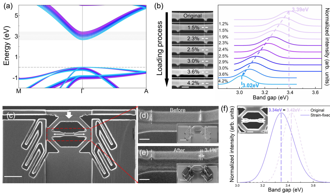
FIG. 3. Deep strain engineering-induced band gap modulation and strain-fixed GaN device. (a) The band structure evolution of GaN as a function of tensile strain from 0% (dark violet) to 7% (light blue) was calculated by DFT. (b) The SEM images of a GaN microbridge during the loading process, and the corresponding normalized CL spectra shift from “invisible UV” ( \sim 3.4 eV) to the “visible blue light” ( \sim 3 eV) regime during the tensile loading process. Initial transparent violet spectra refer to the invisible light regime. Scale bar: 500 nm. (c) The design and working principle of the strain-fixed GaN device with a push-to-pull structure. Scale bar: 2 \mu\text{m} . (d) and (e) The strain-fixed GaN device with 3.1% uniaxial tensile strain. Scale bar: 500 nm. Inset: The morphology of a strain-fixed GaN device before and after strain maintenance. Scale bar: 2 \mu\text{m} . (f) CL characterization of a strain-fixed GaN microbridge with band gap shift from 3.42 to 3.34 eV. Inset: the area where we detected CL characterization. Scale bar: 1 \mu\text{m} .
