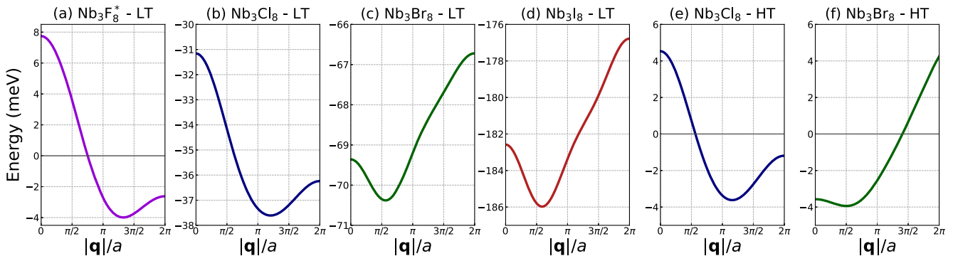
FIG. 24. Energies of the exchange interactions as a function of \mathbf{q} for (a)–(d) all LT ( R\bar{3}m ) \text{Nb}_3\text{X}_8 compounds and (e)–(f) HT ( P\bar{3}m1 ) \text{Nb}_3\text{Cl}_8 and \text{Nb}_3\text{Br}_8 .
