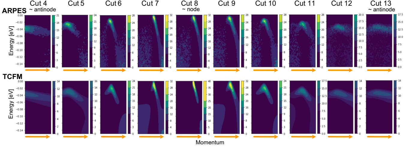
FIG. 2. Comparison between \tilde{I}_{\text{ARPES}}(\mathbf{k}, \omega) and \tilde{I}_{\text{TCFM}}(\mathbf{k}, \omega) . Orange arrows denote the momentum cuts indicated in Fig. 1(a).
