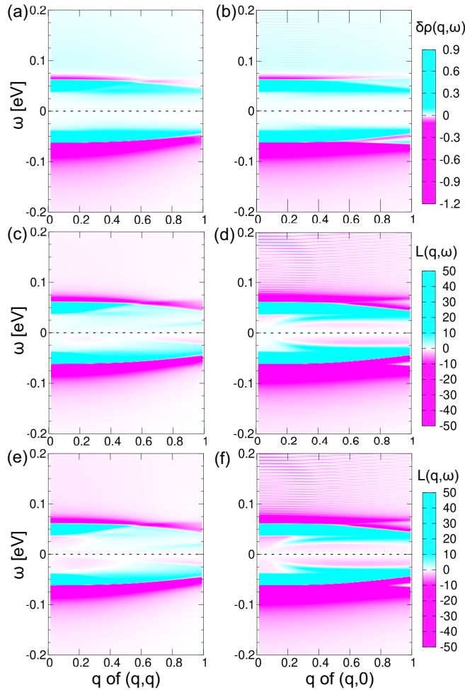
FIG. 15. High-energy structure of (a), (b) \delta\rho(\mathbf{q}, \omega) , (c), (d) L(\mathbf{q}, \omega) along (0,0)-(1,1) and (0,0)-(1,0) , calculated with the Hamiltonian, Eq. (11), and (e), (f) the same as (c), (d) but without the Gaussian contribution, Eq. (A47), around \mathbf{q} \simeq \mathbf{0} . Plots for (0,0)-(\pi,\pi) and (0,0)-(2\pi,0) are shown in Fig. S6 of Supplemental Material [103].
