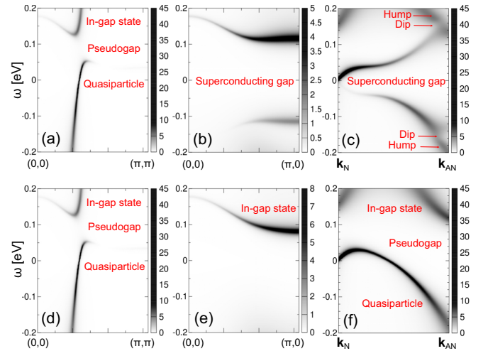
FIG. 21. (a)–(c) The same as Fig. 20 but with \Sigma_{\text{bg}} = 0 . (d)–(f) Normal-state dispersions corresponding to (a)–(c), calculated with \Sigma_{\text{bg}} = 0 and D_{c,0} = D_{d,0} = 0 .
