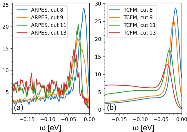
FIG. 4. Energy distribution curves obtained by (a) ARPES ( \tilde{I}_{\text{ARPES}} ) and (b) the TCFM ( \tilde{I}_{\text{TCFM}} ) at \mathbf{k} = \mathbf{k}_{\text{max}} in each cut.
