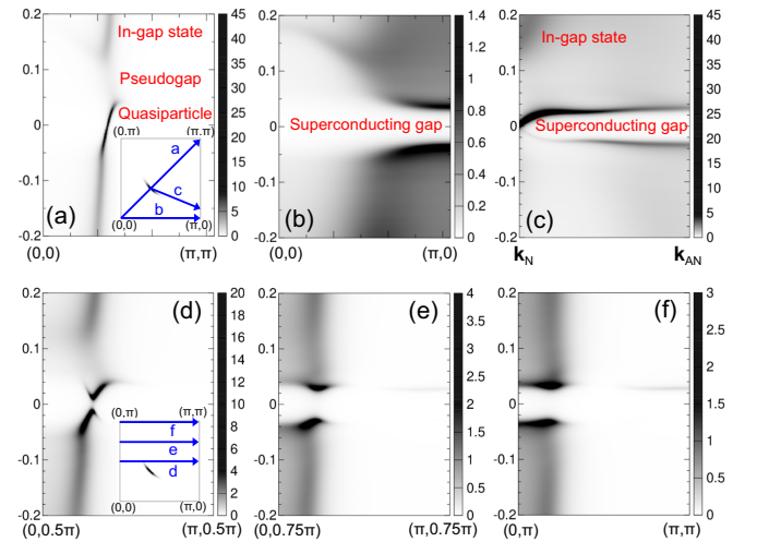
FIG. 3. A(\mathbf{k}, \omega) calculated for the TCFM along (a) (0,0) - (\pi,\pi) , (b) (0,0) - (\pi,0) , (c) \mathbf{k}_N - \mathbf{k}_{AN} , (d) (0,0.5\pi) - (\pi,0.5\pi) , (e) (0,0.75\pi) - (\pi,0.75\pi) , and (f) (0,\pi) - (\pi,\pi) . Insets in (a) and (d) illustrate the momentum cuts used in (a)–(f).
