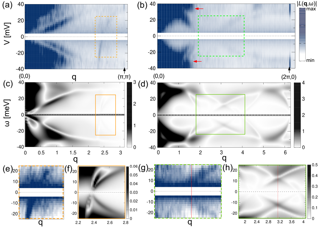
FIG. 10. Comparison of |L(\mathbf{q}, \omega)| between (a), (b) the experiment and (c), (d) the TCFM along the (0,0) - (\pi, \pi) and (0,0) - (2\pi, 0) lines. Enlarged structures are shown in (e)–(h) for areas enclosed by rectangles in (a), (c), (b), and (d), respectively, for the same purpose as in Fig. 9. Red arrows in (b) indicate the mirror signals of \mathbf{q}_5 discussed in Appendix C 1. Red vertical lines in (g) and (h) denote (\pi, 0) . In (a), (b), (e), and (g), it is difficult to obtain accurate experimental data for small |V| because both (dI/dV) and (I/V) in L = (V/I)(dI/dV) are not large enough compared to noise.
