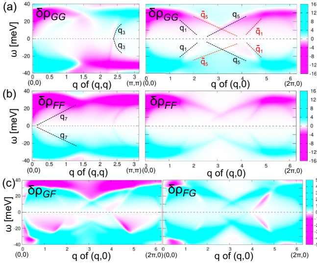
FIG. 24. Each component, Eq. (A35), contributing to \delta\rho(\mathbf{q}, \omega) along the (0,0)-(\pi,\pi) and (0,0)-(2\pi,0) lines. Note that \delta\rho_{GF}(\mathbf{q}, \omega) = \delta\rho_{FG}(\mathbf{q}, \omega) \equiv 0 along (0,0)-(\pi,\pi) .
