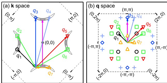
FIG. 8. Schematic of the relation between (a) the \mathbf{k} -space structure of the spectral function and (b) the QPI signals in the \mathbf{q} space. \mathbf{q}_i 's ( i = 1, \dots, 7 ) denote momenta connecting the tips of the banana-shaped spectral intensity. The vertical magenta arrows passing through (0, 0) represent the new branch observed nearby \mathbf{q}_3 .
