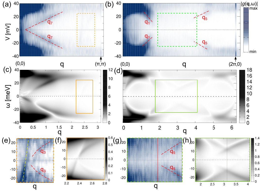
FIG. 9. Comparison of |g(\mathbf{q}, \omega)| between (a), (b) the experiments and (c), (d) the TCFM along the (0,0)-(\pi, \pi) and (0,0)-(2\pi, 0) lines. V_{\text{set}} = -0.1 V. Enlarged structures are shown in (e)–(h) for areas enclosed by rectangles in (a), (c), (b), and (d), respectively, with different gray scales for better visibility of the dispersions. In (e) and (f), \mathbf{q}_3 is visible as electron-hole symmetric dispersions while an additional electron-hole asymmetric dispersion [denoted by yellow dashed line in (e)] is seen on the smaller- \mathbf{q} side of \mathbf{q}_3 . In (g) and (h), electron-hole symmetric \mathbf{q}_1 and \mathbf{q}_5 are visible in small and large \mathbf{q} regions, respectively. Red vertical lines denote (\pi, 0) .
