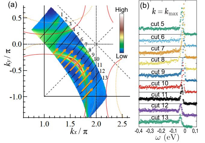
FIG. 1. ARPES experimental result for the optimally doped Bi2212 [86]. (a) Momentum-space map of the low-energy spectral intensity. The red solid (orange dashed) curves denote the normal-state Fermi surface (shadow band), black solid lines denote the momentum cuts along which the dispersion is measured, and the orange arrows on them denote the data used in the fitting in this study. (b) The EDCs at \mathbf{k} = \mathbf{k}_{\text{max}} along the cuts 5–13.
