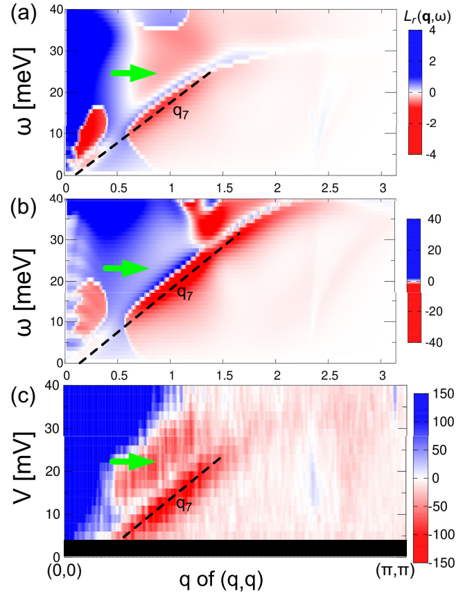
FIG. 13. Relative-sign structure L_r(\mathbf{q}, \omega > 0) along (0,0) - (\pi, \pi) , obtained by (a) the TCFM, (b) the single-component Hamiltonian, Eq. (11), and (c) the experiment. The light green arrows indicate the area discussed in the main text. Note that the dashed line ( \mathbf{q}_7 dispersion) is drawn by following the octet model illustrated in Fig. 8. Black region in (c) indicates an energy range where accurate data are difficult to obtain because both (dI/dV) and (I/V) in L = (V/I)(dI/dV) are not large enough compared to noise.
