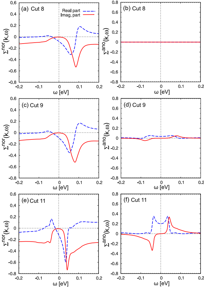
FIG. 19. The \omega dependence of the TCFM self-energy at \mathbf{k} = \mathbf{k}_{\max} in the cuts 8 [(a), (b)], 9 [(c), (d)], and 11 [(e), (f)], corresponding to the spectra in Fig. 4(b). Note that the corresponding self-energy for the cut 13 is presented in Figs. 5(c) and 5(d), to which the scale of the ordinate is adjusted.
