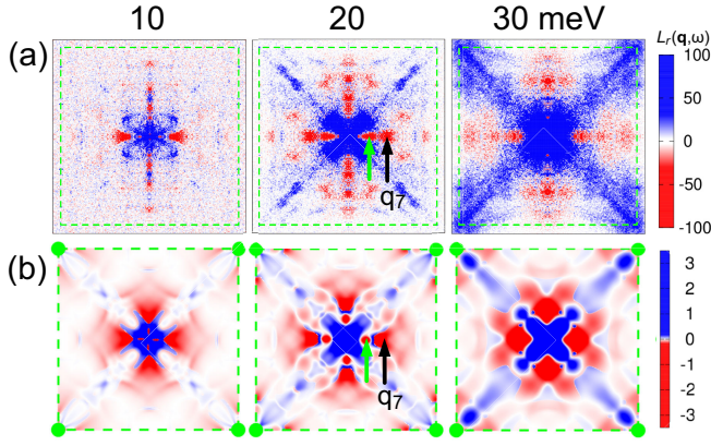
FIG. 26. Comparison of \mathbf{q} -space maps of L_r between (a) the experiment and (b) the TCFM. Light green circles in (b) denote the Bragg points, (\pm 2\pi, 0) and (0, \pm 2\pi) . Light green arrows denote the signal discussed in Sec. V C 2. Black arrows denote the \mathbf{q}_7 spots.
