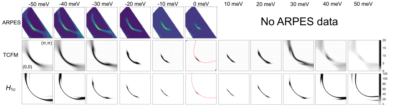
FIG. 6. Comparison between momentum-space maps of ARPES spectra (top panels) and of A(\mathbf{k}, \omega) calculated for the TCFM (middle panels) and the single-component Hamiltonian [Eq. (11)] (bottom panels) at various energies. Red dashed curves at 0 meV in the theoretical results depict the Fermi surface of the normal state ( D_c = D_d = 0 ). In the TCFM result, we also plot tiny normal-state Luttinger surfaces (zeros of the Green's function) by blue solid curves around (\pi, 0) and (0, \pi) .
