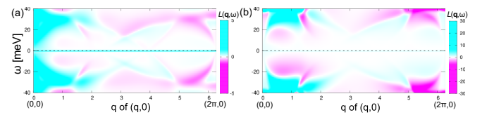
FIG. 25. Sign structure of L(\mathbf{q}, \omega) along (0,0)-(2\pi,0) calculated with (a) the TCFM and (b) the single-component Hamiltonian, Eq. (11).
