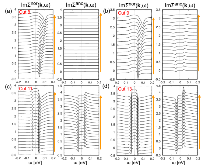
FIG. 18. The \omega dependence of \text{Im}\Sigma^{\text{nor}} and \text{Im}\Sigma^{\text{ano}} along the cuts 8, 9, 11, and 13 [(a)–(d), respectively]. Each curve is shifted vertically by 0.2 for clarity. The orange arrows correspond to those in Fig. 1(a).
