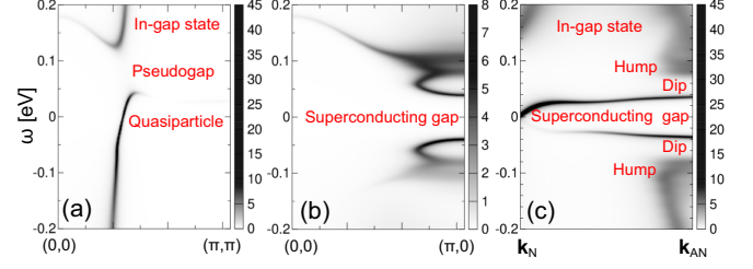
FIG. 20. A(\mathbf{k}, \omega) calculated for the TCFM along (a) (0, 0) - (\pi, \pi) , (b) (0, 0) - (\pi, 0) , and (c) \mathbf{k}_N - \mathbf{k}_{AN} , with setting \text{Im } \Sigma_{\text{bg}} = 0 .
