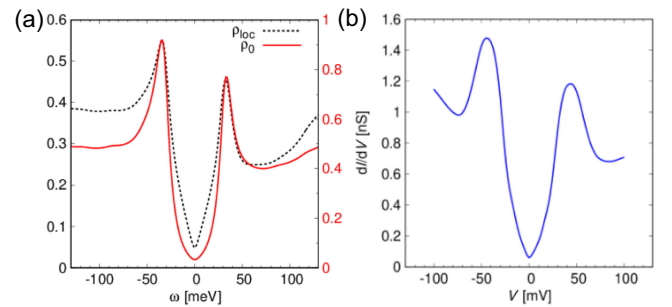
FIG. 7. Comparison between (a) the calculated DOS and (b) the STM experimental result of dI/dV . In (a), \rho_{\text{loc}} is the DOS of the TCFM, defined by Eq. (A13), while \rho_0 is the DOS projected onto the surface (and hence more suitable for the comparison with the STM experimental result) as defined by Eq. (A26).
