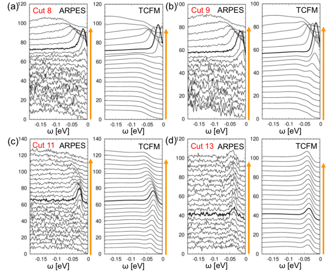
FIG. 17. (a)–(d) Comparison of the EDCs along the cuts 8, 9, 11, and 13 between ARPES ( \tilde{I}_{\text{ARPES}} ) and the TCFM ( \tilde{I}_{\text{TCFM}} ). Each curve is shifted vertically by 5 for clarity. Orange arrows correspond to those in Fig. 1 and bold curves denote the EDC closest to \mathbf{k}_{\text{max}} .
