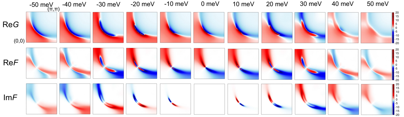
FIG. 22. Isoenergy momentum-space maps of \text{Re}G , \text{Re}F , and \text{Im}F . For \text{Im}G , see A(\mathbf{k}, \omega) = -(1/\pi) \text{Im}G in Fig. 6 lower panels.
