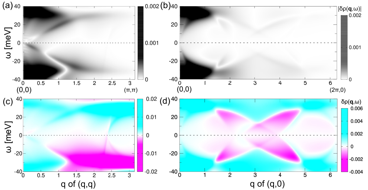
FIG. 11. (a), (b) |\delta\rho(\mathbf{q}, \omega)| calculated with the TCFM for r_0 = r_{0SC} = 0.4a along the (0,0) - (\pi, \pi) and (0,0) - (2\pi, 0) lines. (c), (d) Corresponding \delta\rho (with signs) calculated with the TCFM for \mathbf{q} -independent \hat{V}_{imp} .
