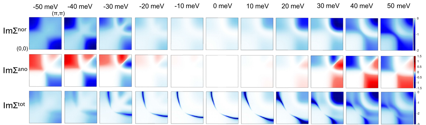
FIG. 23. Isoenergy momentum-space maps of \text{Im} \Sigma^{\text{nor}} , \text{Im} \Sigma^{\text{tot}} , and \text{Im} \Sigma^{\text{ano}} .
