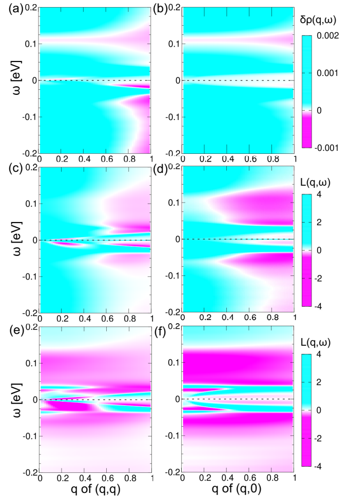
FIG. 14. High-energy structure of (a), (b) \delta\rho(\mathbf{q},\omega) , (c), (d) L(\mathbf{q},\omega) along (0,0)-(1,1) [(a), (c)] and (0,0)-(1,0) [(b), (d)], calculated with the TCFM, and (e), (f) the same as (c), (d) but without the Gaussian contribution, Eq. (A47), around \mathbf{q} \approx \mathbf{0} . Plots for full ranges, (0,0)-(\pi,\pi) and (0,0)-(2\pi,0) , are shown in Fig. S5 of Supplemental Material [103].
