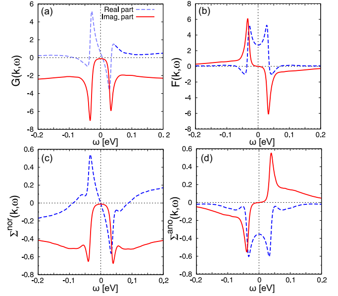
FIG. 5. Real (blue dashed curve) and imaginary (red solid curve) parts of (a) G , (b) F , (c) \Sigma^{\text{nor}} , and (d) \Sigma^{\text{ano}} at the antinode, \mathbf{k} = \mathbf{k}_{\text{AN}} = (\pi, 0.14\pi) , calculated by the fitted TCFM.
