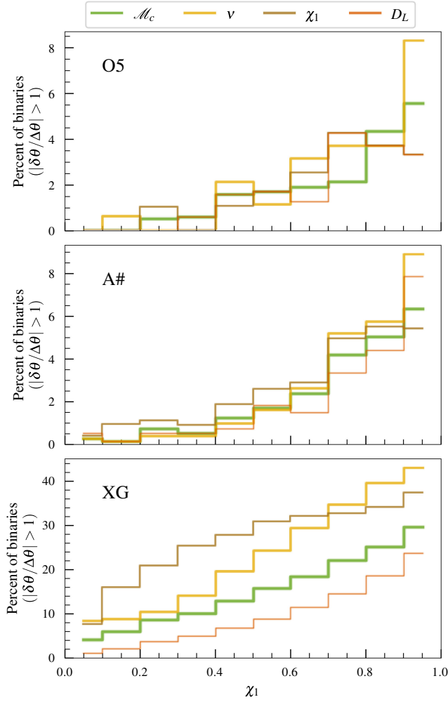
FIG. 8. Percentage of binaries in each \chi_1 bin with |\delta\theta/\Delta\theta| > 1 for different parameters. The top, middle, and bottom panels show the percentages for the O5 , A# , and XG networks, respectively.
