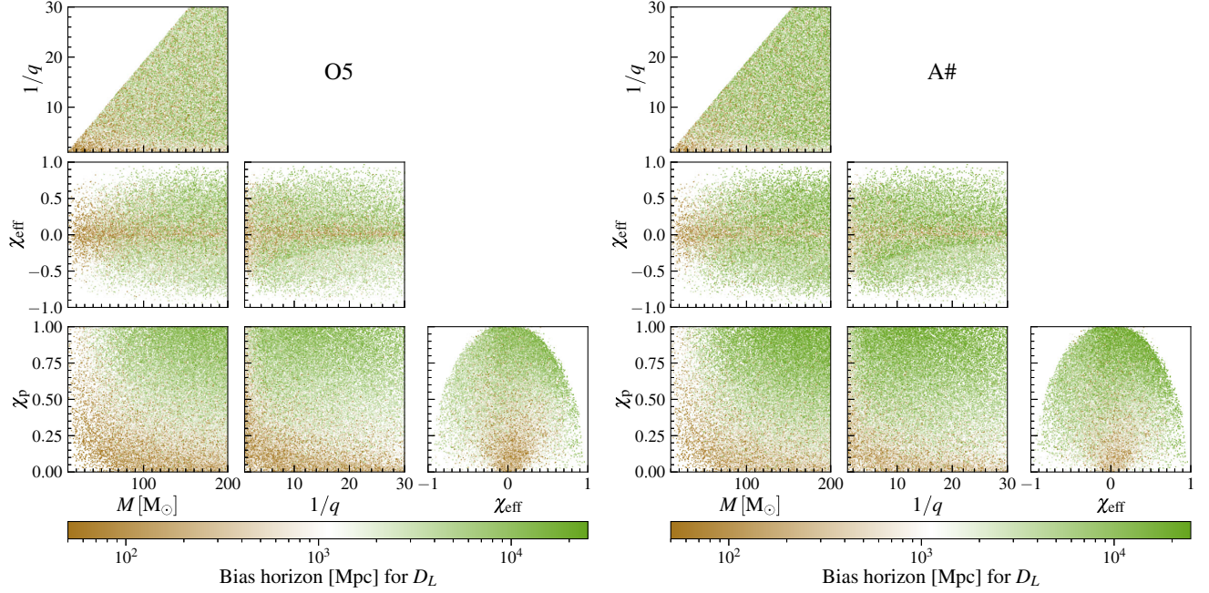
FIG. 10. Distribution of the 50,000 binaries in the parameter space represented in Fig. 9, with the color scale showing the distance to which the D_L parameter is biased ( \delta D_L / \Delta D_L \geq 1 ) for the O5 (left) and A# (right) networks. Systematic biases become less important if a binary is at a larger distance since measurement precision decreases with distance. Therefore, a large bias horizon signifies that a given parameter ( D_L in this case) is measured well enough for systematic biases to be important even at such large distances. Notice that the binaries are biased up to a greater distance in the A# network compared to the O5 network due to its greater sensitivity and the resultant improvement in measurement precision.
