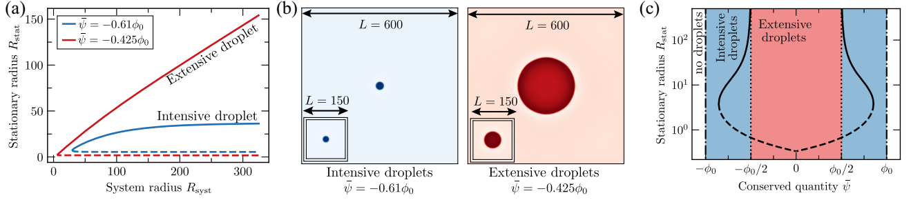
FIG. 3. Critical transition between intensive (blue) and extensive (red) active droplets. (a) There are two classes of stationary solutions, depending on the value of the conserved quantity \tilde{\psi} . The stationary droplet size R_{\text{stat}} either increases with system size R_{\text{syst}} (red line) or saturates for large values of R_{\text{syst}} (blue line). We refer to these cases as extensive (red) and intensive (blue) active droplets. Stable branches are depicted by solid lines and unstable branches are dashed. (b) Stationary concentration fields (component A) corresponding to each class [color code as in (a)] are shown for large ( L = 600 ) and small systems ( L = 150 ). They are obtained from numerically solving Eqs. (3). Note that the large red droplet would undergo a shape instability once the spherical droplet shape is perturbed. (c) Dependence of the stable (solid line) and unstable (dashed line) stationary radius, R_{\text{stat}} , on the conserved quantity \tilde{\psi} for \alpha = 0 in an infinite system. The stable branch (solid line) diverges following a power law, R_{\text{stat}} \propto |\tilde{\psi} - \tilde{\psi}_{\text{crit}}^{\pm}|^{-1} , for \tilde{\psi} \gtrless \tilde{\psi}_{\text{crit}}^{\pm} , supporting that the transition controlled by the conserved quantity is critical. Note, these stationary radii have been computed for a finite value of the surface tension, thereby leading to a gap between the onset of stationary droplets (where the stable and unstable branch converge) and the binodal (dash-dotted line). Furthermore, we show the \tilde{\psi} value for the critical transition between (dotted line). Because of our choice of the phase diagram, the system is symmetric around \tilde{\psi} = 0 . Note that \tilde{\psi} < 0 corresponds to an A-rich droplet surrounded by an S-rich phase, while \tilde{\psi} > 0 corresponds to an S-rich droplet surrounded by an A-rich phase. We color coded the regions where no droplets (white), intensive active droplet (blue), and extensive active droplet (red) exists for a system for large K , such that stationary radii get large and Laplace pressure effects can be neglected. Details on the analytical calculation of R_{\text{stat}} are given in Appendix E, and parameter choices for all three panels are discussed in Appendix H. All length scales in this figure are given in the terms of the interface width.
