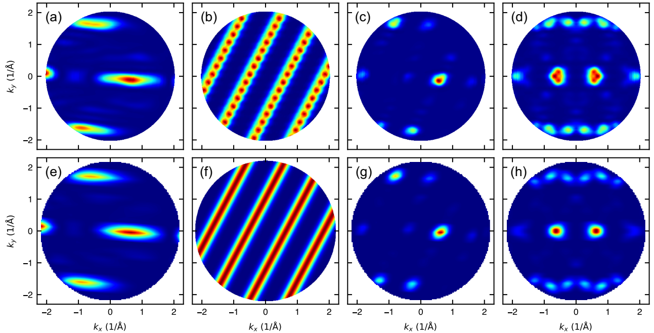
FIG. 13. (a)–(d) Decomposition of the photoemission intensity of exciton S_1 from the ab initio expOT simulation into individual contributions. (a) Absolute square of the Fourier-transformed LUMO band wave functions |\mathcal{F}[\xi_{c_1q}](\mathbf{q} + \mathbf{G})|^2 . (b) Absolute square of the BSE eigenvector |X_{v_1c_1q}^m|^2 from Eq. (C23). Panel (d) shows the symmetrized photoemission intensity shown in panel (c). (e)–(h) Analogous to (a)–(d) but for the exciton model following Eq. (C21). (e) Absolute square of a Fourier-transformed LUMO of a gas-phase molecule |\mathcal{F}[\xi_L](\mathbf{k})|^2 . (f) Factor |\sum_{\mathbf{R}}^{\text{crystal}} \alpha(\mathbf{R}) e^{i\beta(\mathbf{R})} e^{-ik\cdot\mathbf{R}}|^2 arising from the envelope function and model phase factor. Panel (g) and (h) show the photoemission intensity I_{\text{model}}(\mathbf{k}) [product of panels (e) and (f)], before and after symmetrization, respectively.
