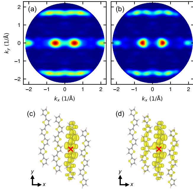
FIG. 12. (a) Simulated momentum map for S_1 of the tetramer and (b) S_4 of the tetramer. Panels (c) and (d) show the corresponding fixed-hole electron density |\Psi(\mathbf{r}_e, \mathbf{r}_h = \text{fixed})|^2 (isosurface at 0.5% of maximum value). The hole has been fixed 0.5 Å above a carbon atom connecting the central thiophene rings, as indicated by the red crosses.
