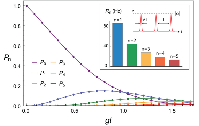
FIG. 4. Detection probabilities for the first few accessible states when FBS system is stimulated with a single photon, plotted over gt ( g as the coupling rate, t as time). Optical loss is taken as \gamma = g . Solid lines correspond to Eq. (20) and circles correspond to simulations that include mechanical dephasing and loss. Inset: Heralding rates for Fock states n = 1-5 |n\rangle_{\text{ph}} in Hz with pulsed source amplitude |\alpha| = 0.2 and duty cycle T = 2/g .
