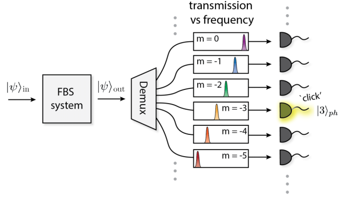
FIG. 3. Scheme describing quantum state synthesis in a forward Brillouin scattering system. The entangled state, |\psi\rangle_{\text{out}} , goes through a demultiplexer, filtering by frequency into different transmission lines to an array of single-photon detectors. The detection event (shown by the yellow highlight) projects the phonon into a Fock state.
