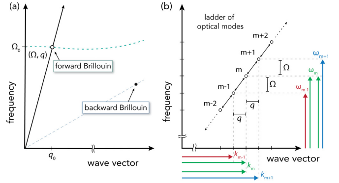
FIG. 2. Phase-matching conditions for intramodal forward Brillouin scattering in a resonator. (a) Acoustic dispersion, with the discrete forward Brillouin active mode shown as a white circle, where the mechanical frequency is approximately equal to the cut-off frequency, i.e., \Omega \cong \Omega_0 . A backward Brillouin active mode is shown as a black dot for comparison. (b) Optical dispersion, where the phonon frequency and wave vector resonantly couple adjacent discrete optical modes.
