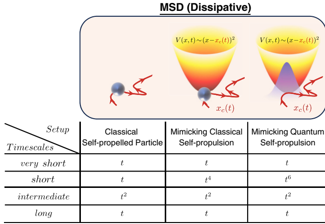
FIG. 1. Schematics and dynamics of dissipative quantum and classical overdamped active systems. (Left) Classical self-propelled particle (blue) with trajectory (red) and corresponding characteristic scaling of the MSD of an ensemble of self-propelled particles. (Center) Displacing a passive classical particle with a moving harmonic trapping potential (red to yellow paraboloid) mimics self-propulsion. (Right) Replacing the trapped classical particle by a quantum particle (wave function in blue) enables mimicking of quantum self-propulsion.
