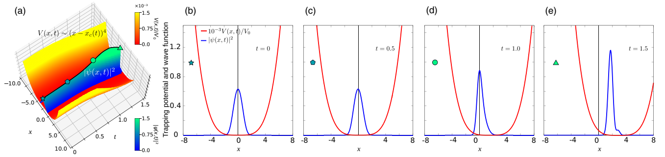
FIG. 4. Transient localization of the wave function. (a) Time evolution of the confining potential V(x, t) and the wave-function profile \langle \psi_t | \psi_t \rangle \equiv |\psi(x, t)|^2 , shown using red-yellow and blue-green color maps, respectively, for D = 1 , \tau = 1 , q = 4 . In the final state, the peak of the profile (shown with the black line) increases in height compared to the initial state, indicating stronger localization. (b)–(e) Potential (red) and wave-function profiles (blue) at different time instants t = 0, 0.5, 1.0 , and 1.5 , respectively. The time instants marked by different symbols in (a) correspond to those in (b)–(e).
