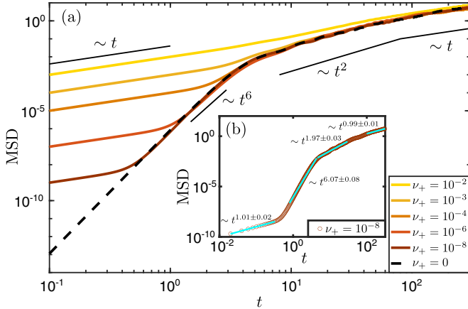
FIG. 2. MSD of a dissipative quantum-active particle. (a) MSD at various timescales for D = 0.01 , \tau = 10 , and \nu_- = 10^{-2} . (b) Fits of the MSD (cyan solid lines) for \nu_+ = 10^{-8} indicating the scaling behavior presented in Fig. 1 for a quantum-active particle. Uncertainties represent the standard deviation across 500 simulations and do not account for possible systematic numerical uncertainties.
