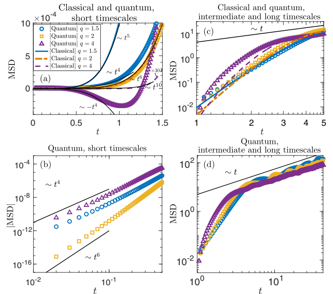
FIG. 5. MSD of a nondissipative quantum-active particle. (a) MSD at short timescales for D = 1 and \tau = 10 reveals quantum-active scaling being in general different from classical. (b) Log-log plot of the absolute values of MSD indicates \sim t^4 scaling for q \neq 2 and \sim t^6 for q = 2 . (c), (d) Crossover to the diffusive regime at long timescales for D = 1 and \tau = 1 . (a), (c) Comparison of quantum and classical active MSD. In all panels, an average is taken over 500 stochastic trajectories for each q considered.
