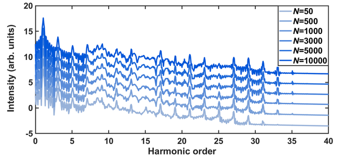
FIG. 5. Numerical convergence of HHG spectra for different average photon numbers N while keeping the effective field amplitude |E| = \sqrt{2\omega_l N / \epsilon_0 V} fixed. Spectra are vertically offset for clarity.
