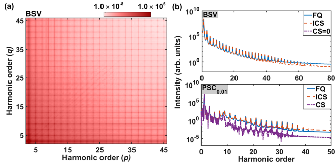
FIG. 4. (a) Cross-correlation C_{qp} between harmonic modes (q, p) for BSV light calculated via Husimi-distribution-based methods. (b) Comparison of the HHG spectra obtained from the FQ theory and Husimi-distribution-based methods for BSV light and PSC light with \chi = 0.01 , where ICS and CS denote incoherent summation and coherent summation of semiclassical spectra, respectively.
