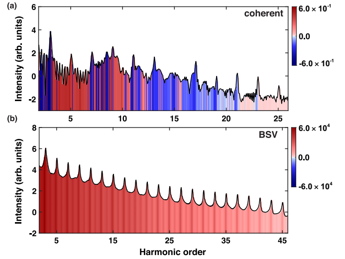
FIG. 2. Expectation value of the normally ordered variance of the number operator for each harmonic mode under (a) coherent light and (b) BSV light. Positive, negative, and zero values correspond to super-Poissonian, sub-Poissonian, and Poissonian statistics, respectively.
