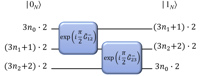
FIG. 1. Application of the logical X gate on a qutrit ( d = 3 ) encoded in a three-mode rotation-symmetric bosonic code of order N = 2 . Each of the lines indicates a single bosonic mode.
