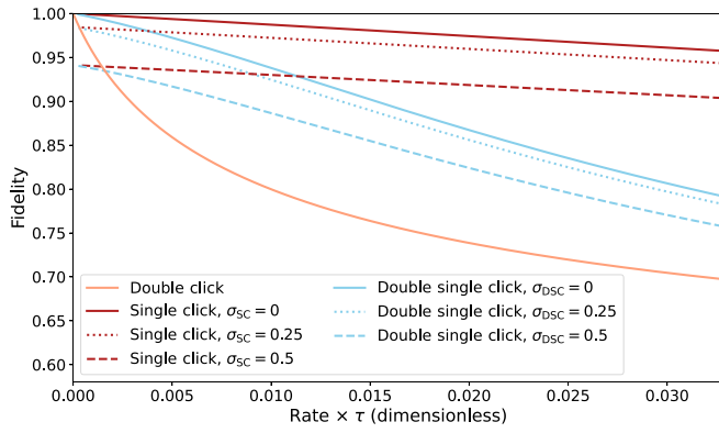
FIG. 2. Trade-offs between fidelity and rate for the three RSP protocols: DC (peach), SC (red), and DSC (blue). Shown for \sigma_{sc}, \sigma_{dsc} \in \{0 \text{ (solid)}, 0.25 \text{ (dotted)}, 0.5 \text{ (dashed)}\} . This analysis assumes a server efficiency of \eta_s = 0.091 , including a detector efficiency of 0.7. The values shown are for |\alpha|^2 \lesssim 3 (DC), |\alpha|^2 \lesssim 0.3 (SC), |\alpha|^2 \lesssim 1.2 (DSC).
