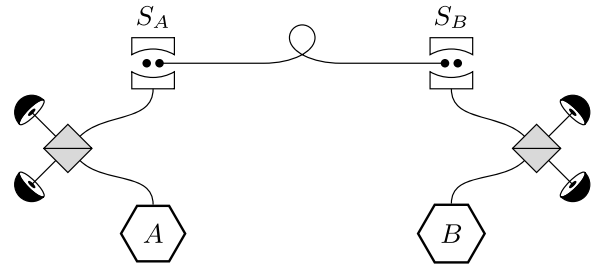
FIG. 5. Schematic drawing of the repeater QKD protocol between two clients A and B . The untrusted third party has prepared a long-distance entangled pair between nodes S_A and S_B . Client A ( B ) remotely prepares a new qubit of the form |+\theta\rangle on node S_A ( S_B ). Once remote state preparation succeeds for client A ( B ), a local Bell state measurement is performed between the two qubits at node S_A ( S_B ).
