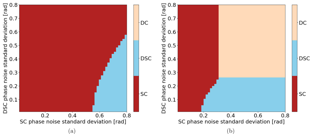
FIG. 8. Optimal RSP protocol—DC, DSC, or SC—giving the highest fidelity for target rate R\tau = 0.01 , across varying phase noise \sigma_{SC} and \sigma_{DSC} . Alternative values for Fig. 4(c). (a) \eta_S = 0.07 and (b) \eta_S = 0.35 .
