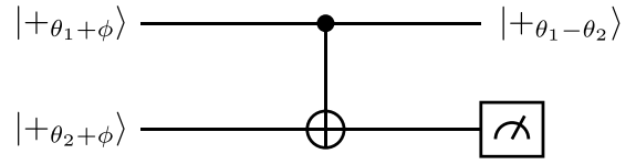
FIG. 3. Local operations in the DSC protocol: Some random phase \phi that gets added through phase wandering gets canceled out after applying a CNOT gate and measuring the target qubit, as long as the random phase is the same for the two qubits.
