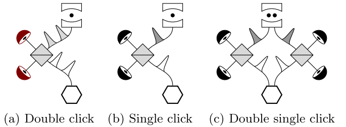
FIG. 1. Diagram illustrating the three remote state preparation protocols. The ion trap represents the server, with a dot denoting an emitting qubit, while the hexagon represents the client equipped with a weak coherent pulse source. Both client and server send their quantum states to the Bell state measurement station. In the double-click protocol in panel (a), a two-mode encoding is used, such as polarization or time bin, while in the single-click [panel (b)] and double-single-click [panel (c)] protocols, presence-absence encoding is applied in a single-mode configuration. The protocols in panels (a) and (c) both require two photons to be detected, but the protocol in panel (c) allows for retrying of each node separately, as the photons are entangled with separate memory qubits. The color of the detectors in panel (a) illustrates that the detectors can decode the encoding of the photons. The two paths and BSM stations are drawn in panel (c) to illustrate the pulses coming from two different memory qubits. It is not required to have two separate BSM stations. The server's qubit is entangled with the emitted light, which, along with the client's light, is mixed on a beam-splitter and analysed by the BSM. Upon successful detection, the server's qubit is projected into a state selected by the client.
