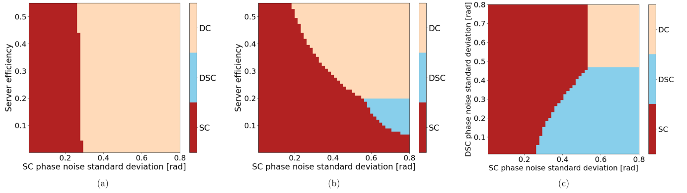
FIG. 4. Optimal RSP protocol—DC, DSC, or SC—as a function of phase noise ( \sigma_{SC} , \sigma_{DSC} , in radians) and server efficiency \eta_s (which includes detector efficiency). For each parameter combination, we find the smallest |\alpha|^2 at which the stated target is achievable and select the best-performing protocol: DC (peach), DSC (blue), or SC (red). Each panel fixes one parameter and optimizes a different figure of merit, as detailed in the subcaptions. (a) Protocol that gives the highest dimensionless rate R\tau given a target fidelity of 0.98 for \sigma_{DSC} = 0.5 rad. (b) Protocol that gives the highest fidelity given a target of R\tau = 0.01 for rad. (c) Protocol that gives the highest fidelity given a target of R\tau = 0.01 for \eta_s = 0.21 .
