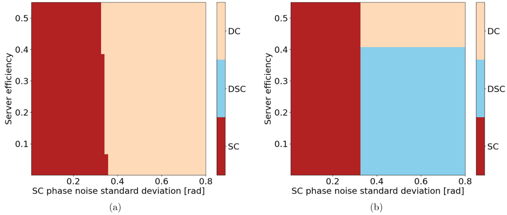
FIG. 6. Optimal RSP protocol—DC, DSC, or SC—giving the highest rate for a given target fidelity, across varying phase noise \sigma_{\text{SC}} and server efficiency. Alternative values for Fig. 4(a). (a) F_{\text{targ}} = 0.97 , \sigma_{\text{DSC}} = 0.5 rad and (b) F_{\text{targ}} = 0.97 , \sigma_{\text{DSC}} = 0.25 rad.
