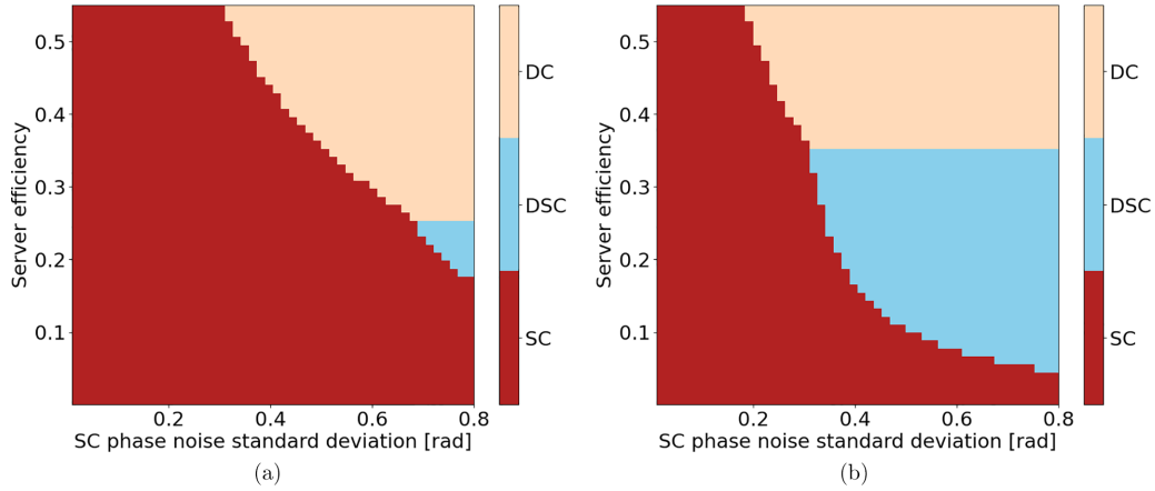
FIG. 7. Optimal RSP protocol—DC, DSC, or SC—giving the highest fidelity for a given target rate, across varying phase noise \sigma_{SC} and server efficiency. Alternative values for Fig. 4(b). (a) Target R\tau = 0.03 , \sigma_{DSC} = 0.5 rad and (b) Target R\tau = 0.01 , \sigma_{DSC} = 0.25 rad.
