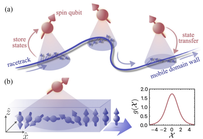
FIG. 1. (a) Schematic diagram illustrating topological quantum signal transmission in a hybrid system, where spin qubits interact with a magnetic nanowire hosting mobile DW textures. (b) A spin qubit interacts with a DW in the magnetic racetrack. The coupling g(\mathcal{X}) varies as a function of the distance \mathcal{X} between the qubit and the DW.
