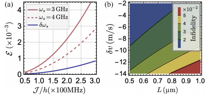
FIG. 3. (a) Two-qubit gate infidelity analysis. The (dashed) red curves illustrate the error caused by spin axis tilting for different spin qubit frequencies \omega_s . The purple curve depicts the error induced by qubit frequency shifts. (b) Infidelity due to DW decoherence as a function of the velocity variation and qubit separation.
