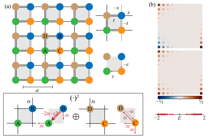
FIG. 2. (a) Implementation based on a \pi -flux quadrupole insulator with reciprocal couplings s \equiv 1 and t as well as additional nonreciprocal couplings of strength \varepsilon . The squared parent system (box) decomposes into the AB and CD subsystems, where the sum rule enforces unidirectional couplings between A and B. (b) The two corner states for the system in panel (a) with 10 \times 10 unit cells and in \varepsilon = -t = 1/2 . Each state belongs to two degenerate eigenvalues forming an exceptional point, and this also applies to all other states of this exceptionally deficient system. The bottom part shows the energy spectrum of the system, with the zero-energy corner states marked in green.
