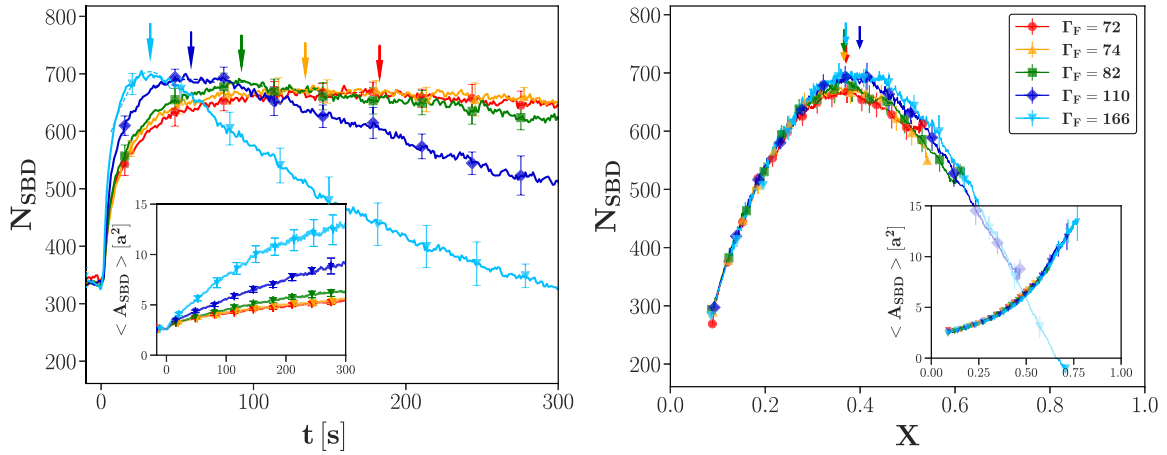
FIG. 4. The left image shows the number of symmetry-broken domains and the average size of the domains (inset) as a function of time for different quench depths. The error bars are averages of about ten independent quenches with about 9000 particles in the field of view. Whereas the average size of the symmetry-broken domains grows monotonically as expected, the number of symmetry-broken domains first increases to a maximum but then decreases in favor of fewer but larger domains. The arrows are a guide to the eye to identify the maxima extracted by fitting a Gaussian distribution around the numeric maxima of the experimental data. The right image shows the same data but plotted as the fraction of symmetry-broken area, which is implicitly a function of time. The curves almost superimpose as a function of crystallinity and are independent of the quench depth. The arrows are pointing to the maximum of each curve, which is about X \sim 37\% .
