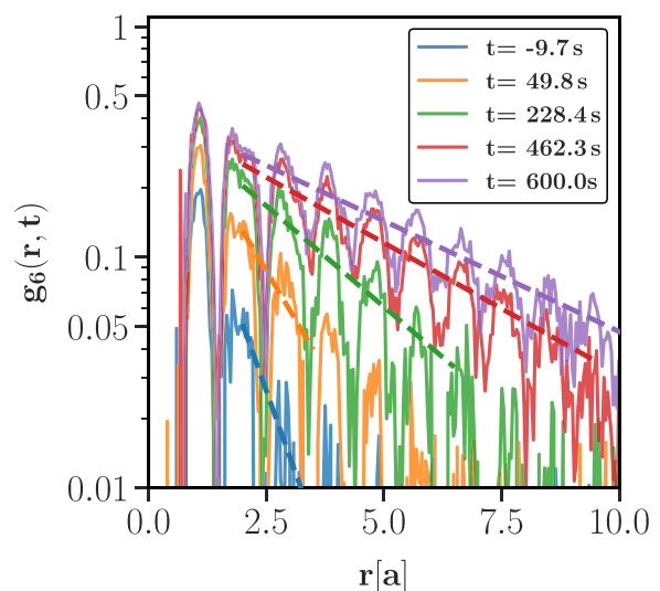
FIG. 1. Bond order correlation function before the quench (blue) at an initial \Gamma_{\text{in}} = 16 and after to a final coupling strength of \Gamma_F = 74 for various waiting times. Dotted lines are exponential fits to the curves, which appear as straight lines in the lin-log plot.
