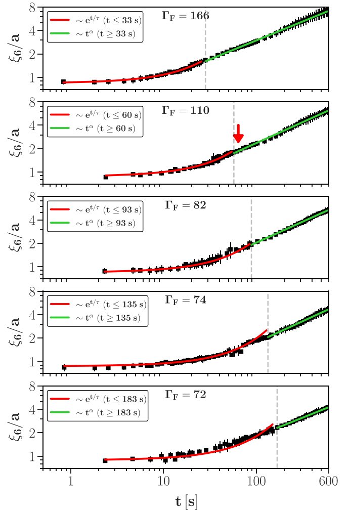
FIG. 2. \xi_6 is presented in a log-log plot for different quench depths. Shortly after the quench, the growing behavior is exponential and switches to algebraic later. The quench depth increases from bottom to top and the crossover time decreases for deeper quenches. The crossover from exponential to algebraic takes place when about 37% particles belong to symmetry-broken domains (see discussion below). The vertical dashed lines are the times, where the number of domains have their maximum, indicated with arrows in Fig. 4. For the quench \Gamma_F = 110 , the red arrow shows the time that the system is in the state shown in Fig. 3.
