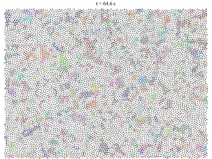
FIG. 3. The symmetry-broken domains are presented 64 s after a quench from \Gamma_{\text{In}} = 16 to a final coupling strength of \Gamma_F = 110 . Small dots are fluidlike particles, whereas big ones are crystal-like. Different colors indicate individual grains, which are labeled in time.
