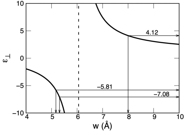
FIG. 3. Dielectric constant across a water thin film as a function of the defined width w of the film for a given value of the 2D polarizability \alpha_{\perp} = 6.06 \text{ \AA} , as obtained with DFT simulations described in the text. Values of \epsilon_{\perp} are highlighted for three values of w for the same film: (i) the distance between the origins of the confining potentials w = 8 \text{ \AA} , (ii) w = 5.17 \text{ \AA} , the accessible perpendicular space as defined by Kumar et al. [21], for this bilayer film, and (iii) w = 5.31 \text{ \AA} , obtained from normalising the 2D density of the film with the 3D density of bulk water. Negative values for \epsilon_{\perp} indicate overscreening, a larger polarization than what is needed to screen the field completely.
