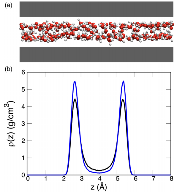
FIG. 1. (a) Schematic view of the simulation box, perpendicular to the confining plane. The gray-shaded regions represent the location of the confining soft potentials. Oxygen and hydrogen atoms in the water molecules are represented as red and white spheres, respectively. (b) Oxygen density profiles along the confining direction for 2D densities \sigma = 0.177 \text{ \AA}^{-2} (black) and 0.195 \text{ \AA}^{-2} (blue).
