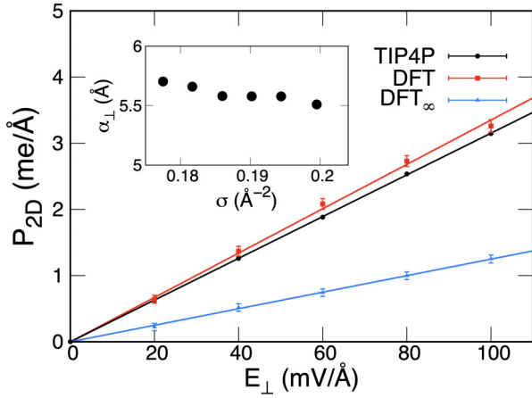
FIG. 2. 2D polarization \mathcal{P}_{2D} vs external traverse electric field \mathcal{E}_{\perp}^{\text{ext}} for TIP4P/2005 water classical trajectories (black) and for DFT calculations using the classical TIP4P/2005 under the same external field (red). In blue, we show the pure electronic response obtained from DFT as explained in the text. Inset: 2D density dependence of \alpha_{\perp} obtained with the TIP4P/2005 classical simulations.
