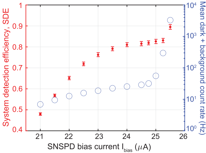
FIG. 9. Characterization of SNSPD: SDE and DBCR vs detector bias current. The error bars depicted correspond to one Poissonian distribution standard deviation in the measured count rates and an additional 0.1 dB error in the measured calibration optical power.
