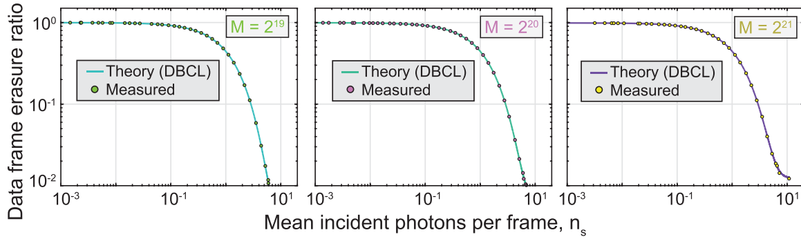
FIG. 11. Comparison of theoretical dark-background-count-limited (DBCL) and experimentally measured PPM frame erasure ratio, for PPM 2^{19} , 2^{20} , and 2^{21} with T_{\text{slot}} \approx 400 ps. The theoretical curves are plotted for a detection efficiency \eta_s = 0.815 and a dark/background count rate (DBCR) of 15 Hz.
