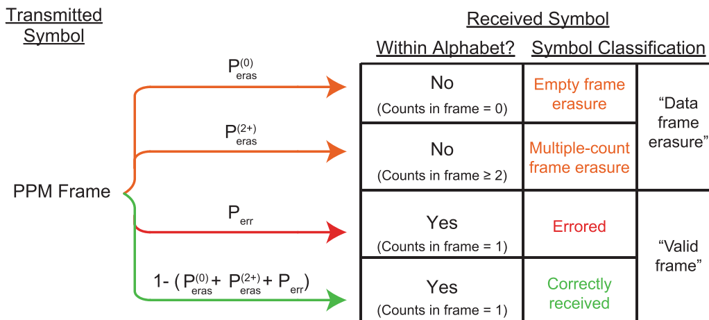
FIG. 8. Schematic depicting a PPM erasure channel diagram. Each detected PPM frame is categorized into one of four outcomes based on the number of counts measured in the frame.
