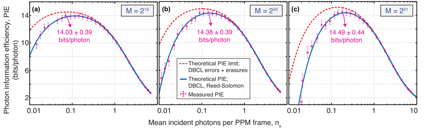
FIG. 4. Measured and theoretical dark-background-count-limited PIE vs mean incident photon number per PPM frame, n_s , for (a) M = 2^{19} , (b) M = 2^{20} , and (c) M = 2^{21} . Dashed red curve: maximum achievable mutual information rate per incident photon for theoretical DBCL frame error and erasure probabilities. Solid blue curve: PIE achievable for such a channel upon employing RS coding. Both theoretical curves assume a transmitter source that produces infinite extinction ratio optical pulses. Magenta data points: measured PIE and its uncertainty estimates. All curves shown are computed for experimentally determined SDE and DBCR ( \eta_s = 0.815 , DBCR = 15 Hz), allowing direct comparison of theoretical and measured PIEs.
