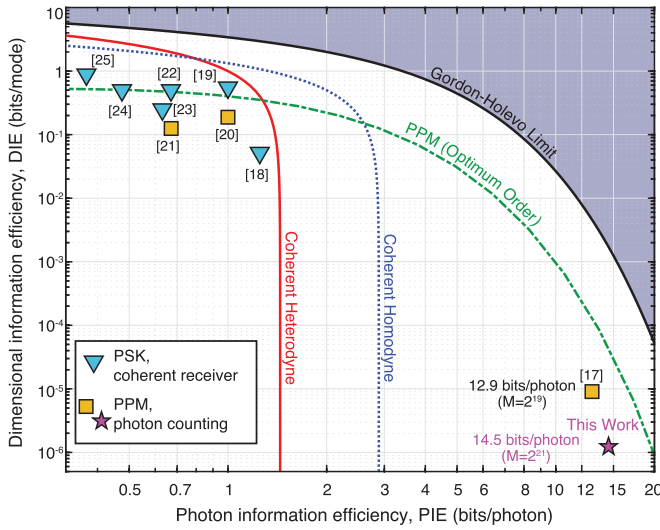
FIG. 2. Comparison of experimentally demonstrated PIEs and their associated DIEs, alongside theoretical capacities for photon counters (Gordon-Holevo), coherent homodyne and heterodyne, as well as for PPM with optimum modulation order and photon counters. The symbols display key experimental demonstrations cited in the references section of this paper. The highest PIE enables communication with the faintest received signal ( M : order of PPM; PSK: Phase-Shift Keying).
