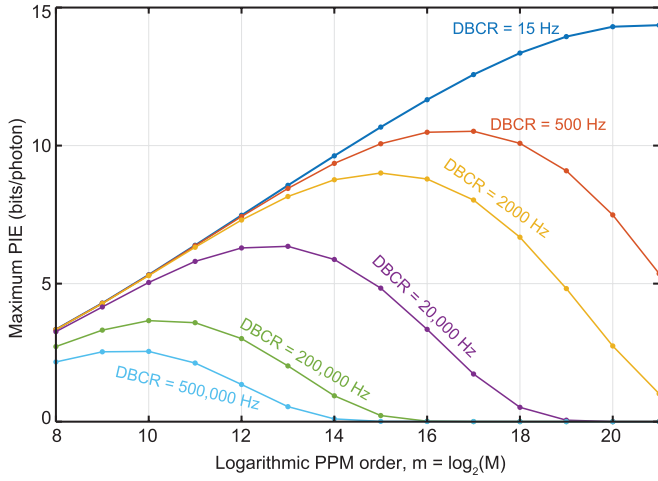
FIG. 15. Maximum attainable PIE vs logarithmic PPM order m = \log_2(M) , computed from theoretical frame erasure and error probabilities, over a range of DBCR values.
