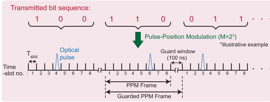
FIG. 6. Illustrative schematic depicting the pulse-position modulation (PPM) scheme employed in this work, for an example case of M = 2^3 . A computer-generated bit sequence is segmented into bit strings of length m = \log_2(M) , and each unique bit string is mapped to a unique temporal position of an optical pulse in one out of M time slots. Consecutive PPM frames are separated by a guard window of 100 ns.
