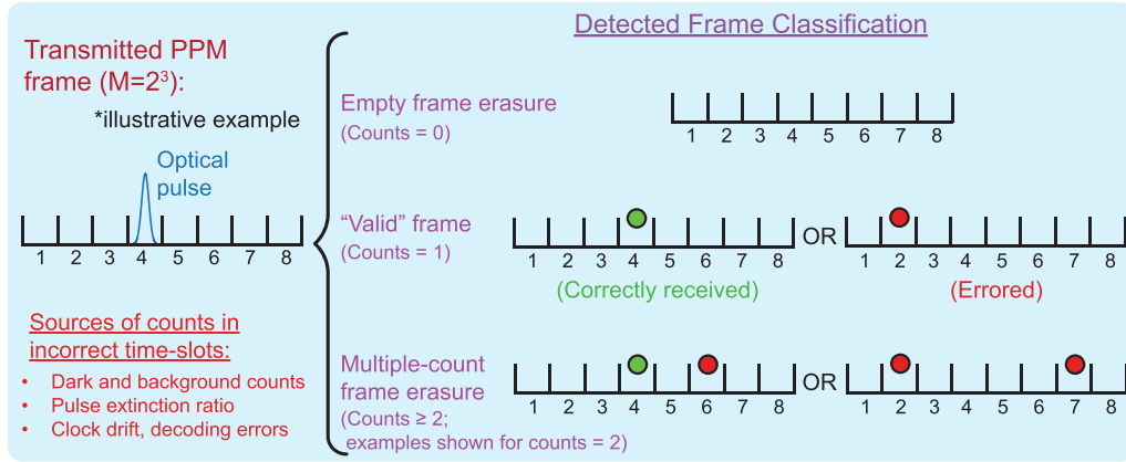
FIG. 7. Schematic illustrating possible detection events for an example case of M = 2^3 . Detected frames that contain zero counts are declared as empty frame erasures, while frames with two or more counts are declared multiple-count frame erasures. If a detected frame contains exactly one count, it is considered a "valid" frame, and is compared with the corresponding transmitted frame to assess frame errors.
