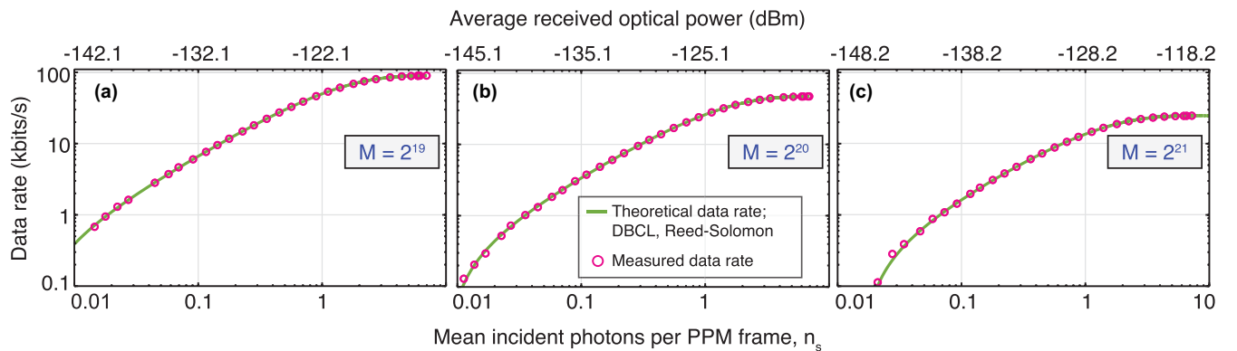
FIG. 5. Measured and theoretical data rate vs mean incident photon number per PPM frame, n_s , and average incident optical power (top axes), for (a) M = 2^{19} , (b) M = 2^{20} , and (c) M = 2^{21} . Solid green curve: theoretically computed data rate achievable for a PPM channel with DBCL error and erasure probabilities upon employing RS coding. Magenta circles: measured data rate. All curves shown are computed for experimentally determined SDE and DBCR ( \eta_s = 0.815 , DBCR = 15 Hz), allowing direct comparison of theoretical and measured data rates.
