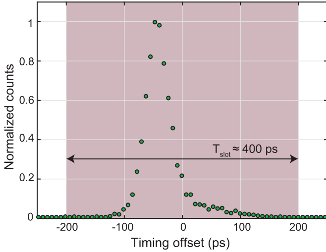
FIG. 10. Shape of the transmitted optical pulse reconstructed by overlaying arrival timestamps of photons detected in known time slots over a long acquisition time. The shaded portion represents T_{\text{slot}} \approx 400 ps, the duration of one PPM time slot. The optical pulse, generated by directly modulating a DFB laser, consists of weak tails that are confined well within this time slot, thereby providing a sufficient extinction ratio to achieve near dark-background-count-limited detection.
