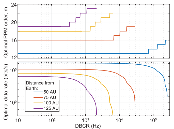
FIG. 16. Performance of adaptive PPM modulation at a fixed receiver power. Top: PPM order M that provides optimal (i.e., maximum) downlink data rate vs DBCR. Bottom: Corresponding optimal data rate. Both plots are shown for four representative transmitter-receiver distances (i.e., received powers).
