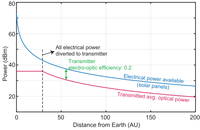
FIG. 13. Variation of electrical power generated by solar panels, and the resulting variation of output average optical power, with distance from Earth. A.U.: astronomical units.
