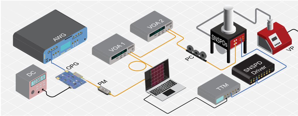
FIG. 3. Experimental schematic of a communication test bed employing a high extinction-ratio optical pulse generator (OPG) source to generate a WCS, using SNSPDs for detection. DC: direct current (power supply); PM: (inline) power meter; VP: vacuum pump.
