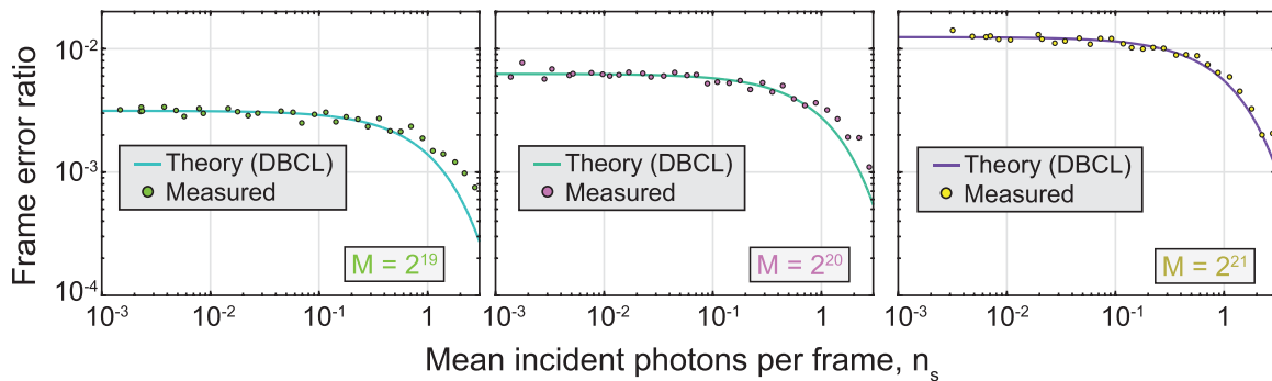
FIG. 12. Comparison of theoretical dark-background-count-limited (DBCL) and experimentally measured PPM frame error ratio, for PPM 2^{19} , 2^{20} , and 2^{21} with T_{\text{slot}} \approx 400 ps. The theoretical curves are plotted for a detection efficiency \eta_s = 0.815 and a dark count rate (DBCR) of 15 Hz. The slight deviation of experimental observation from DBCL performance for n_s \gtrsim 1 can be attributed to the lack of sufficient frame error statistics at such high n_s , with possible minor contributions from the finite extinction of the pulse tails outside of the transmitted time slot.
