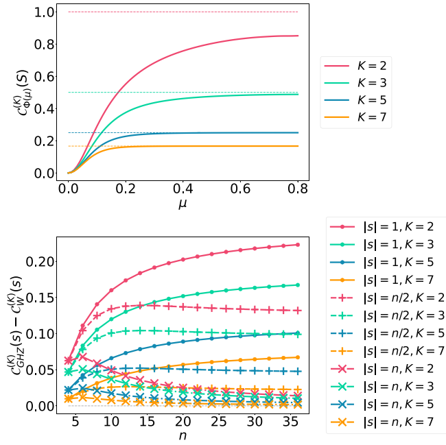
FIG. 3. GCE ( s = S ) of the 40-qubit spin-squeezed state |\Phi(\mu)\rangle for different K and interaction strength \mu (upper plot), and the GCE difference C_{GH}^{(K)}(s) - C_W^{(K)}(s) for different n , |s| and K (lower plot). For |\Phi(\mu)\rangle , GCE measures more entanglement and goes asymptotically to \sim(K-1)^{-1} for larger K and \mu . For GHZ and W , GCE concludes more entanglement in GHZ state than in W state as C_{GH}^{(K)}(s) > C_W^{(K)}(s) , and the GCE difference decreases for increasing K and |s| .
