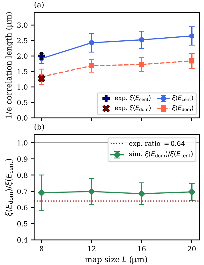
FIG. 11. Finite-size behavior of the correlation-length hierarchy. (a) 1/e correlation lengths \xi(E_{\text{cent}}) and \xi(E_{\text{dom}}) vs map size L (mean \pm std over 30 disorder realizations; fixed 0.4 \mu\text{m} pitch and 0.85 \mu\text{m} optical FWHM); filled markers are the experimental values at L = 8 \mu\text{m} . (b) The hierarchy ratio \xi(E_{\text{dom}})/\xi(E_{\text{cent}}) is finite-size-robust ( \approx 0.69 – 0.70 ) and close to the experimental value 0.64 (dotted line), even though the absolute lengths in panel (a) drift with L .
