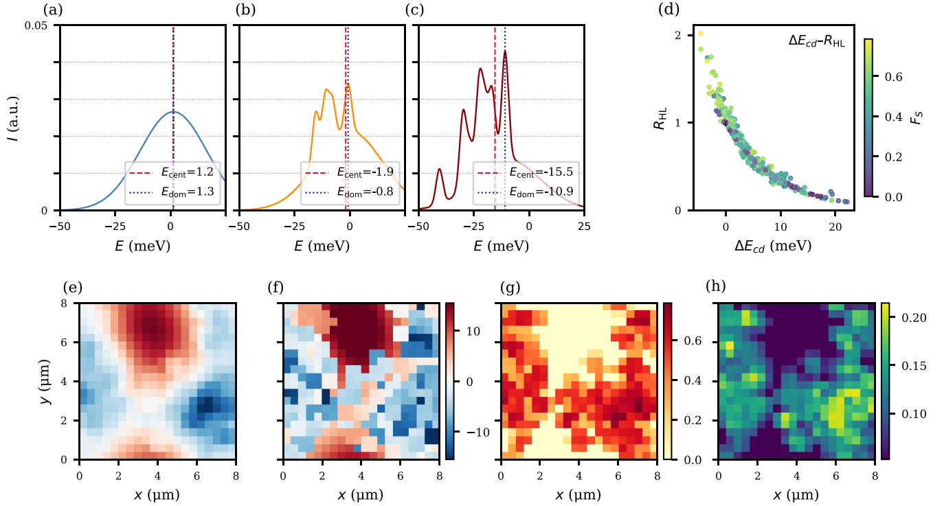
FIG. 6. Simulated local PL spectra and spectral descriptor maps. Upper row: Three representative PL spectra from the 20 \times 20 measurement map, illustrating the three spectral types present in the hierarchical disorder regime. (a) Background-dominated pixel: A single broad Gaussian background peak with E_{\text{cent}} \approx E_{\text{dom}} and no resolved sharp lines ( F_S \approx 0 ). (b) Mixed pixel: The background peak is visible alongside one or two sharp trap peaks; the centroid E_{\text{cent}} is pulled below the dominant peak E_{\text{dom}} by the trap-related weight on the low-energy side of the envelope. (c) Trap-rich pixel: Several sharp lines above the background, with the centroid pulled toward the cluster of trap energies. Vertical dashed and dotted lines mark E_{\text{cent}} (red) and E_{\text{dom}} (blue) for each pixel. (d) Scatter plot of \Delta E_{\text{cd}} vs R_{\text{HL}} for all 400 pixels, colored by F_S . The tight anticorrelation ( \rho_S = -0.955 for this single representative seed; cf. the five-seed mean \rho_S = -0.976 \pm 0.009 in Table II) reflects the robust spectral shape relation derived in Proposition 4; pixels with larger F_S (yellow) show the strongest separation between centroid and dominant-peak energy. Lower row: Spatial maps of four spectral descriptors across the 20 \times 20 measurement grid. (e) \delta E_{\text{cent}} = E_{\text{cent}} - \langle E_{\text{cent}} \rangle : Smooth micron-scale fluctuations tracking V_{\text{slow}} , with \xi(E_{\text{cent}}) \approx 1.93 \mu\text{m} . (f) \delta E_{\text{dom}} = E_{\text{dom}} - \langle E_{\text{dom}} \rangle : More fragmented pattern with additional trap-switching fluctuations, confirming \xi(E_{\text{dom}}) < \xi(E_{\text{cent}}) . Panels (e) and (f) share a common color scale (in meV), so the larger fluctuation amplitude of \delta E_{\text{dom}} is apparent. (g) F_S map: Trap-density-modulated sharp-fraction distribution. (h) R_1 (spectral roughness) map: Closely tracks F_S , consistent with \rho_S(F_S, R_1) = 0.909 .
