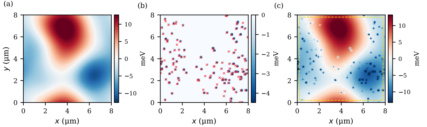
FIG. 2. Hierarchical disorder landscape. (a) Slow correlated disorder V_{\text{slow}}(\mathbf{r}) with amplitude W_s = 6 meV and correlation length \xi_s = 2 \mu\text{m} , generated by FFT-based Gaussian filtering. The smooth red/blue domains of size \sim \xi_s represent the slow-disorder component that gives rise to micron-scale spectral families in the model. (b) Trap disorder V_{\text{trap}}(\mathbf{r}) consisting of N_t = 133 Gaussian potential wells ( W_t = 12 meV, \sigma_t = 50 nm, n_t = 2 \mu\text{m}^{-2} , consistent with n_t L^2 \approx 128 over the 8 \times 8 \mu\text{m}^2 domain). The color scale is saturated at the second percentile of V_{\text{trap}} for visibility; because the field is near zero between the sparse wells, this displayed lower bound is much shallower than the deepest individual well centers, whose bare trap-depth distribution is parametrized by W_t = 12 meV. Red crosses mark the trap centers, which are drawn from P(\mathbf{r}) \propto \exp(-V_{\text{slow}}(\mathbf{r})/E_{\text{bias}}) , with E_{\text{bias}} = 7 meV, biasing the trap positions, or optically active trap sites, toward slow-potential minima. (c) Effective potential V_{\text{eff}} = V_{\text{slow}} + V_{\text{trap}} , showing the combined landscape experienced by excitons. The gold dashed rectangle indicates the 20 \times 20 measurement grid area (spanning 7.6 \times 7.6 \mu\text{m}^2 , i.e., a 0.4 \mu\text{m} pitch matching the experimental 400 nm step, with a 0.2 \mu\text{m} margin from each edge).
