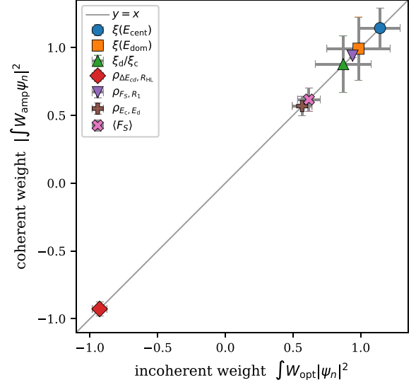
FIG. 10. Descriptor statistics are insensitive to the optical-weight model. For each descriptor statistic (labeled), the value obtained with the coherent radiative weight \int W_{amp} \psi_n|^2 (vertical axis) is plotted against that from the incoherent local-density weight \int W_{opt} |\psi_n|^2 (horizontal axis); error bars are the seed-to-seed standard deviation over five disorder realizations. All points lie close to the y = x line, showing that the two weightings yield statistically indistinguishable descriptor covariance and correlation-length hierarchy within the seed-to-seed uncertainty.
