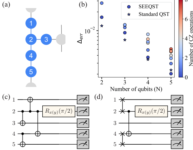
FIG. 3. Experimental implementation. (a) Layout of the five qubits used on the ibm_marrakesh quantum processor. (b) Average reconstruction error \Delta_{\text{err}} for the state |+y\rangle^{\otimes N} , as a function of the number of qubits N and the number of CZ operations in the SEEQST circuits. (c) The two circuits for the selective block S_{32} in a five-qubit state, where all qubits are off-diagonal. (d) The two quantum circuits for the selective block S_{18} in a five-qubit state, where q_1 and q_5 are off-diagonal. Since they are not directly connected, two additional SWAP operations are required to effectively implement \text{CNOT}_{15} as required by SEEQST.
