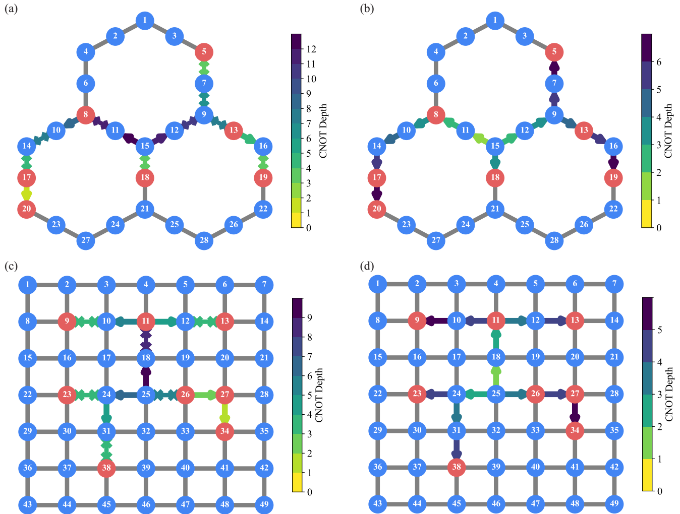
FIG. 6. Circuit depth for SEEQST for different qubit layouts. Red nodes represent off-diagonal qubits. Arrows represent CNOT gates (control \rightarrow target), and SWAP gates are denoted by \times - \times . (a) Implementation on a heavy-hexagon lattice, inspired by panel (b), which depicts the GHZ-state-generation circuit layout with all red qubits enclosed within boundary B . (c) Implementation on a square lattice, inspired by the GHZ-state-generation layout shown in panel (d).
