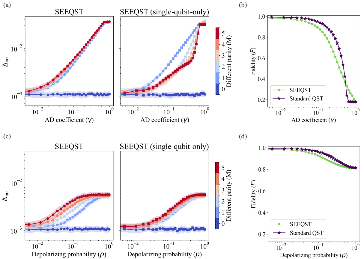
FIG. 8. Numerical simulation of SEEQST performance under noise. The effect of (a) amplitude damping and (c) depolarizing noise on the estimation error \Delta_{\text{err}} for different SEEQST subsets, categorized by the different parity M . Left panels show results for the standard SEEQST protocol, while right panels show the performance for its single-qubit gates only variant. (b), (d) Impact of amplitude damping and depolarizing noise on the state fidelity F , comparing SEEQST with standard QST. All simulations are for full-rank five-qubit states and 16384 shots per measurement setting. Solid lines represent the mean over multiple simulation runs, and the shaded regions show the standard deviation.
