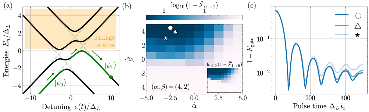
FIG. 4. On-the-go operations using coherent shuttling-induced excitations. The energy spectrum of the Hamiltonian (10), where we marked in orange the undesired leakage states, is plotted in panel (a). In addition, we plot the minimum infidelities 1 - \tilde{F} for the state transfers |\psi_0\rangle \rightarrow |\psi_1\rangle [panel (b)] and |\psi_1\rangle \rightarrow |\psi_0\rangle (inset), for possible pulse times \Delta_L t_f \in [0, 500] . Using the Horodecki identity, in panel (c), we analyze the effective X-gate average gate fidelity F_{\text{gate}} = (1 + \sum_{j=0,1} |\langle \psi_j(0) | \psi_{1-j}(t_f) \rangle|^2) / 3 for the computational subspace spanned by the lower two eigenstates as a function of possible pulse times \Delta_L t_f for the indicated circle, square, and star parameters in panel (b). The parameters used are t_c / \Delta_L = 0.1 , \Delta_R / \Delta_L = 5 , \phi_L = 0.1 , \phi_R = \pi/2 . The detuning is swept from \varepsilon / \Delta_L \in [-10, 10] .
