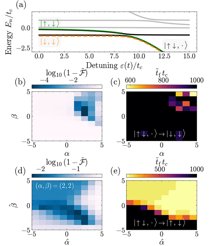
FIG. 3. Initialization of a spin qubit in a DQD. The energy spectrum is shown in panel (a). The optimal infidelity and corresponding pulse times for the adiabatic protocol ( |\uparrow\downarrow, \cdot\rangle \mapsto |\downarrow, \downarrow\rangle ) are illustrated in panels (b) and (c). Similarly, for the di-ad protocol ( |\uparrow\downarrow, \cdot\rangle \mapsto |\uparrow, \downarrow\rangle ), we showcase the infidelities and pulse times in panels (d) and (e). The DQD parameters read \tilde{U}/t_c = 10 , E_Z/t_c = 0.9 , \Delta E_Z/t_c = 0.1 , \Delta E_X/t_c = 0.01 , where we sweep the detuning \varepsilon(0)/t_c = 15 to \varepsilon(t_f)/t_c = 0 . For the di-ad protocol, we fix the adiabatic parameters to (\alpha, \beta) = (2, 2) . For the protocol, we sweep possible pulse times t_f t_c \in [0, 1000] .
