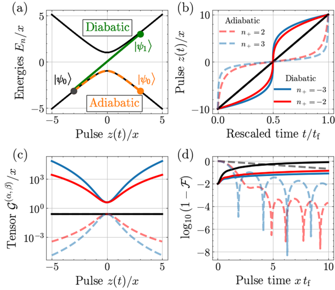
FIG. 2. Coherent state transfer for the adiabatic ( |\psi_0\rangle \mapsto |\psi_0\rangle , dashed lines) and the diabatic ( |\psi_0\rangle \mapsto |\psi_1\rangle , solid lines) evolution in the Landau-Zener model. We show the energy spectrum [panel (a)], the di-ad pulse [panel (b)], originating from the corresponding di-ad metric [panel (c)], and the resulting infidelities 1-\mathcal{F} [panel (d)] with \mathcal{F} = |\langle\psi_0(t_f)|U(t_f)\psi_0(0)\rangle|^2 for adiabatic and \mathcal{F} = |\langle\psi_1(t_f)|U(t_f)\psi_0(0)\rangle|^2 for diabatic evolution, where U(t_f) describes the unitary evolution given the pulse z(t)/x . The Hamiltonian parameters used are z(0)/x = -z(t_f)/x = -10 . The colored pulses refer to different n_+ with the appropriate sign for adiabatic (dashed) and diabatic (solid) protocols: |n_+| = 0, 2, 3 corresponds to black, red, and blue, respectively.
