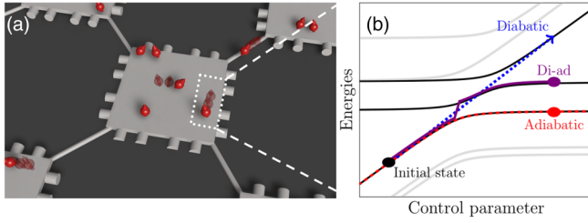
FIG. 1. Application of the di-ad protocol [panel (a)], here, spin qubit shuttling, and the emergent dense energy spectrum as a function of some control parameter [panel (b)]. The di-ad protocols allow for flexible and high-fidelity state transfer beyond the extrema of adiabatic (red, dashed) and diabatic (blue, dashed) limits by selectively operating between both regimes (purple).
