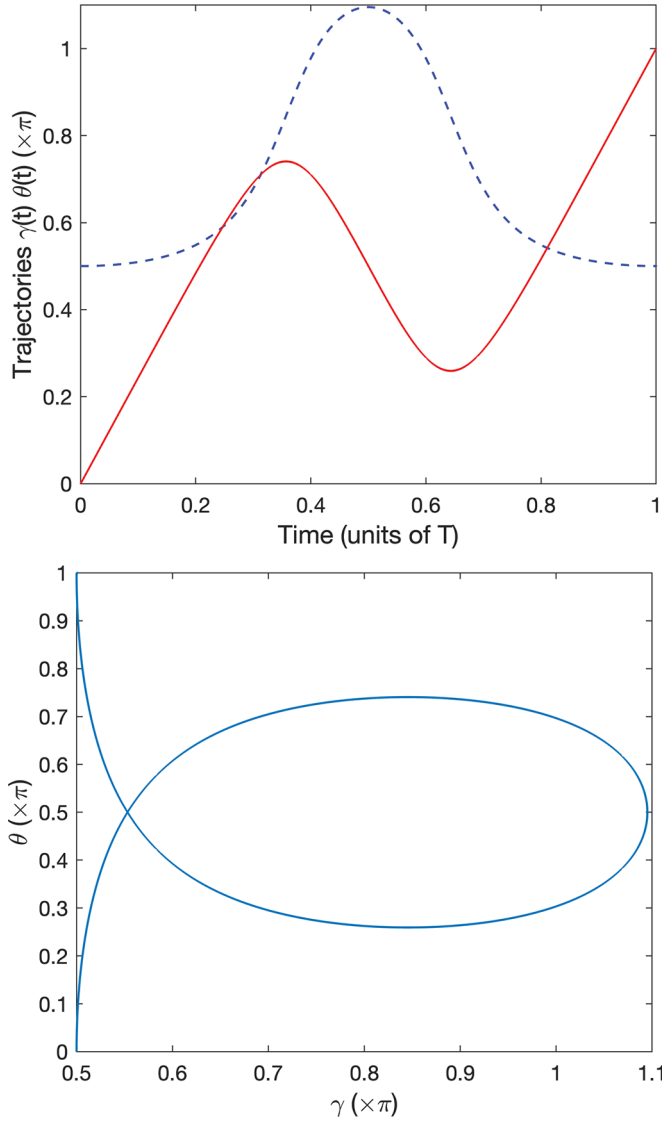
FIG. 7. Upper frame: Optimal trajectories \theta(t) (full line), \gamma(t) (dashed line) for fifth-order 0\pi -NOP with pulse area \mathcal{A} \approx 2.435\pi . Lower frame: corresponding optimal trajectory \tilde{\theta}(\gamma) .
