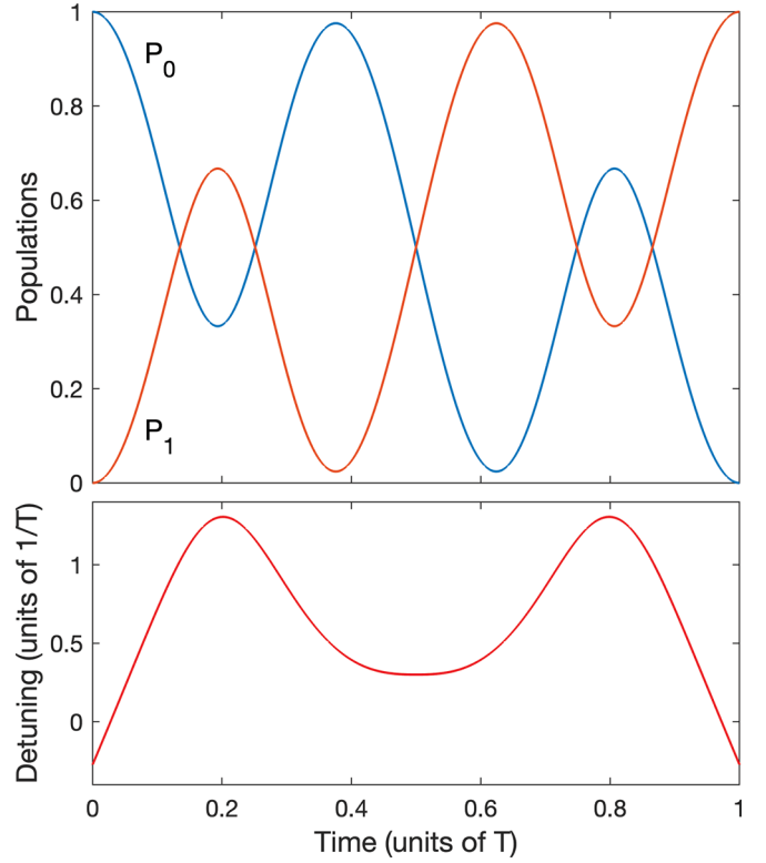
FIG. 12. Same as Fig. 8 but for the optimal trajectory of Fig. 11.
