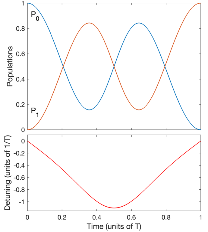
FIG. 8. Population dynamics P_j = |\langle j | \phi_0(t) \rangle|^2 , j = 0, 1 (upper frame), associated with the detuning (lower frame) with the square pulse of amplitude \Omega_0 \approx 2.435\pi/T resulting from the optimal trajectories \theta(t) and \gamma(t) of Fig. 7.
