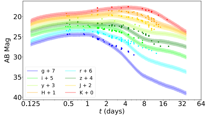
FIG. 5. Light curves predicted by our kilonova surrogate model for the Nedora21 GW + EM ejecta posteriors presented in Fig. 4, with solid lines corresponding to the median posterior values and shaded bands representing 1\sigma uncertainty. This posterior includes the effect of marginalizing over unknown model systematic uncertainty \sigma_{\text{sys}} , as described in the text.
