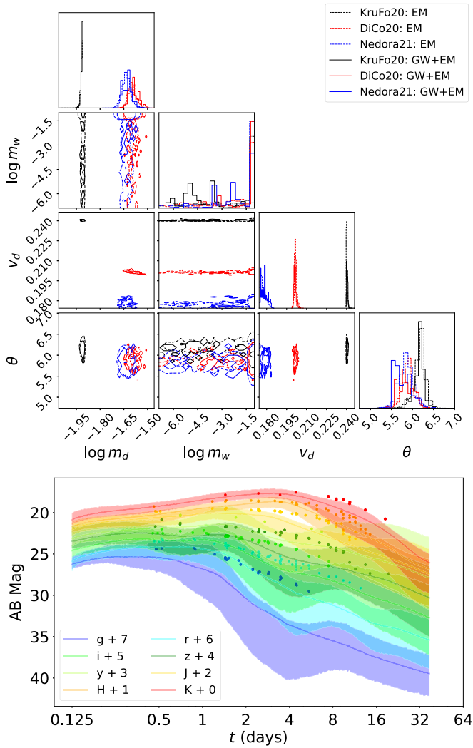
FIG. 7. Top: Ejecta posterior distributions using EM (dashed) and GW + EM (solid) likelihoods with an assumed disk mass ejection of f_{\text{disk}} = 30\% . In contrast to Fig. 4, m_w is less constrained (leading to the large uncertainties in the light curves below) and v_d is specific to the ejecta fit model. Bottom: Light curves associated with the Nedora21 GW + EM ejecta posteriors presented above, with solid lines corresponding to the median posterior values and shaded bands representing 1\sigma uncertainty. It is obvious that, at least for the purposes of parameter inference, assuming the same fixed disk fraction for all three ejecta fits yields poor fits to the data with a relatively high degree of uncertainty.
