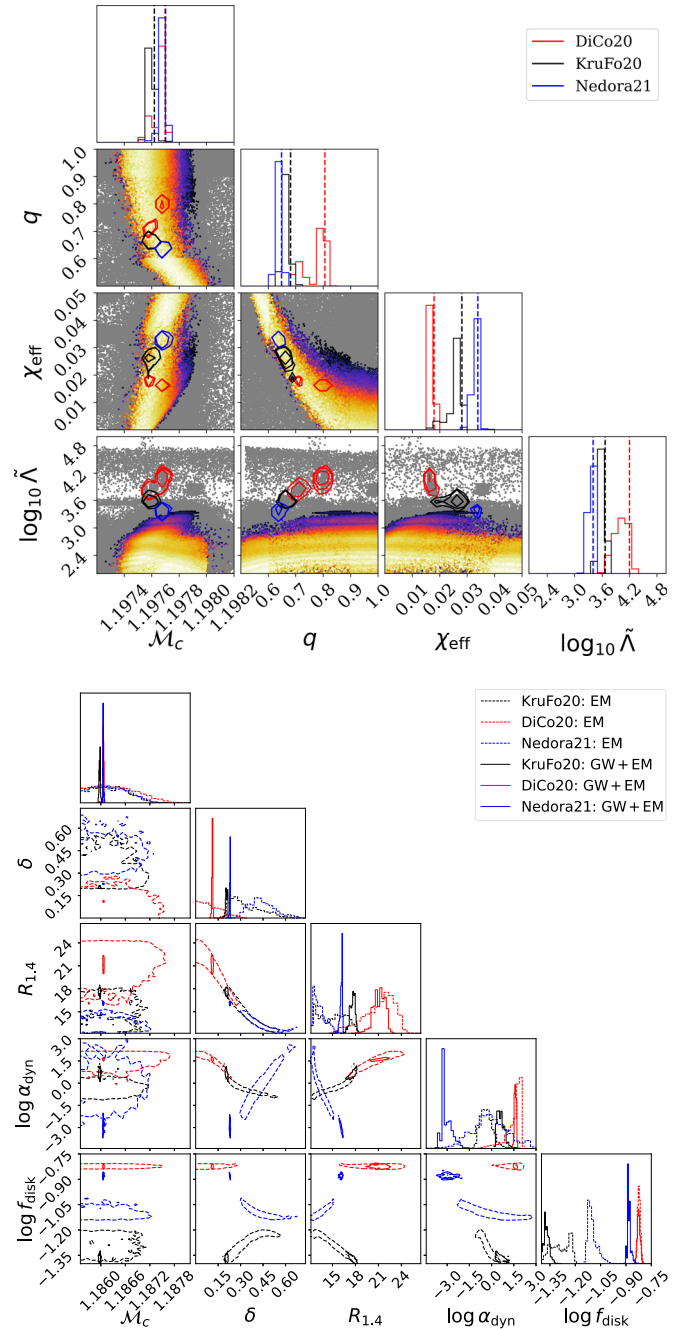
FIG. 6. Same as Figs. 2 and 3, but not allowing for systematic uncertainty in v_d (i.e., \beta_\phi = 0 ). Note the recreation of the v_{\text{ej}} contours from Fig. 1 in the R_{1.4} vs \delta plane.
