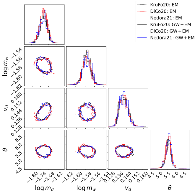
FIG. 4. Ejecta posterior distributions using EM (dashed) and GW + EM (solid) likelihoods with the disk mass ejection fraction left as a free parameter. The wind velocity is fixed to v_w = 0.10c per the posteriors in Ref. [56]. There is little difference in the ejecta posteriors between the two approaches, modulo artifacts from varying sample counts, due to our kilonova model requiring parameters in a very narrow region to recreate the AT2017gfo light curves. Figure 3 highlights the differences in the binary parameters when including the GW likelihood.
