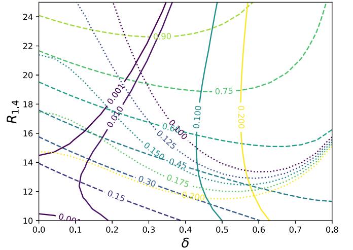
FIG. 1. Solid, dashed, and dotted line contours corresponding to the KruFo20 dynamical ejecta mass m_{\text{ej}} , disk mass m_{\text{disk}} , and ejecta velocity v_{\text{ej}} , respectively. Contours were calculated as a function of mass asymmetry \delta = (m_1 - m_2)/(m_1 + m_2) and neutron star radius R_{1.4} . Mass and velocity units are in M_\odot and c , respectively.
