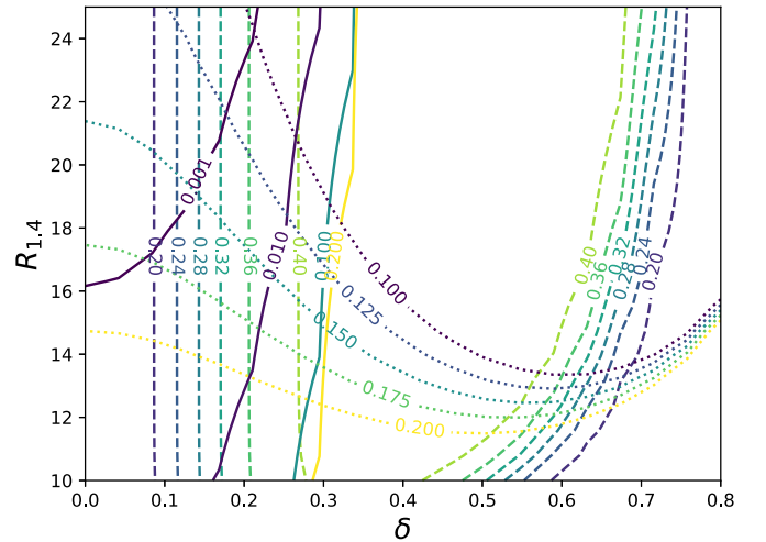
FIG. 8. Ejecta contours as in Fig. 1, but for the DiCo20 forward model. The disk mass (dashed lines) is constrained by \delta but unbounded in the R_{1,4} dimension.
