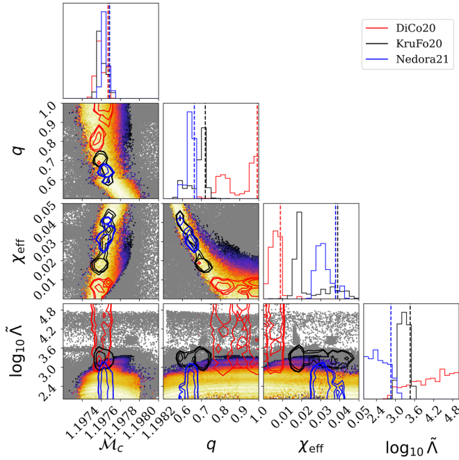
FIG. 2. In this figure, the colored dots represent the input marginal likelihood data assumed in our analysis. In black, red, and blue, we overplot posteriors corresponding to the 90% credible interval for the KruFo20, DiCo20, and Nedora21 GW + EM predictions, respectively. Here, \mathcal{M}_c is in the detector frame.
