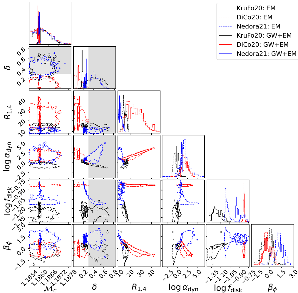
FIG. 3. Binary parameter posterior distributions using EM (dashed) and GW + EM (solid) likelihoods using \log f_{\text{disk}} priors of [-0.9, -0.75] , [-1.4, -1.2] , and [-1.2, -1] for DiCo20, KruFo20, and Nedora21, respectively. The inclusion of the GW likelihood most noticeably affects the chirp mass \mathcal{M}_c and mass asymmetry \delta , while simultaneously providing tighter constraints on the neutron star radius R_{1.4} and ejected disk fraction f_{\text{disk}} . Gray shaded regions represent \delta > 0.3 for which the secondary star's mass is subsolar ( < 1M_\odot ).
